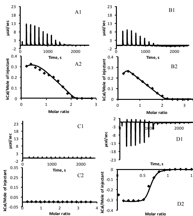
Fig. 1 Isothermal titration calorimetry isotherms obtained by titrating (A1+A2) 0.2 % w/v methylcellulose with 2 % w/v poly (acrylic acid), (B1+B2) 0.2 % methylcellulose with 2 % w/v poly(methacrylic acid), (C1+C2) 0.2 % w/v dextran with 2 % w/v poly (acrylic acid), (D1+D2) 0.2 % w/v polyacrylamide with 2 % w/v poly(acrylic acid) solutions all at pH 2.0. 1 denotes raw graphical data which has been transformed to measure the relationship of concentration labelled 2 whose fitting allows parameter determination. (See Figures S4-6, Supplementary Information for the full set of ITC isotherms for all combinations).
