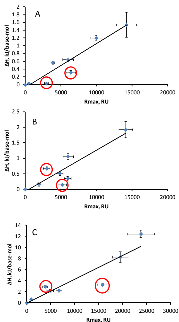
Figure 3. Correlation between enthalpy ( \Delta H ) and Biacore response for IPCs formed by PAA (A), PMAA (B) and TA (C) with each of the non-ionic polymers, outliers (red) were not included in the linear fitting, and were defined as outside 3 standard deviations using Grubbs' test (98 % confidence level).
