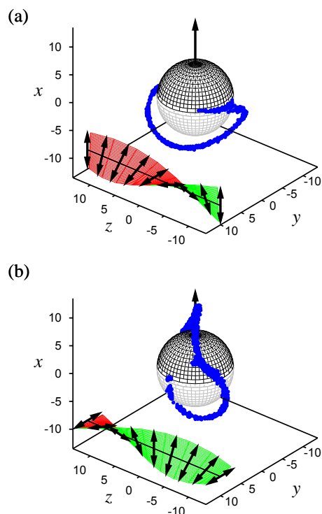
Fig. 10 As Fig. 4, but for a Janus colloid ( r_0 = 6 , d_0/p = 0.24 ) with planar surface anchoring at the upper (black) hemisphere and a homeotropic anchoring at the lower (grey) hemisphere. The arrow through the colloid indicates its orientation \hat{\mathbf{u}}_J . The configurations are related to (a) \vartheta = 90^\circ and (b) \vartheta = 0^\circ .
