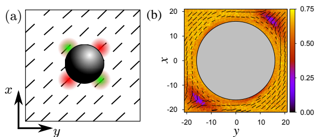
Fig. 6 (a) Sketch of a cross-section of the simulation cell in the x - y plane at z = z' . Colloid and \hat{\mathbf{n}}_0(z) are represented by the gray shaded area and the dashes respectively. Red and green areas refer to respective regions in which locally planar anchored mesogens are orthogonal or collinear to \hat{\mathbf{n}}_0(z) . (b) Corresponding data for \hat{\mathbf{n}}_0(z) (dashes) and the local order parameter at z = 0.2 (see attached color bar).
