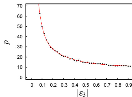
Fig. 2 Pitch p as a function of the magnitude of the chiral coupling constant, |\epsilon_3| . The red line is intended to guide the eye. The transition from the cholesteric to the blue phase occurs at |\epsilon_3| = 0.2 . 25
