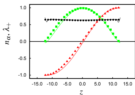
Fig. 3 Plots of components n_x ( \blacktriangle , \text{---} ) and n_y ( \blacksquare , \text{---} ) of the local director field and of the local nematic order parameter \lambda_+ ( \bullet , \text{---} ) as functions of z . Data are obtained for \epsilon_3 = -0.10 and s_z = 27 , where lines refer to the presence and symbols to the absence of the colloid.
