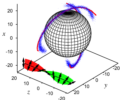
Fig. 5 As Fig. 4, but for a planar anchoring. The fit of Eqn. (22) to the MC data is obtained for r_{\text{eff}} = 22 and \delta r = 0.2r_{\text{eff}} .
