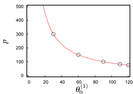
Fig. 7 The red line represents the pitch of a TNC with s_z = 27 as a function of the angle \theta_0^{(1)} at constant \theta_0^{(2)} = 0^\circ (see Eqn. 11) whereas the circles mark the relevant pitches used in Fig. 8 and 9 in a TNC.
