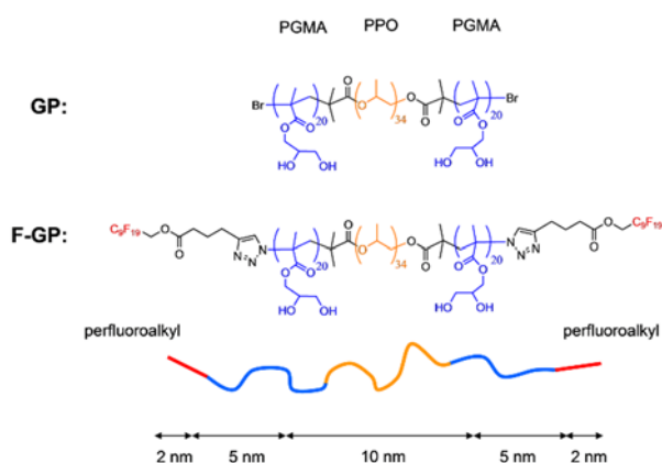
Figure 1: Structures of the studied block copolymers GP and F-GP and schematic representation of a polymer chain with its hydrophobic (yellow), hydrophilic (blue) and fluorophilic (red) building blocks and their approximate contour lengths in fully stretched all-trans conformation.
