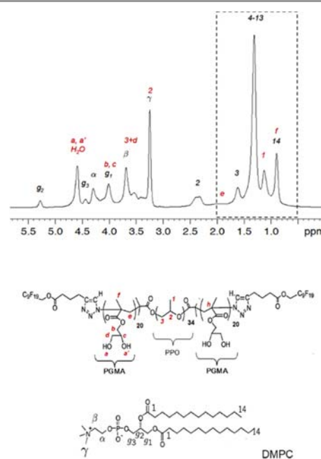
Figure 6: ^1\text{H} NMR spectrum of the mixture of DMPC with FGP (5 mol%) and structures of the molecules including assignment of the ^1\text{H} resonances. Peaks labelled in red originate from the polymer and peaks labelled in black originate from lipid resonances. The region of the spectrum inside the dashed box is evaluated in a 2D-NOESY experiment (see Figure 7).
