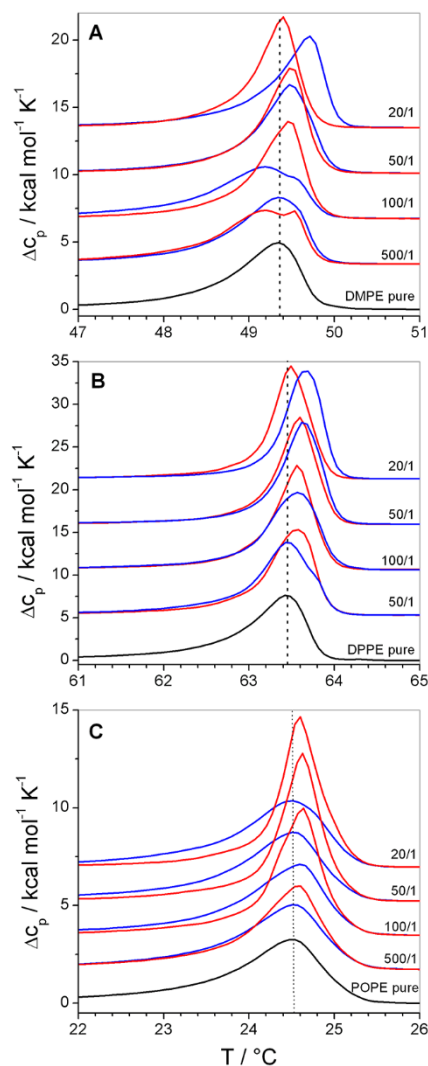
Figure 4: DSC thermograms of polymer bound lipid vesicles prepared from A: DMPE, B: DPPE and C: POPE. Black traces represent the phase transition of the pure lipid vesicles, blue traces their mixtures with GP and red traces their mixtures with F-GP. The lipid/polymer molar mixing ratio is given in the figure. Dotted lines are drawn at T_m of the pure lipid membranes. The lipid concentration is always 1 mmol/L.
