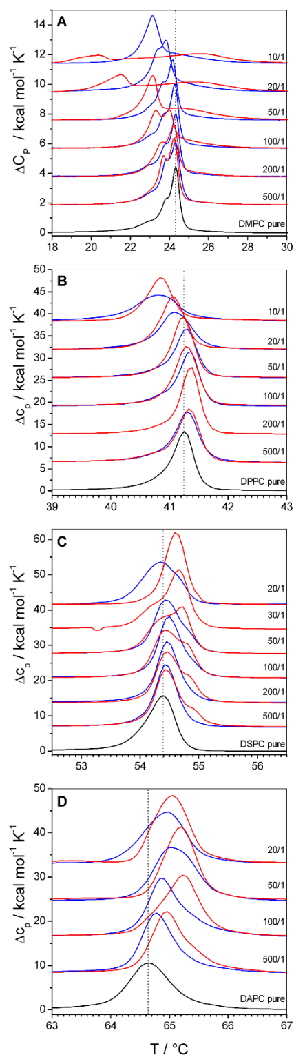
Figure 2: DSC thermograms of polymer bound lipid vesicles prepared from A: DMPC, B: DPPC, C: DSPC and D: DAPC. Black traces represent the phase transition of the pure lipid vesicles, blue traces their mixtures with GP and red traces their mixtures with F-GP. The lipid/polymer molar mixing ratio is given in the figure. Dotted lines are drawn at T_m of the pure lipid membranes.
