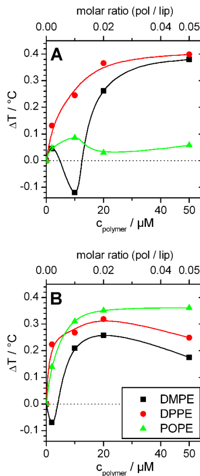
Figure 5: Change of the main transition temperatures of lipid membranes prepared from DMPE (black), DPPE (red) and POPE (green) after addition of different amounts of A: GP and B: F-GP. The lipid concentration is always 1 mmol/L. The temperature where half of the transition enthalpy was consumed was interpreted as transition temperature. The inserted lines are drawn to guide the eyes.
