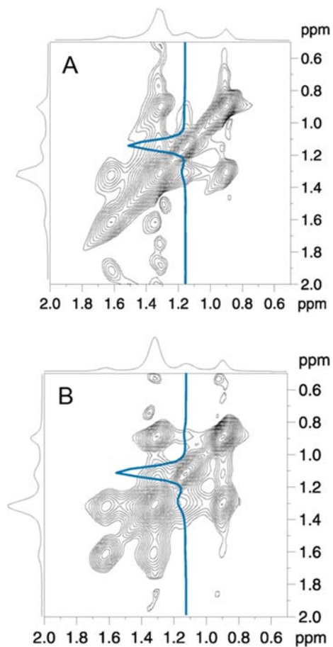
Figure 7: 2D-NOESY - spectra of DMPC mixed with A: unfluorinated and B: fluorinated polymer (both 5 mol%) measured at 40 °C. The base level of the counter plots is set to 5% of the highest intensity. The blue lines represent slices at the position of the PPO-methyl resonance in the \omega_1 - dimension.
