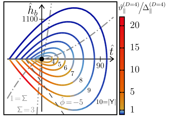
FIG. 1. Behavior of the normalized scaling function \vartheta_{\parallel}^{(D=4)} ( \mathcal{Y} = \text{sgn}(t) L/\xi(t, h_b) , \Sigma = \text{sgn}(th_b) \xi_t/\xi_h ) of the CCF from Landau theory along lines of constant scaling variable |\mathcal{Y}| = 4, 5, \dots, 10 (from the inner to the outermost ring) in the thermodynamic state space of the solvent spanned by \hat{t} = (L/\xi_+^{(0)})^{1/\nu} t and \hat{h}_b = (L/\xi_h^{(0)})^{\beta\delta/\nu} h_b . The color along the lines of constant |\mathcal{Y}| indicates the absolute value |\vartheta_{\parallel}^{(D=4)}| . The bulk critical point of the solvent (\hat{t}, \hat{h}_b) = (0, 0) is indicated by \bullet . The region shown here lies above the capillary transition critical point (\mathcal{Y}_{\parallel,c} = -11, \Sigma_{\parallel,c} = 1.3) [20], where the film coexistence line ends. For (+, +) boundary conditions, the capillary condensation transition occurs for \hat{t} < 0 and \hat{h}_b < 0 . The dash-dotted lines indicate the thermodynamic paths \Sigma = 1 and 3 and the dashed line the path of constant order parameter \hat{\phi} = \frac{t}{\xi_+^{(0)}} \phi/\mathcal{B}_t = -5 . Within Landau theory \nu = 1/2 and \nu/(\beta\delta) = 1/3 . \Delta_{\parallel}^{(D=4)} = |\vartheta_{\parallel}^{(D=4)}(\mathcal{Y} = 0, \Sigma)| , which is independent of \Sigma .
