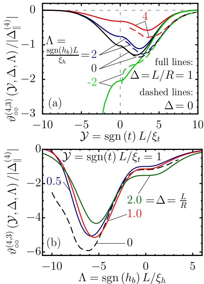
FIG. 4. Effect of the bulk field ( \Lambda \neq 0 ) on the scaling function \vartheta_{\circ\circ}^{(D=4, d=3)} of the critical Casimir force [Eq. (6)] as obtained from Landau theory. (a) Normalized \vartheta_{\circ\circ}^{(4,3)} shown as a function of \mathcal{Y} = \text{sgn}(t) L / \xi_t for \Delta = L/R = 1 (full lines) and within the Derjaguin approximation ( \Delta = 0 , dashed lines) for four values of \Lambda = \text{sgn}(h_b) L / \xi_h . (b) Normalized \vartheta_{\circ\circ}^{(4,3)} shown as a function of \Lambda for \mathcal{Y} = 1 and for four values of \Delta . The curves are normalized with the critical Casimir amplitude \Delta_{\parallel}^{(4)} for the film.
