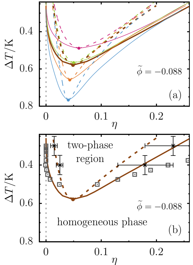
FIG. 6. Segregation phase diagram from theory (RPA), experiment, and simulations (MC). (a) The phase diagram obtained within RPA using the four available background potentials U_{bck} from Fig. 5, and their average. The critical Casimir potential is calculated within the Derjaguin approximation using the local functional approach (see Sec. IV A) for a reduced solvent order parameter \tilde{\phi} = -0.088 . The background contributions U_{bck} have been extracted from the experimentally determined effective potentials [compare Eq. (17)] at \Delta T/K = 0.6 (magenta), 0.5 (green), 0.4 (orange), and 0.3 (blue). The thick dark red curve corresponds to the average of the four potentials U_{bck} . The solid lines show the phase boundaries in terms of the packing fraction \eta of the colloids, the dashed lines correspond to the spinodals, and dots represent critical points. (b) Comparison of the theoretical predictions for the phase boundaries (based on the average U_{bck} ) with Monte Carlo simulations ( \square ) and experiments ( \times , with error bars) of Ref. [10]. On the temperature axis \Delta T = T_c - T increases from top to bottom in order to mimic a lower critical point T_c (of the solvent) as observed experimentally.
