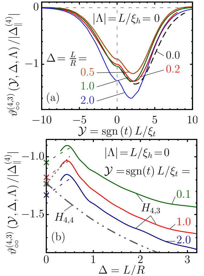
FIG. 3. The critical Casimir force between two like colloids in zero bulk field ( \Lambda = 0 ) as obtained from Landau theory. (a) The normalized scaling function \vartheta_{\infty}^{(D=4,d=3)} versus \mathcal{Y} = \text{sgn}(t)L/\xi_t for five values of \Delta = L/R , where L is the surface-to-surface distance between two H_{4,3} -particles of radius R . The curve \Delta = 0 corresponds to the Derjaguin approximation. (b) The normalized scaling function \vartheta_{\infty}^{(4,3)} versus \Delta for three values of \mathcal{Y} > 0 . The results of the Derjaguin approximation as given by Eq. (7) are shown by dashed lines ( \Delta \rightarrow 0 , next to leading order) and by crosses ( \Delta = 0 ). We recall the relation \vartheta_{\infty}^{(D=4,d=3)}(\mathcal{Y} = 0, \Delta = 0, \Lambda = 0) = \frac{\pi}{3} \tilde{\vartheta}_{\parallel}^{(D=4)}(0, 0) = \frac{\pi}{3} \Delta_{\parallel}^{(4)} . For comparison, the scaling function \vartheta_{\infty}^{(D=4,d=4)} at the critical point ( \mathcal{Y} = \Lambda = 0 ) for H_{4,4} -particles [20] is shown by the grey dash-dotted line. Interestingly, the full dependence on \Delta of the Derjaguin approximation for H_{4,4} (grey dotted line emerging from the grey cross) displays a trend opposite to the result \vartheta_{\infty}^{(D=4,d=4)} of Ref. [20], obtained from the full calculation.
