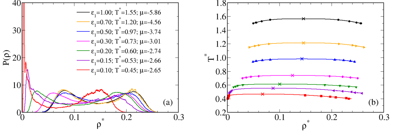
FIG. 2. Panel (a): density probability distribution P(\rho) for different \varepsilon_1 ; data are reported at reduced temperatures and chemical potentials (in unit of \varepsilon ) whereby P(\rho) first displays a double-peak behavior. Panel (b): SUS gas-liquid coexistence points (symbols) for different \varepsilon_1 , with corresponding critical points (crosses). Lines are the interpolations of simulation points obtained by the scaling law for the densities and the law of rectilinear diameters; color convention for \varepsilon_1 as in panel (a).
