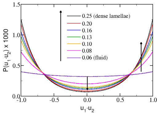
FIG. 8. Orientational order parameter P(u_1 \cdot u_2) for T^* = 0.40 and increasing pressures. The onset of the lamellar phase is seen here as a peak resolving in the |\cos(\theta)| \rightarrow 1 .
