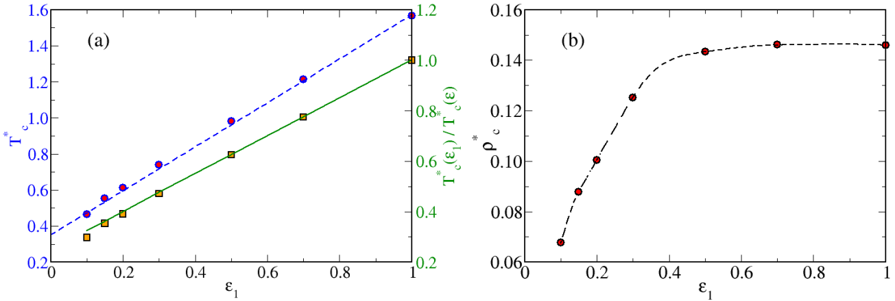
FIG. 3. Critical temperatures (panel a, circles, scale on the left, blue) and densities (panel b) as functions of \varepsilon_1 ; dashed lines are guides to the eye. In panel (a) we also show the comparison between results obtained from simulations (squares) and mean-field scaling (full line) for T_c^*(\varepsilon_1)/T_c^*(\varepsilon) (scale on the right, green).
