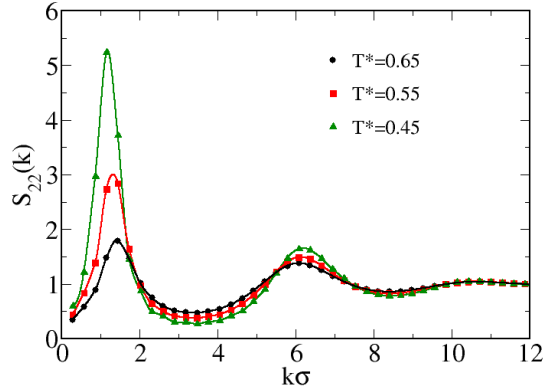
FIG. 11. Enhancement of the low- k peak of S_{22}(k) for Janus dumbbells upon lowering the temperature at fixed \rho^* = 0.20 .
