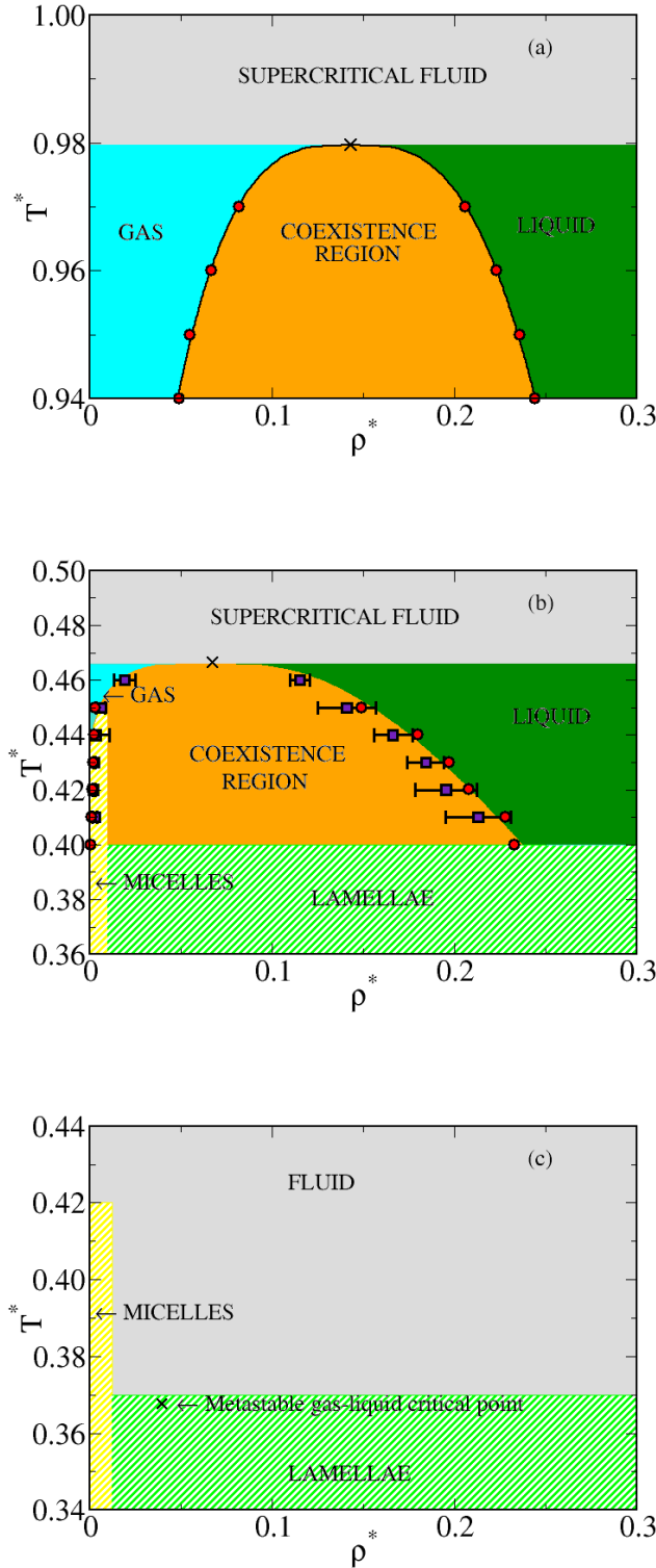
FIG. 4. Progressive schematic modification of the fluid phase diagram as estimated by SUS simulations lowering \varepsilon_1 from (a) 0.5 to (b) 0.1 till (c) 0.025. Circles are gas-liquid coexistence points whereas crosses mark the relative critical points. Squares in panel (b) are coexistence points estimated by NPT simulations.
