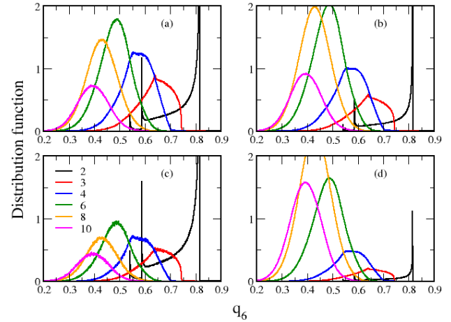
FIG. 9. Distributions of q_6 for several values of N_b (color convention in the legend of panel c). Top panels refer to T^* = 0.46 with \rho^* \approx 0.009 (a) and \rho^* \approx 0.120 (b); bottom panels, T^* = 0.42 with \rho^* \approx 0.001 (c) and \rho^* \approx 0.220 (d).
