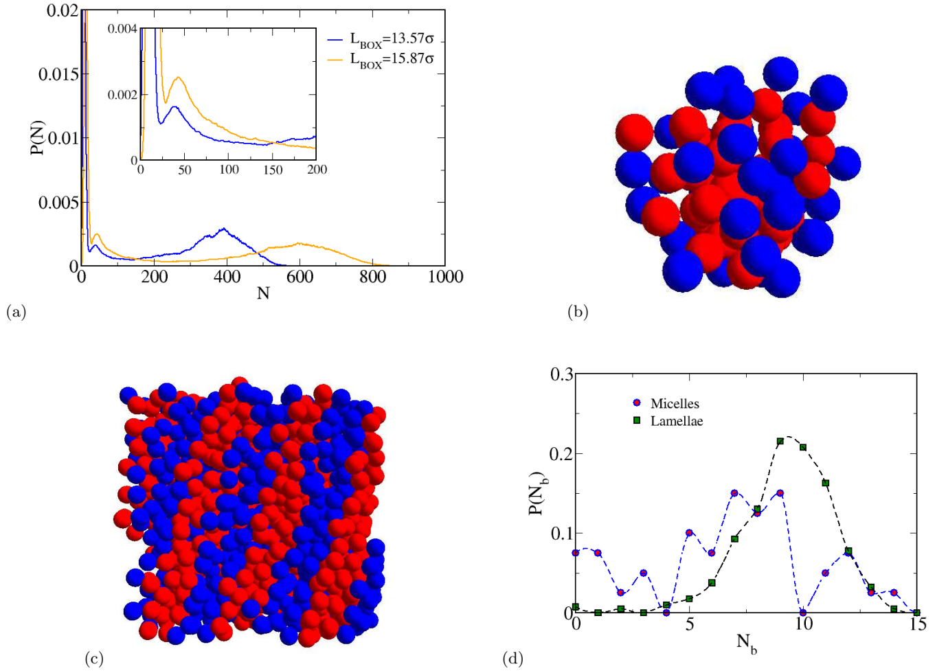
FIG. 5. Focus on the case \varepsilon_1 = 0.1 . Panel (a): probability distribution of the number of particles P(n) at T^* = 0.45 and two different box sizes with a magnification of micellar peaks in the inset. Typical microscopic configurations of self-assembled structures developed in the system, i.e. micelles (panel b) and lamellae (panel c), observed at T^* = 0.38 . Panel (d): bond probability distributions P(N_b) for different aggregates at T^* = 0.38 .
