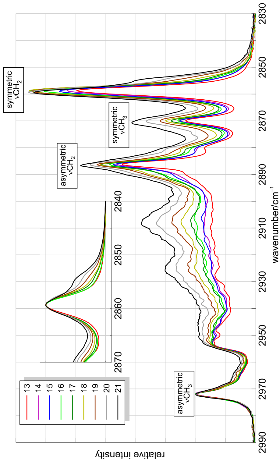
Figure 11: Averaged Raman jet spectra of alkanes in He expansions in the CH stretching region, scaled to the asymmetric methyl stretching band at \approx 2970 \text{ cm}^{-1} . The inlay illustrates the evolution of the symmetric methylene CH stretching band.
