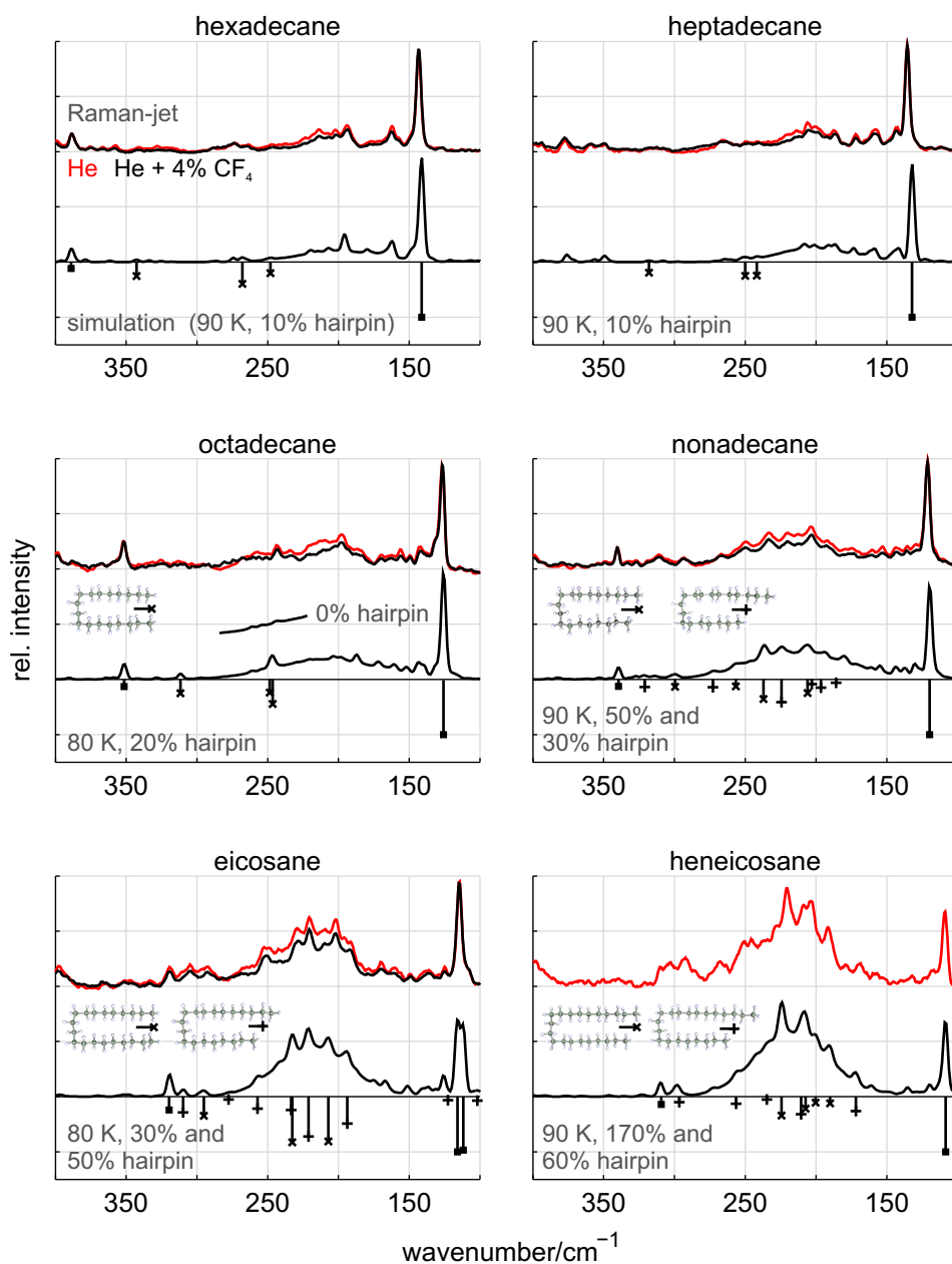
Figure 6: Comparison of averaged jet-cooled Raman spectra of n=16 – 21 in the low-frequency region to B3LYP-D3/6-311++G** simulations (He expansion in red, He+CF 4 expansions in black). For better clarity, stem plots are restricted to sufficiently Raman active all-trans conformer (squares) and hairpin conformer vibrations (upright and tilted crosses). Simulated harmonic wavenumbers are scaled: \tilde{\nu} \times 0.99 ( n=16, 18 – 21 ), \tilde{\nu} \times 0.98 ( n=17 ). Hairpin fractions in percent are relative to all-trans.
