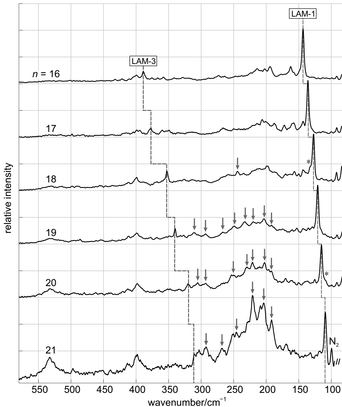
Figure 5: Averaged jet-cooled Raman spectra of the low-frequency region of alkanes with chain lengths n=16 – 21 in He expansions. Mode mixing is considered in case of n=18, 20 (marked with *). Bands assigned to hairpin conformers are marked with arrows. Air impurities ( \tilde{\nu} \leq 100 \text{ cm}^{-1} ) are prominent especially in the case of n=21 .
