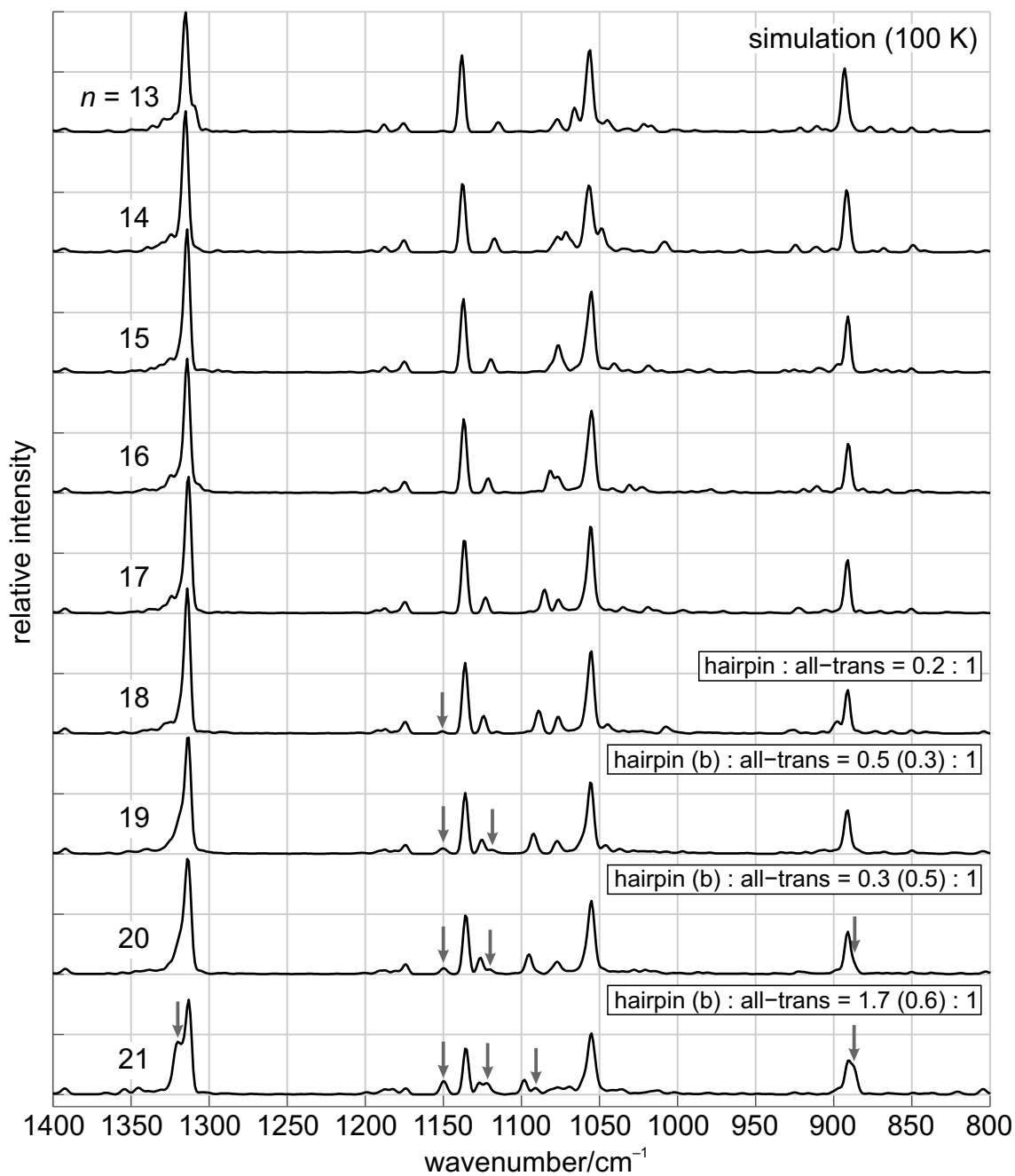
Figure 10: Simulated Raman spectra of the CC stretching region from harmonic B3LYP-D3/6-311++G** calculations (wavenumbers scaled by 0.99), see low-frequency spectra and simulations. Intensity scaled in analogy to the experimental spectra.
