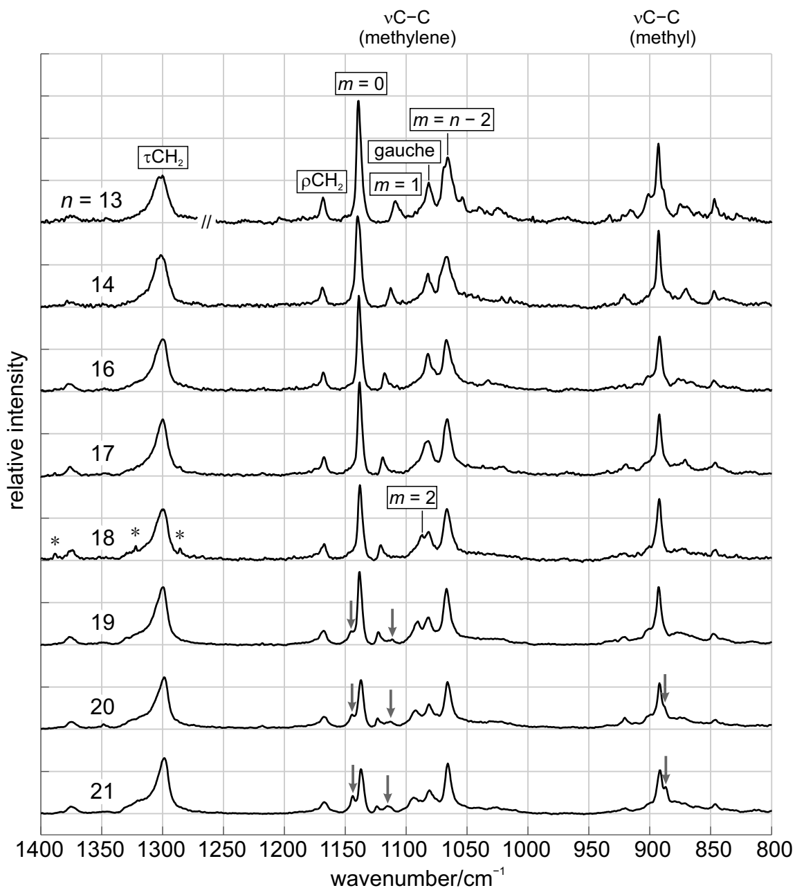
Figure 9: Jet-cooled Raman spectra of the CC stretching region of alkanes with chain length n=13, 14 , and 16-21 in He expansions, scaled to the integral of the \text{CH}_2 twisting vibration ( \rho =rocking, \nu =stretching, \tau =twisting). Bands assigned to hairpin conformers are marked with arrows, impurities with *.
