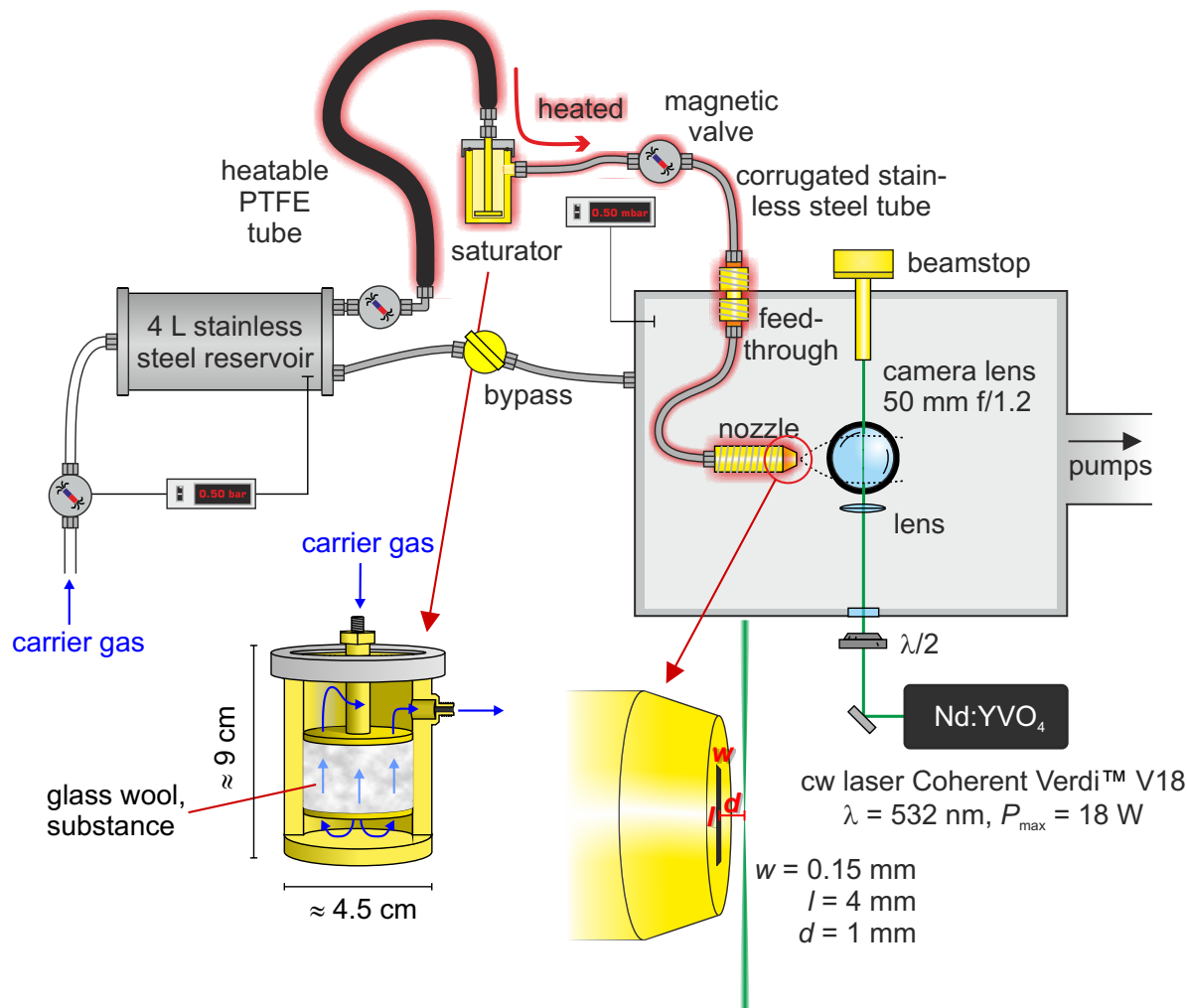
Figure 2: Sketch of the jet setup. Heating is provided by resistance heating cables or wires, wrapped around the components.
