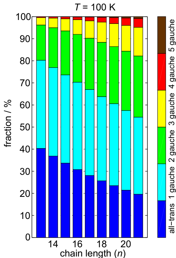
Figure 3: Conformer fractions calculated for different chain lengths at a temperature T=100 \text{ K} using a model partition function with a uniform gauche energy penalty of 2.5 \text{ kJ mol}^{-1} .
