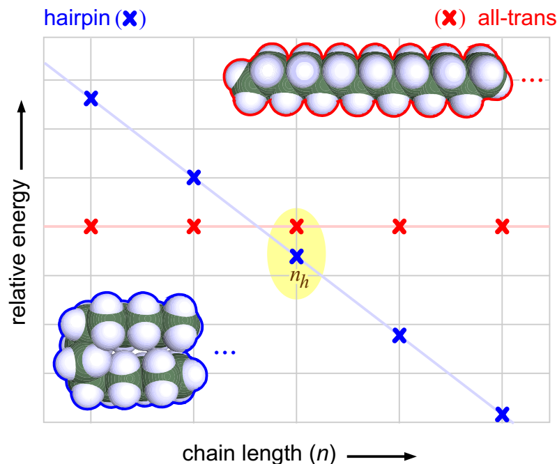
Figure 1: Cartoon of the energy of a folded hairpin conformer relative to the all-trans conformer as a function of chain length n . n_h marks the first preference for a hairpin structure.
