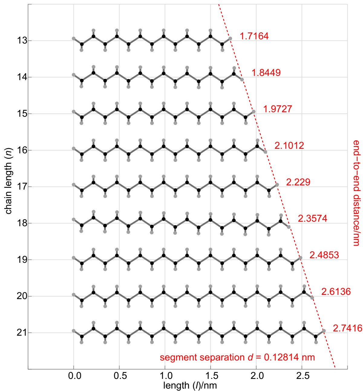
Figure 7: Projection of all-trans alkane atom coordinates on the plane spanned by the carbon atoms (optimized structures on the B3LYP-D3/6-311++G** level, Turbomole v6.4 46 ).
