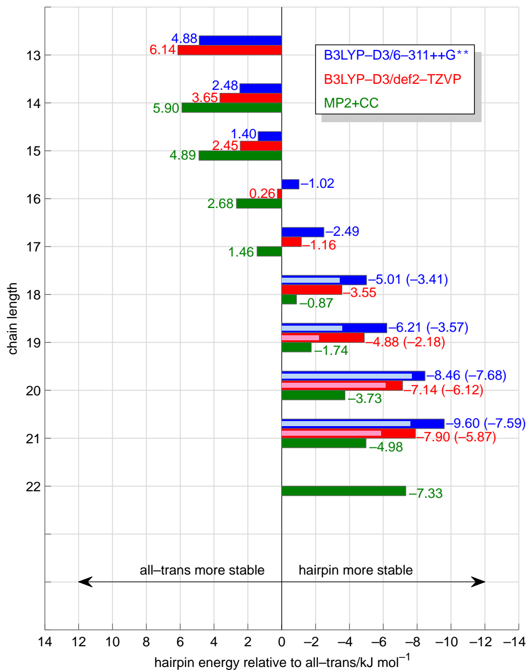
Figure 12: Energy of the hairpin conformer relative to the all-trans conformer. Blue, red and green bars comprise electronic and zero-point vibrational energy from B3LYP-D3/6-311++G**, B3LYP-D3/def2-TZVP, and a composite MP2/coupled cluster calculation (MP2+CC). 25 Energies from hairpin b conformers are drawn with light colors and are given in parentheses.
