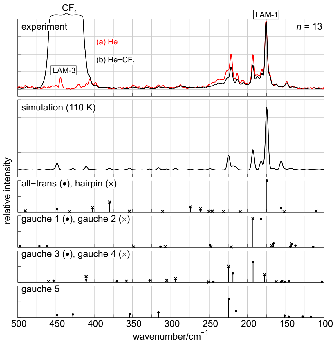
Figure 4: Comparison of averaged jet-cooled Raman spectra of tridecane in the low-frequency region to a B3LYP-D3/6-311++G** simulation. Stem plots correspond to unweighted scattering cross sections relative to the all-trans accordion vibration (LAM-1). Only vibrations with at least 1% of the accordion vibration intensity are included.
