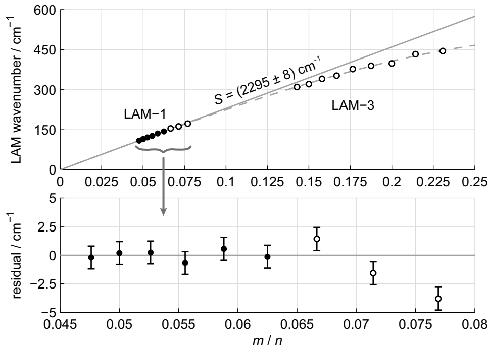
Figure 8: Extrapolation of Raman jet LAM wavenumbers (circles) of normal alkanes ( n=13 – 21 ) to infinite chain length. Tridecane, tetradecane, and pentadecane LAM-1 wavenumbers as well as LAM-3 wavenumbers are excluded from the linear fit (open circles). The complete set of wavenumbers is fitted with a third order polynomial (dashed line) to guide the eye and demonstrate non-linearity in the LAM-3 region.
