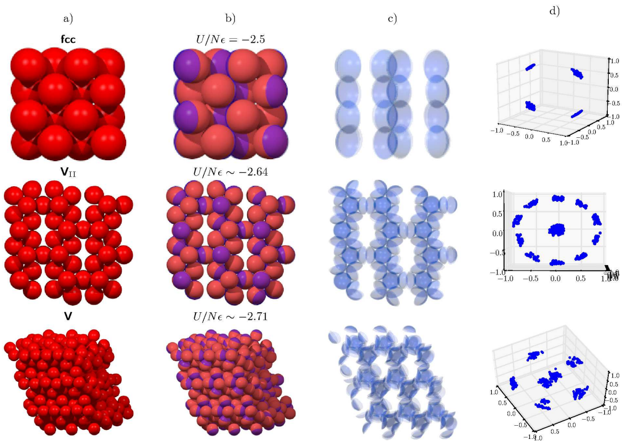
FIG. 9: Stable crystals for coverage fraction \chi = 0.3 and their energy per particle in the low-temperature limit. a) The hard cores of the particles (red); b) the hard cores of the particles as well as their bonding volumes (transparent blue); c) only the bonding volumes; d) the particle orientations, depicted on the surface of a unit sphere.
