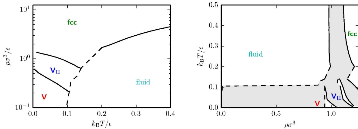
FIG. 8: Phase diagram in the T - p plane and \rho - T plane for \chi = 0.3 . The dashed line indicates estimated fluid-crystal coexistences in the region where the fluid could not be equilibrated. The symbols of crystals \mathbf{V} and \mathbf{V}_{\text{II}} are indicated on the left from their stability regions for clarity. The grey areas indicates the coexistence regions.
