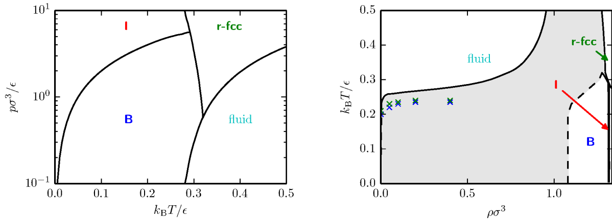
FIG. 4: Equilibrium phase diagrams for \chi = 0.6 in T-p and \rho-T representations. In the \rho-T diagram, the gray areas indicate coexistence regions, and the crosses indicate the region where lamellar clusters start forming spontaneously. In particular, for each density the blue cross denote the highest temperature where, starting from a fluid at given \rho , we observed lamellar clusters in our NVT simulations. The lowest temperature where we did not observe lamellae is indicated by a green cross. The dashed line is an estimate of where the bilayer sheets start to separate and the crystal breaks up, introducing a finite-size effect, which makes the bilayer sheets coexistence densities difficult to calculate, for further discussion see Ref. [49].
