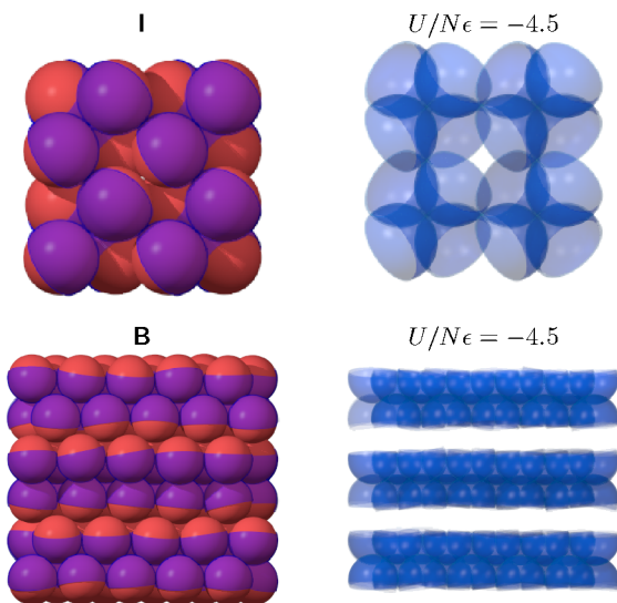
FIG. 5: Stable crystal structures and their ground-state energies for patch coverage fraction \chi = 0.6 . The particles themselves are depicted in red. The bonding volumes of the particles are shown as transparent blue regions.
