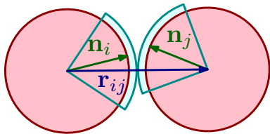
FIG. 2: Schematic representation of two patchy spheres interacting via a Kern-Frenkel potential (Eq. 1). The attractive bonding volumes are shown in blue. The vector \mathbf{r}_{ij} points from particle i to particle j . The vectors \hat{\mathbf{n}}_i and \hat{\mathbf{n}}_j show the orientations of the particles i and j .
