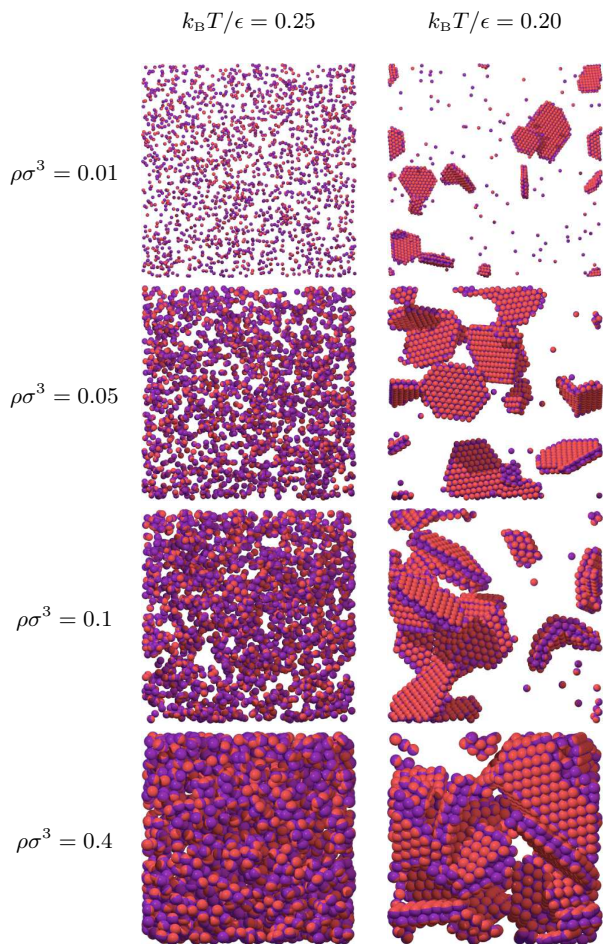
FIG. 3: Typical snapshots from constant NVT simulations of particle configurations at \chi = 0.6 , k_B T/\epsilon = 0.25 and k_B T/\epsilon = 0.20 for four number densities \rho\sigma^3 = 0.01, 0.05, 0.1 and 0.4 . The particles are depicted in red. The Kern-Frenkel interaction bonding volumes are shown as transparent blue regions.
