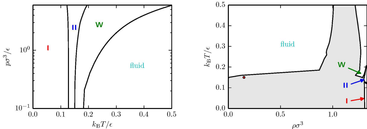
FIG. 6: Equilibrium phase diagram for the Kern-Frenkel model with coverage fraction \chi = 0.5 in the T - p and the \rho - T plane. The critical point is marked with a red dot. Note that the critical point is metastable with respect to the fluid-crystal coexistence.
