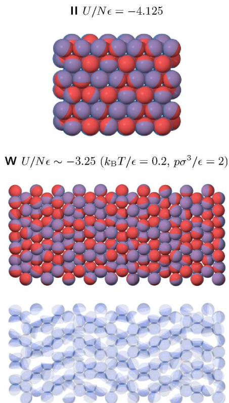
FIG. 7: Typical snapshots of parts of crystals II and W inside a rectangular box for \chi = 0.5 . The bonding volume is depicted with transparent blue. At the very bottom we show only the bonding volumes of crystal W to indicate its bonding patterns.
