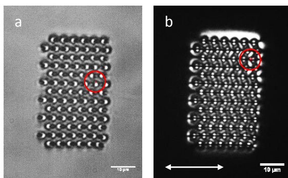
Figure 4. Optical microscopy images of a single colloidal assembly of 3.13 \mu\text{m} silica beads in a photo-polymerised nematic matrix. The image of the sample between open parallel polarisers (a) and cross polarizers (b) shows that the assembly, nor the defect lines are impacted by the laser tweezers. The center of the laser beam is at the center of the red circle.
