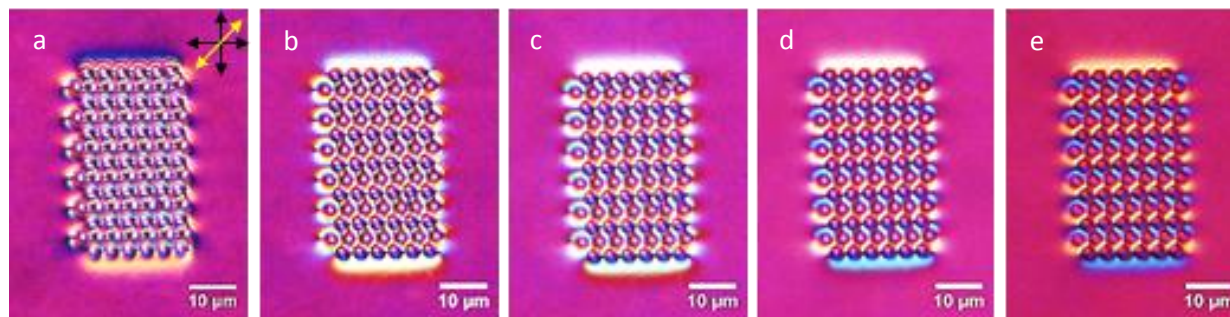
Figure 5. Optical microscopy images of a colloidal crystal of 3.1 \mu\text{m} silica particles embedded in a polymerised nematic matrix, imaged between crossed polarizers with a retardation plate added at different temperatures. The colors indicate the orientation of the optical axis of the material and therefore also the orientation of molecules around the colloidal assembly. a) 47°C; b) 71°C; c) 92°C; d) 133°C and e) >150°C, which is the maximum allowed temperature of the thermistor, used to measure the temperature. The black arrows indicate the direction of the polarizer and analyzer, the yellow arrow indicates the direction of the slow axis of the red retardation plate.
