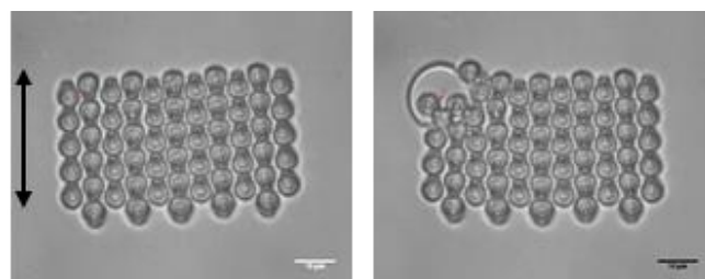
Figure 3. Optical microscopy images of a colloidal crystal of 5.01 \mu\text{m} DMOAP-silica colloids in the reactive LC medium. The right image shows the disruptive effect of laser tweezers on the assembly. The laser power is approximately 385 mW. The molten island in the left upper corner of the colloidal assembly is the isotropic phase of the LC host. The black arrow indicates the rubbing direction.
