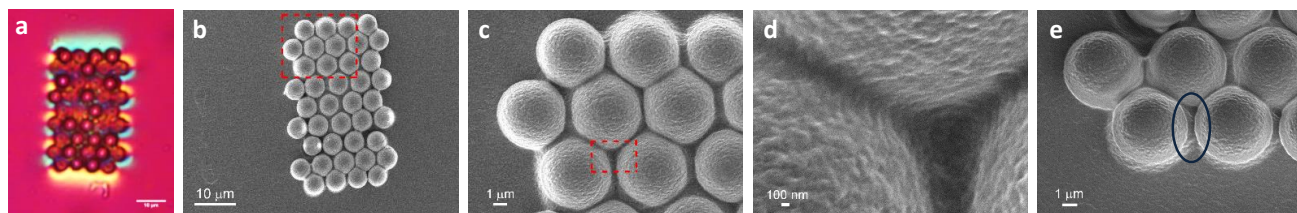
Figure 8. (a) Reflection mode Optical microscopy images of a colloidal crystal of 5 \mu\text{m} silica particles embedded in a polymerised nematic matrix after the unpolymerised LC was washed out, imaged between crossed polarizers with a retardation plate added; (b-d) SEM images of the same assembly at different magnifications; (e) SEM image of the assembly tilted by 12°. Blue ellipse indicates the region where topological defect is expected to be observed.
