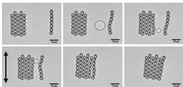
Figure 2. Sequence of optical microscopy images, showing the optical tweezers assisted assembly of chains of 3.1 \mu\text{m} DMOAP-functionalized silica microspheres in the reactive LC medium. The circular object on the images is the isotropic island produced by the laser tweezers. The maximum laser power is approximately 385 mW. The red cross indicates the position of the laser tweezers focus. The scale bar is 10 \mu\text{m} . The black double headed arrow indicates the rubbing direction, i.e. the nematic director far away from the colloidal particles.
