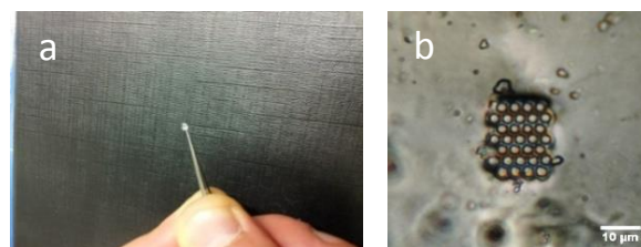
Figure 10. a) a portion of the polymer network film extracted from a cell. The portion contains a colloidal assembly which is shown in (b) imaged under polarizing microscope with only the polarizer and without the analyser.
