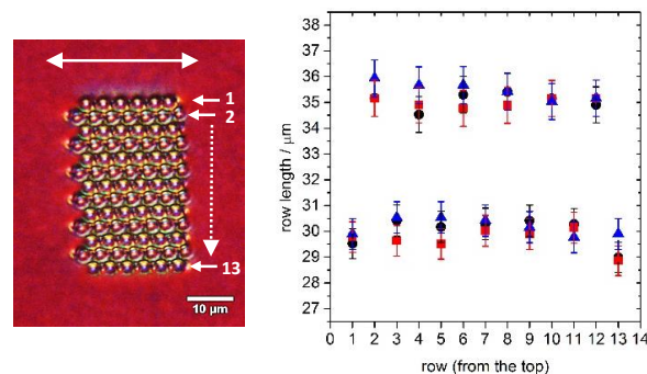
Figure 6. (left) OPM image of a colloidal crystal of 3.1 \mu\text{m} DMOAP-microspheres (left panel) in polymerised at room temperature, in the presence of a retardation plate. (right) Row lengths of the colloidal crystal before (black circles) and after (red squares) polymerisation at room temperature and after polymerisation at 150 °C (blue triangles). The rows are indicated in (a).
