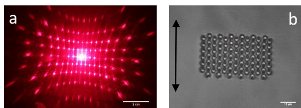
Figure 9. (a) The diffraction pattern of a He-Ne laser beam from the colloidal assembly, shown in panel (b) constituted by 3.1 \mu\text{m} silica particles; the black arrow indicates the nematic director.
