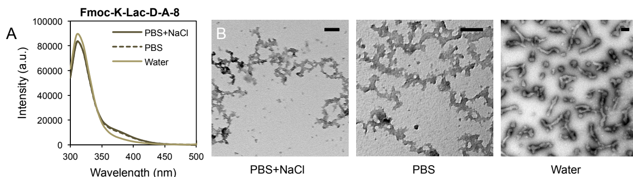
Figure 2: Fluorescence emission spectra (A) and TEM (B) of Fmoc-K-Lac-D-A-8. When prepared in PBS+NaCl and PBS at 10 mg/ml, a broad shoulder around 370 nm is observed, whereas in water the shoulder peak is not as pronounced, perhaps indicating a small degree of self-assembly. Emission spectra displayed in (A) were collected 6 days after sample preparation. TEM samples were stained with uranyl acetate, and the collected images show globular, unordered networks in ionic solutions. Short, fiber-like morphologies are observed only in aqueous solutions, indicating some self-assembly has taken place. Scale bar = 100 nm.
