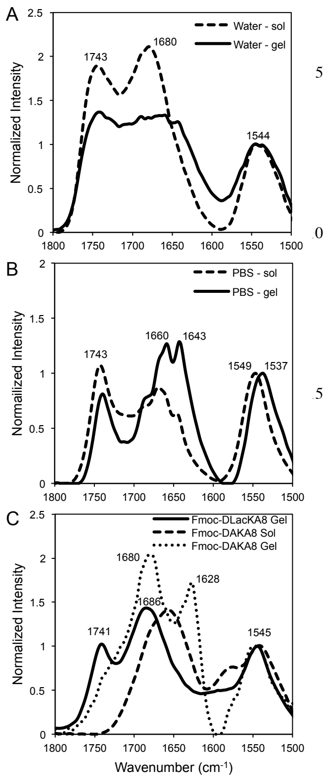
Figure 5: FTIR spectra of Fmoc-D-Lac-K-A-8. The depsipeptide was prepared in water (A) and PBS (B) in solution and in gelled form. In water, the peaks pre- and post-gelation are relatively similar. In PBS, a splitting pattern in the gelled sample at 1660 and 1643 \text{cm}^{-1} is observed. The depsipeptide gel was prepared in PBS+NaCl and compared to the peptide equivalent, Fmoc-DAKA-8 (C) in solution or as a hydrogel. All spectra were normalized to the amide II absorption peak at 1545 \text{cm}^{-1} .
