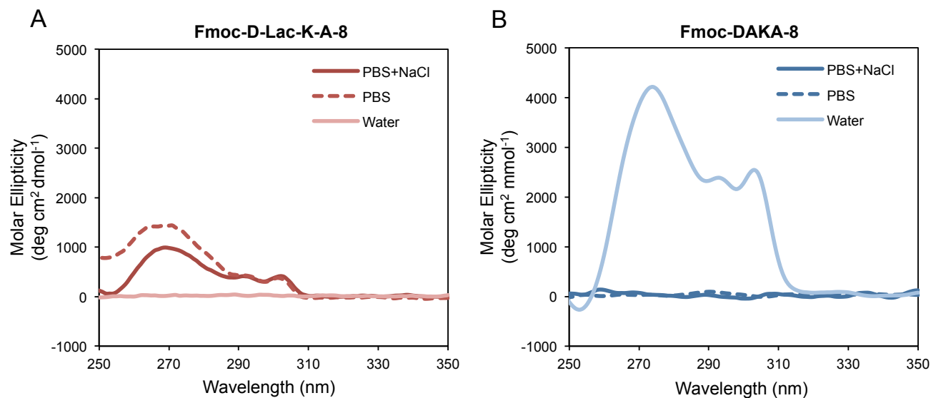
Figure 6: CD spectra of Fmoc-D-Lac-K-A-8 in PBS+NaCl, PBS, and water (A) and Fmoc-DAKA-8, the peptide equivalent (B). The depsipeptide was prepared at 10 mg/ml and aged for 4 days. In PBS+NaCl and PBS, gels formed after 2 days and 6 days respectively. Strong absorbance peaks from 270-300 nm are observed, which have been reported to be helical stacking of the Fmoc-group. No gels formed in water at the time the CD was collected. Fmoc-DAKA-8 only exhibited gelation in water due to poor solubility in PBS and PBS+NaCl, therefore only the CD spectrum of the peptide in water shows a similar positive dichroism from 270-300 nm indicating helical-like association of Fmoc groups.
