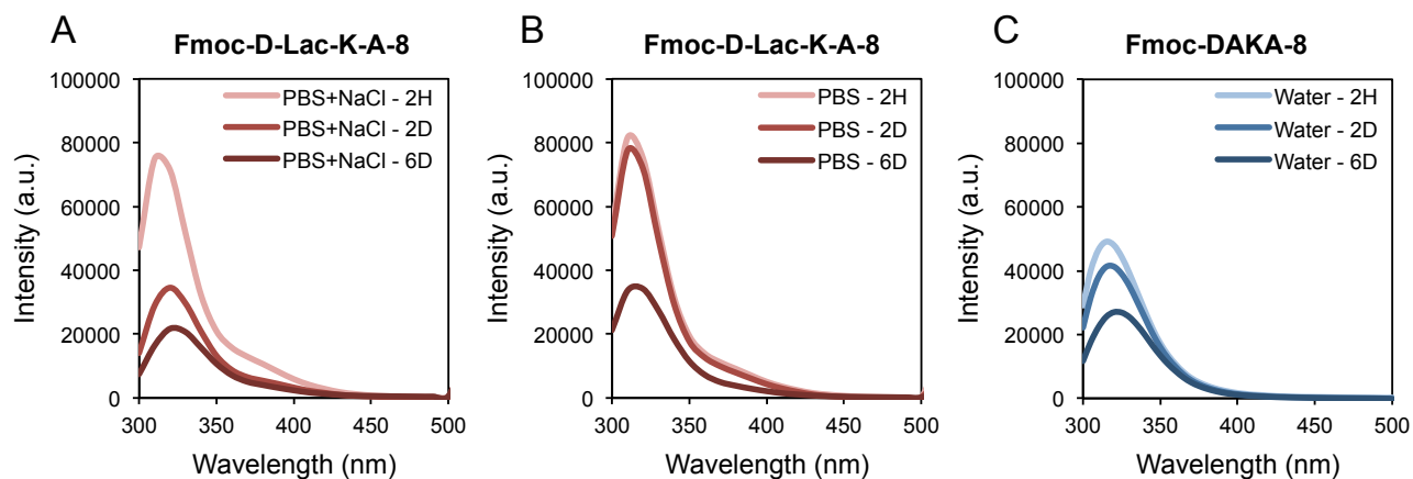
Figure 3: Fluorescence emission spectra of Fmoc-D-Lac-K-A-8 in PBS+NaCl (A) and PBS (B) were collected after 2 hours, 2 days, and 6 days. In PBS+NaCl, both a red shift from 310 to 320 nm and decrease in intensity is observed upon the formation of a gel after 2 days. Similarly, the same trend is observed in PBS after 6 days. The peptide equivalent, Fmoc-DAKA-8 forms a gel in water overnight; emission spectra were collected after 2 hours, 2 days, and 6 days in water (C).
