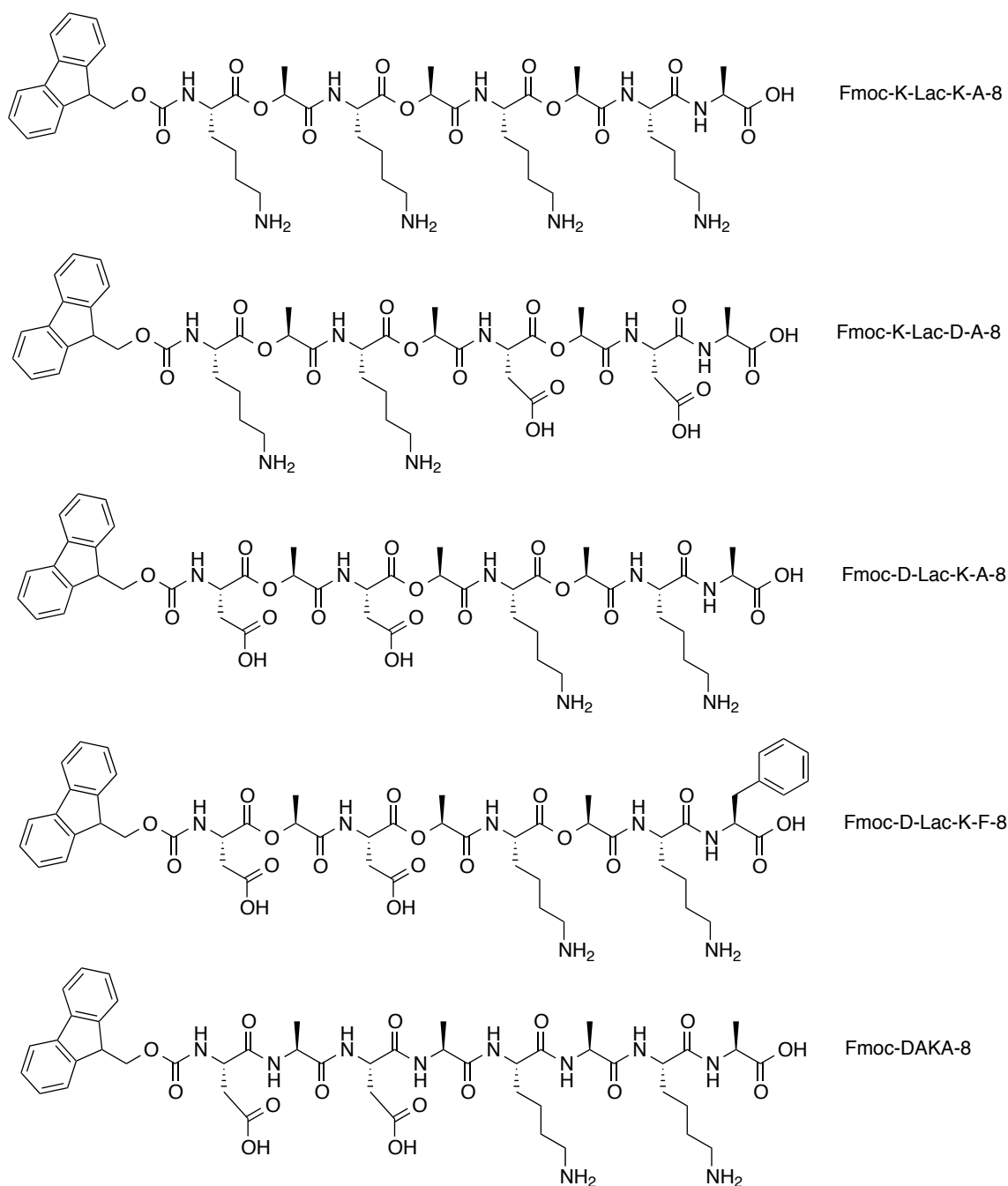
Figure 1: Depsipeptide library. The depsipeptides were named according to the N-terminal amino acid and the order of various residues, where K is lysine, Lac is lactic acid, D is aspartic acid and A or F is the residue at the C-terminus, alanine or phenylalanine respectively. The shorthand name is followed by the total number of residues. Fmoc-DAKA-8 is the peptide equivalent of Fmoc-D-Lac-K-A-8.
