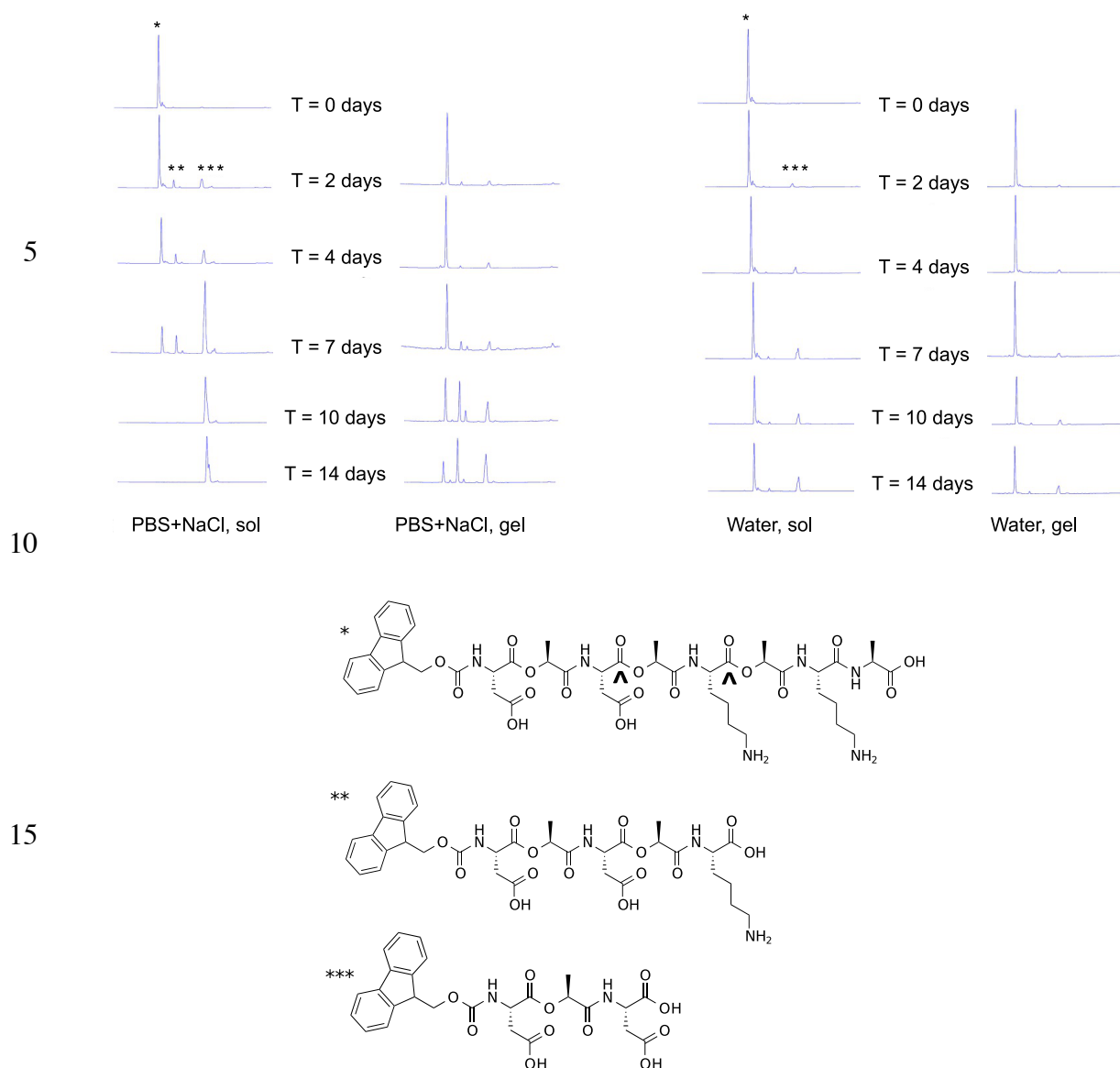
Figure 7: Degradation of Fmoc-D-Lac-K-A-8 over time. Degradation of the depsipeptide was evaluated with HPLC-MS in PBS+NaCl (top left), and water (top right) in a non-gelled and a gelled sample. The chemical structure of Fmoc-D-Lac-K-A-8, represented by the single asterisk (*) is hydrolyzed at two potential ester sites (^), to yield the two predicted degradation products, represented by a double (**) and triple (***) asterisk. As shown by peak intensity changes in the chromatograms over time, the depsipeptide in solution degrades after 2 days and is completely hydrolyzed in the presence of salt after 7 days. In the gelled form, the rate of hydrolysis is slower and is mostly degraded in PBS+NaCl after 14 days. In water, both the depsipeptide in solution and as a gel showed the slowest rate of gelation. The study conducted in PBS and the masses of these structures are provided in the ESI (Figures S2 and S3).
