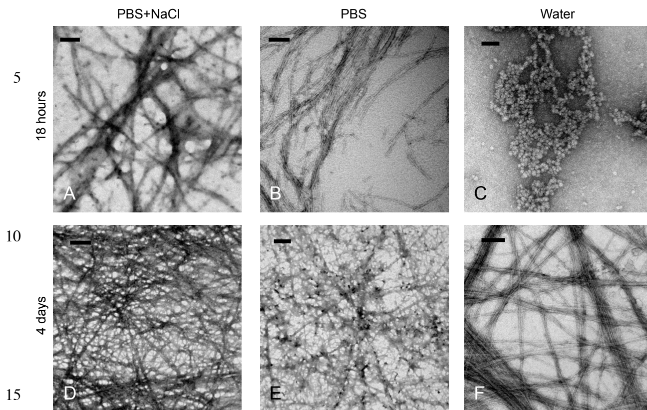
Figure 4: TEM images of Fmoc-D-Lac-K-A-8. The depsipeptide was prepared at 10 mg/ml in PBS+NaCl (A and D), PBS (B and E), and water (C and F). The images were collected after 18 hours (A-C, scale bar = 100 nm) and after 4 or 5 days (D-F, scale bar = 200 nm). After 18 hours, relatively short fiber networks are observed in PBS+NaCl and PBS, while globular aggregates are shown in water. After 4 or 5 days, fibers are observed for all samples.
