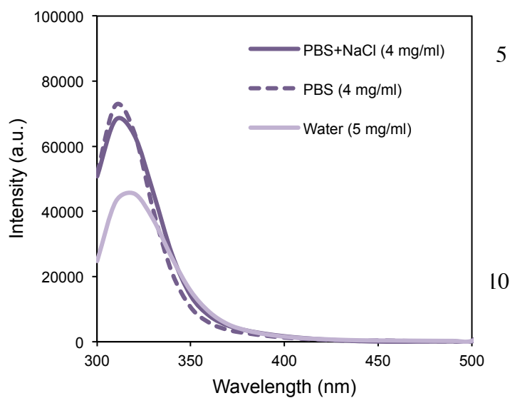
Figure 8: Fluorescence emission spectra of Fmoc-D-Lac-K-F-8. In water, a peak at 320 nm is observed and the depsipeptide also forms a gel under those conditions. The observed peaks at 310 nm in PBS and PBS+NaCl reflect the absorbance of the fluorenyl group in solution, as gels did not form under these conditions.
