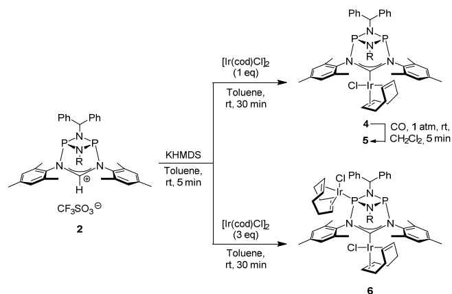
Scheme 2 Metalation of Carbene 3 .
