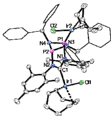
Figure 8 Molecular structure of 6 , thermal ellipsoids set at the 50% probability level. H-atoms have been omitted for clarity. Phenyl rings of the benzhydryl substituents are drawn as wireframes. Selected bond lengths [Å] and angles [°]: Ir1-C1 2.046(3), Ir2-P1 2.2359(8), P1-N1 1.756(3), N1-C1 1.385(4), Ir2-P1-P2 158.50(4), N2-C1-N1 114.9(3).
