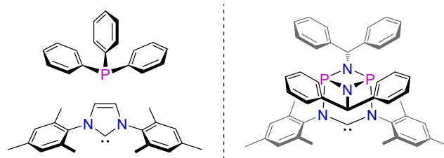
Figure 2 Spatial characteristics of phosphines, NHCs (left) and the targeted 3-dimensional hybrid phosphazane/NHC ligand (right).
