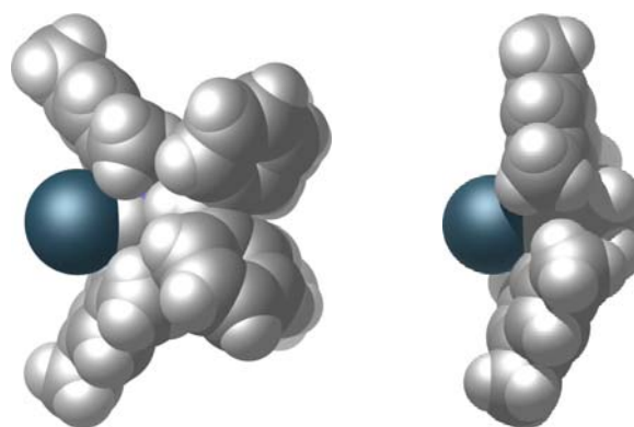
Figure 10 CPK model of the van der Waals surface of complex 4 (left) and, for comparison complex SIMes[ [\text{Ir}(\text{cod})\text{Cl}] ] (right). Cyclooctadiene and chlorido ligands have been omitted for clarity.
