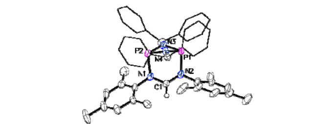
Figure 3 Top: One-pot access to the cationic cyclophosphazane cage compound 2 . Bottom: Molecular structure of 2 , thermal ellipsoids set at the 50% probability level. H-atoms except H(1) and the trifluoromethanesulfonate counterion have been omitted for clarity. Phenyl rings of the benzhydryl substituents are drawn as wireframes. Selected bond lengths [Å] and angles [°]: P1-N2 1.837(3), P1-N3 1.704(3), N1-C1 1.323(4), N2-C1-N1 122.7(3).
