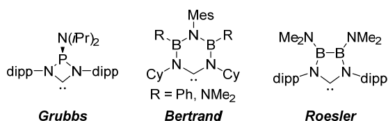
Figure 1 Selection of “inorganic” carbenes.
