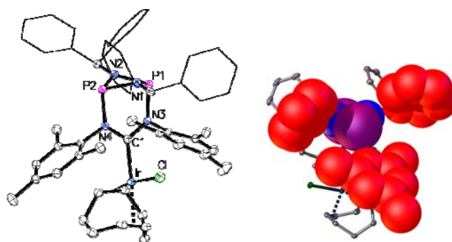
Figure 6 Left: Molecular structure of 4 , thermal ellipsoids set at the 50% probability level. H-atoms have been omitted for clarity. Phenyl rings of the benzhydryl substituents are drawn as wireframes. Selected bond lengths [Å] and angles [°]: Ir-C1 2.040(2), P1-N3 1.7658(19), N3-C1 1.372(3), N3-C1-N4 114.06(19). Bottom: Space-filling representation of one of the C_3 -symmetric binding pockets. Phenyl and mesityl ring marking the boundary of the cavity are highlighted in red.
