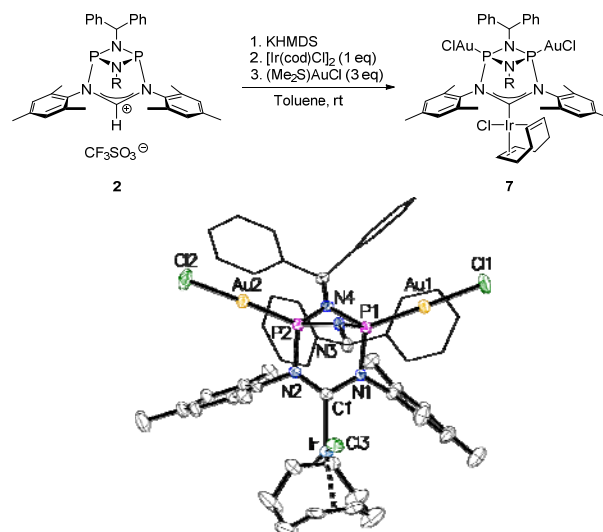
Figure 9 Top: Access to the trimetallic complex 7 . Bottom: Molecular structure of 7 , thermal ellipsoids set at the 50% probability level. H-atoms have been omitted for clarity. Phenyl rings of the benzhydryl substituents are drawn as wireframes. Selected bond lengths [Å] and angles [°]: Au1-P1 2.1839(10), Ir-C1 2.020(4), P1-N1 1.719(4), P1-N3 1.712(4), N1-C1 1.390(5), N2-C1-N1 115.3(4).
