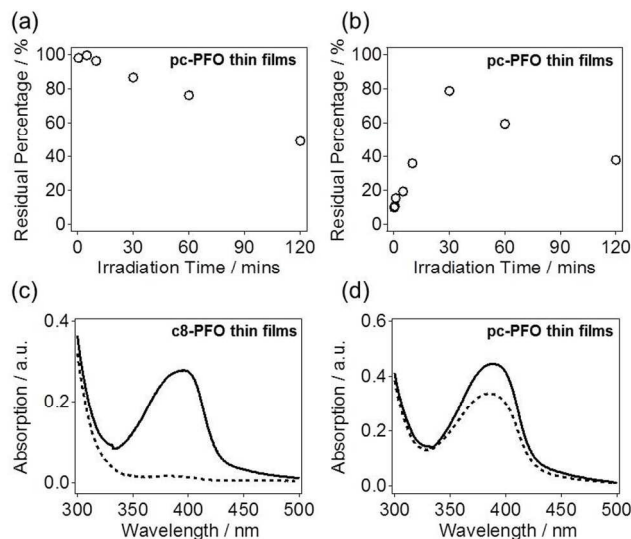
Figure 2. Time series plots of photocrosslinking time versus pc-PFO thin-film residual percentages. The pc-PFO thin-film residual percentages were calculated by dividing the intensity of the absorption peak of pc-PFO thin films (a) after photocrosslinking and (b) after THF wash by the value before photocrosslinking. UV-vis absorption spectra of (c) uncrosslinked c8-PFO and (d) 30-mins photocrosslinked pc-PFO spin-coated thin films before (solid line) and after (dashed line) the immersion and wash in THF.
