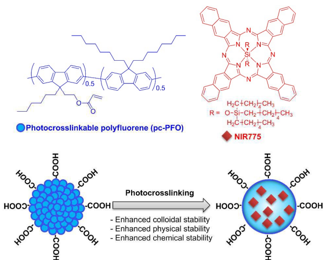
Figure 1. Schematic showing the chemical structures of the photocrosslinkable Pdots used in this study and the NIR dye used for demonstrating stable small-molecule encapsulation into crosslinked Pdots.
