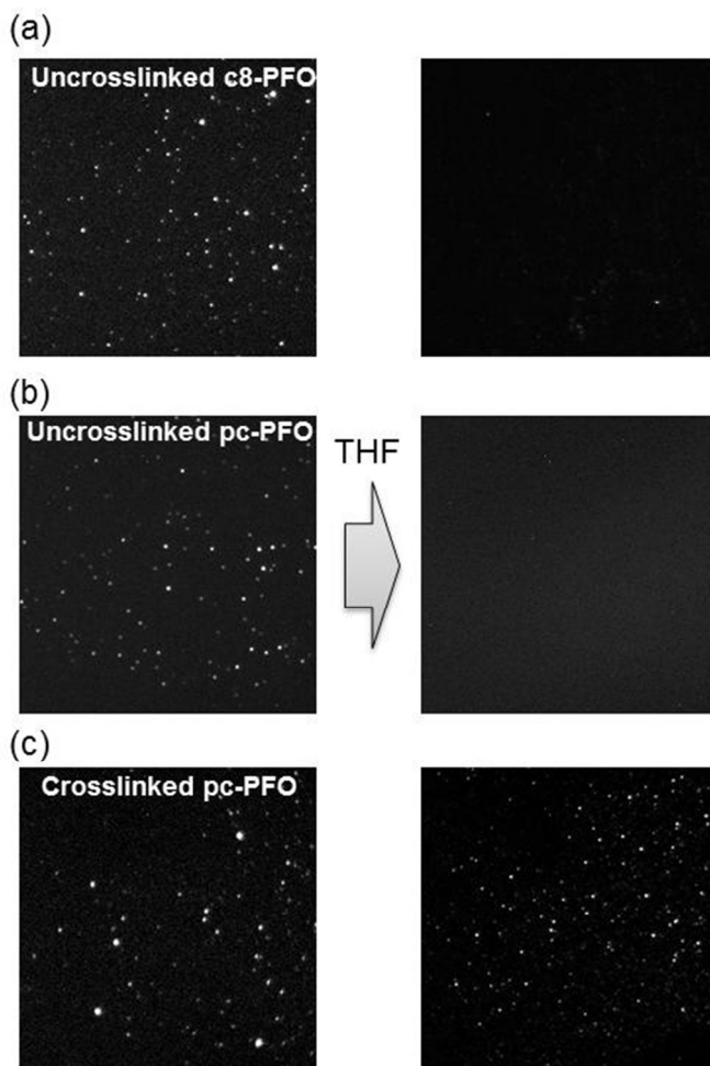
Figure 5. Fluorescence images of (a) uncrosslinked c8-PFO, (b) uncrosslinked pc-PFO Pdots, and (c) 30-min photocrosslinked pc-PFO Pdots before (left) and after (right) the immersion in THF.
