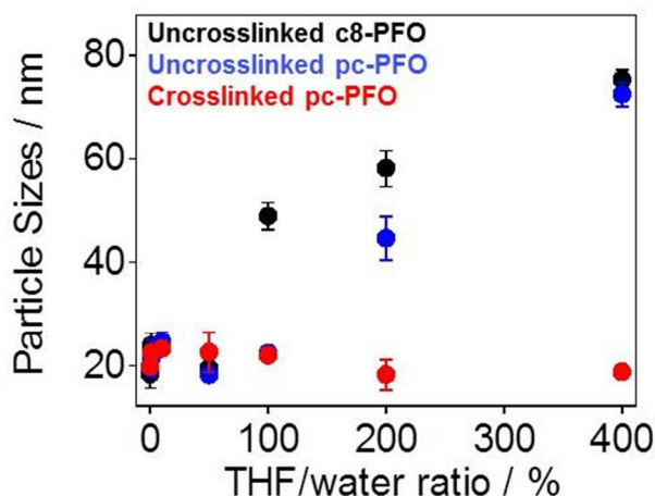
Figure 4. Particle sizes and error bars of uncrosslinked c8-PFO (black), uncrosslinked pc-PFO (blue), and crosslinked pc-PFO (red) Pdots in aqueous solution after being swelled by various amounts of THF solvent.
