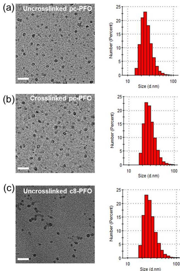
Figure 3. Transmission-electron-microscopy images (left) and histograms showing the distribution of the sizes of Pdots as measured by dynamic-light-scattering (right) of (a) uncrosslinked pc-PFO Pdots; (b) 30-mins photocrosslinked pc-PFO Pdots; (c) uncrosslinked c8-PFO Pdots. Scale bar: 100 nm.
