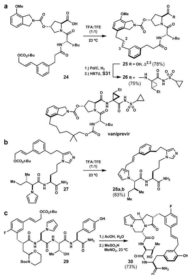
Figure 5. Template design permits incremental variation of product structure. (a) Template 1 allows facile synthesis of vaniprevir analog 26, (b) Three-component coupling of 2 and macrocyclization accesses imidazole-linked macrocycles (e.g. 28a,b). (c) Bi-functional template 3 initiates P1 cyclization and large ring-forming alkylation (e.g. 30). HBTU = O -(benzotriazol-1-yl)- N,N,N',N' -tetramethyluronium hexafluorophosphate
