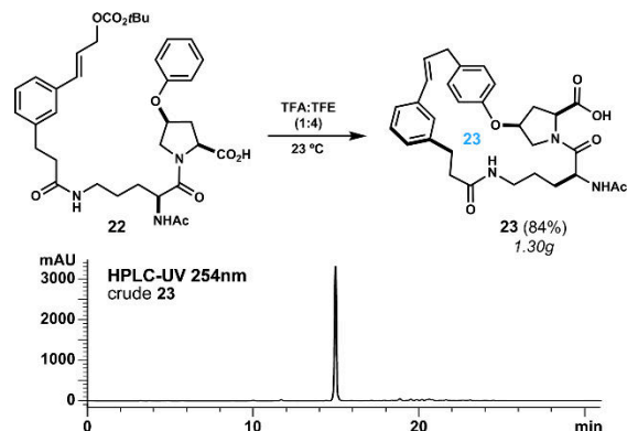
Figure 4. Selective, gram scale synthesis of the 23-membered ring 23 , the macrocyclic core of compounds 16a and 18a . HPLC-UV analysis (C18, 4.6x250 mm 5 \mu , 30 \rightarrow 60% ACN + 0.1% TFA, 1 mL/min) following concentration of the crude reaction mixture. TFE = 2,2,2-trifluoroethanol.
