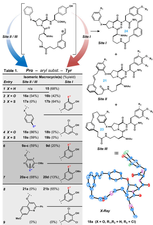
Figure 3. Nucleophile survey within the scaffold Ac-Orn(1)-Pro(X-Ar)-Tyr . Macrocyclization can be tuned for selective or divergent outcome using substituent effects or blocking groups. Alkylation at sites I, II and III accesses 24, 21 and 23-membered rings, respectively (ring size indicated in blue; E^P = aryloxypropyl linkage, E^T = tyrosyl linkage).
