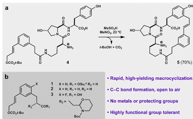
Figure 1. Unprotected peptides acylated with a cinnamyl carbonate-containing template readily macrocyclize in acidic media. (a) Large ring-forming Friedel-Crafts alkylation is insensitive to polar protic functional groups. (b) Template structures used in this work. a 75 mM MeSO 3 H in MeNO 2 , 5 mM in 4 , for 2 hr. b Su = N -succinimidyl.
