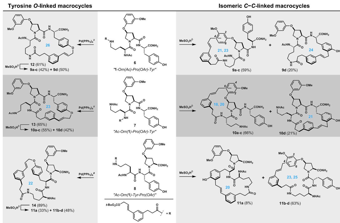
Figure 2. Cyclized product distributions track arene electronics and are responsive to conformational pre-organization. Linear peptidic precursors 6 – 8 undergo facile large ring-forming Friedel-Crafts alkylations, or tyrosine O -alkylation when treated with protic acid or Pd 0 , respectively. Acidolysis of conformationally pre-organized macrocyclic cinnamyl tyrosyl ethers 12 – 14 favors intra-side-chain O → C ortho isomerization in comparison to direct ring-forming reactions. a 10 mol% Pd(PPh 3 ) 4 , DMF, 5 mM in substrate, 1-2 h, 23 °C. b 75 mM MeSO 3 H in MeNO 2 , 5 mM in substrate, 2 h, 23 °C.
