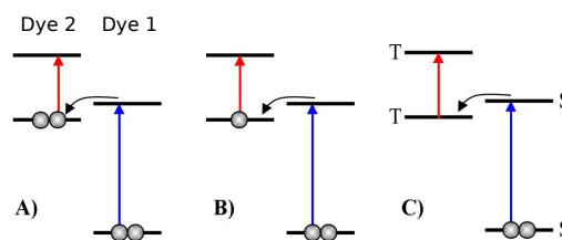
Fig. 1 Various proposed energy level schemes for solar cells based on two dye molecules connected by a molecular diode (molecular linker not shown here, see Fig. 3 below). The occupancy is given for the ground state. A) Simplest concept with both HOMOs doubly occupied. Both dye molecules need to be excited at the same time to generate a hole in the upper HOMO that can take up an electron from the lower LUMO. That is unlikely to happen in the same tandem complex. B) The upper HOMO is partially occupied to allow facile charge transfer between the two dye molecules. Such a situation can be realized in metal-organic dye molecules with an odd number of electrons. This is the analog of an intermediate band solar cell. 27–29 C) Using singlet (S) and triplet (T) excitations. The long lifetime of the triplet allows a significant electron population to accumulate in the lower triplet level, which can be excited by into the upper triplet level. This scheme could also be realized with a single dye molecule.
