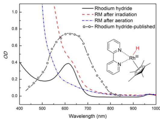
Figure 3: Spectroscopic evidence of presence of \text{Rh}(\text{III})\text{-H} in the photocatalytic system (left side). Spectra of a typical reaction mixture after irradiation (dashed red line), after bubbling with air (dash – dotted blue line), of a prepared \text{Rh}(\text{III})\text{-H} standard (solid black line), and a published 24 spectrum (open circles + dashed line; redrawn from the original) are shown.
