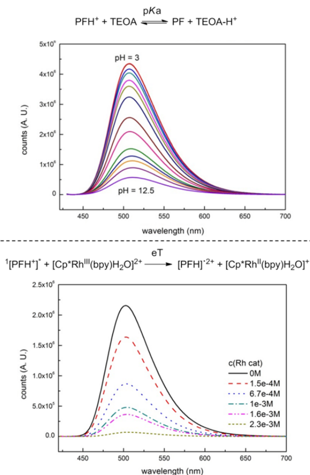
Figure 2: Fluorescence quenching of PF with TEOA (upper part) and \text{Rh}_{\text{cat}} (lower part).
