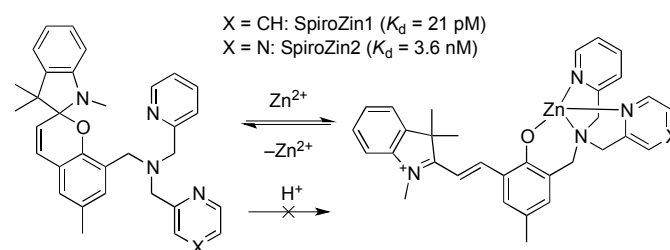
Scheme 1. Structure and sensing mechanism of SpiroZin probes. Replacement of a pyridine (X = CH) by a pyrazine ring (X = N) in the metal-chelating unit decreases the zinc binding affinity of the sensor, improving its dynamic range in live cells. 17
