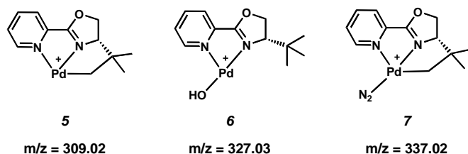
Figure 1: Suggested structures for selected species identified when a solution of ligand 4 and \text{Pd}(\text{OCOCF}_3)_2 is analyzed by DESI-MS.
