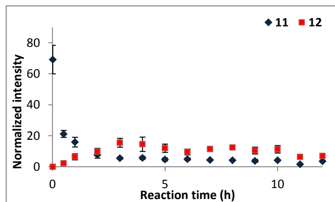
Figure 4: Monitoring of intermediates 11 and 12 by DESI-MS.
