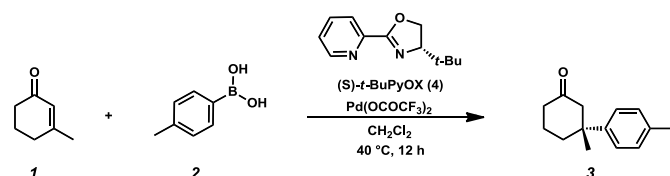
Scheme 1: Asymmetric conjugate addition of arylboronic acids to cyclic enones catalyzed by Pd(OCOCF 3 ) 2 and t -BuPyOX.
