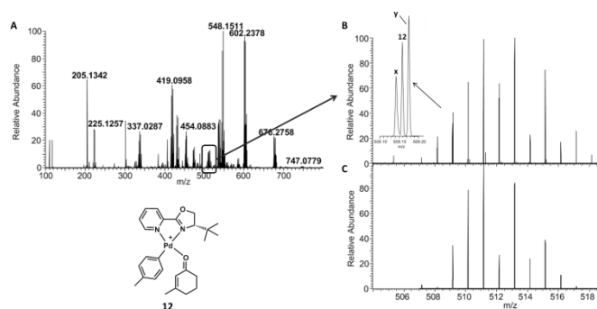
Figure 3A: Incubated reaction sampled and mass analyzed after 8 h B . Experimental spectrum of 12 . The signal is overlaid by x [(\text{PyOx})_2\text{Pd}]^+ ( m/z 513.14) † and y [(\text{PyOx})\text{Pd}(\text{phenyl})_2]\text{NH}_4^+ ( m/z 510.17) C . Simulated spectrum of 12 .
