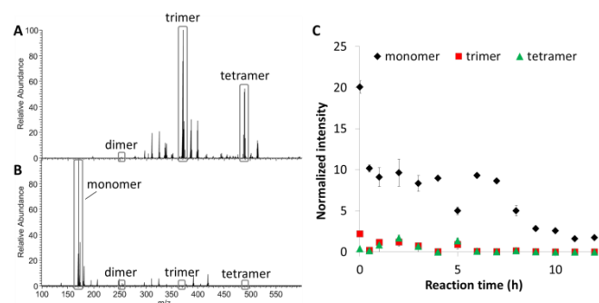
Figure 5A: 1 mmol 2 spotted on a surface and sprayed with CH 2 Cl 2 . Dimer, trimer, and tetramer were detected as OH-adducts in negative ion mode. B. Distribution of 2 after reaction completion. C. Reaction monitored over 12 h. Ion intensities are normalized to the total ion count.
