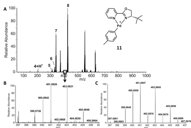
Figure 2A: 1 mmol Pd source and ligand sprayed with 0.1 mmol p -tolylboronic acid B . Experimental spectrum of 11 C . Simulated spectrum of 11 .
