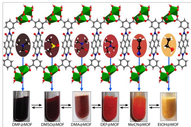
Figure 2. Schematic representation of Mg–NDI crystals showing different colors in different solvents. Hypsochromic shift was found to be observed with the increase in polarity of the solvent medium.
