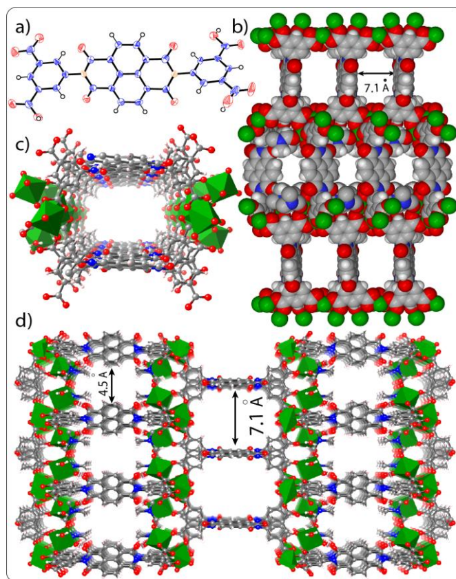
Figure 1. (a) ORTEP diagram of H 4 BINDI; (b) space filled diagram of Mg–NDI; (c) perspective view of a single pore and (d) perspective view of the extended structure of Mg–NDI.
