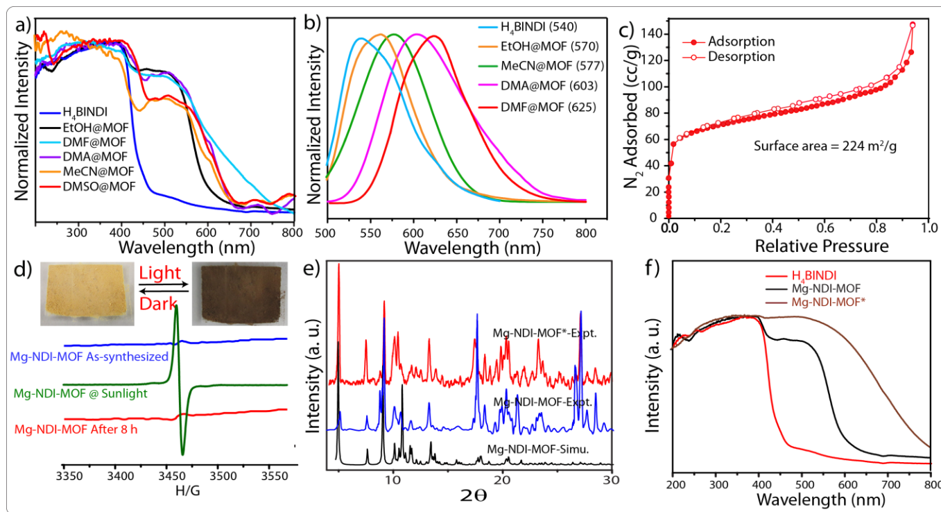
Figure 3. (a) Solid state UV-vis spectra, (b) solid state photoluminescence of Mg-NDI crystals soaked in different solvents; (c) N 2 adsorption isotherm for Mg-NDI; (d) ESR spectra of Mg-NDI crystals before and after irradiation of sunlight; (Inset) photograph representing the reversible photochromic behavior of Mg-NDI MOF crystal in sunlight and dark; (e) PXRD patterns of Mg-NDI crystals before and after irradiation of sunlight; (f) solid state UV-vis spectra of H 4 BINDI (red), Mg-NDI (black) and Mg-NDI* (brown).
