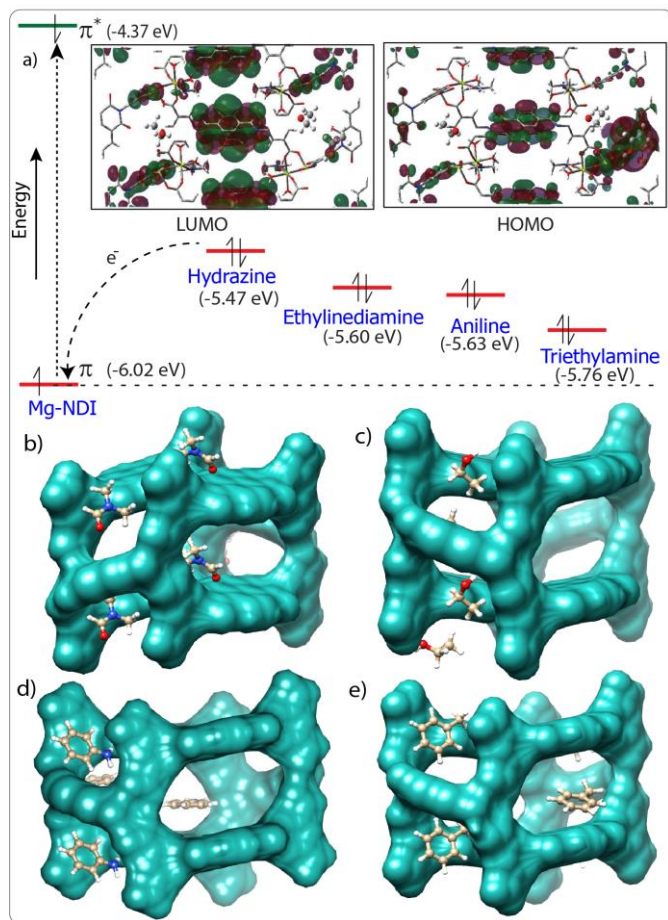
Figure 5. (a) HOMO ( \pi ) and LUMO ( \pi^* ) energy levels of Mg-NDI and different amines. The inset shows contour plots of the HOMO and LUMO for Mg-NDI. Energy optimized structures of (b) DMF, (c) EtOH, (d) Aniline and (e) Toluene incorporated Mg-NDI has been represented.
