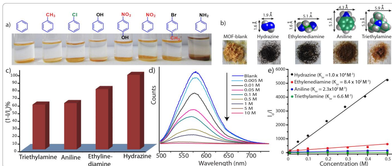
Figure 4. (a) Photograph of selective detection of aniline over other aromatic functional molecules; (b) photograph showing the color change of Mg-NDI samples in presence of different amines (0.1 M); (c) bar chart representation for quenching efficiency of Mg-NDI in presence of different amines (0.01 M) in EtOH; (d) reduction of PL emission intensities of Mg-NDI by gradual increase in concentration of aniline; (e) Stern-Volmer plot for Mg-NDI with different amines.
