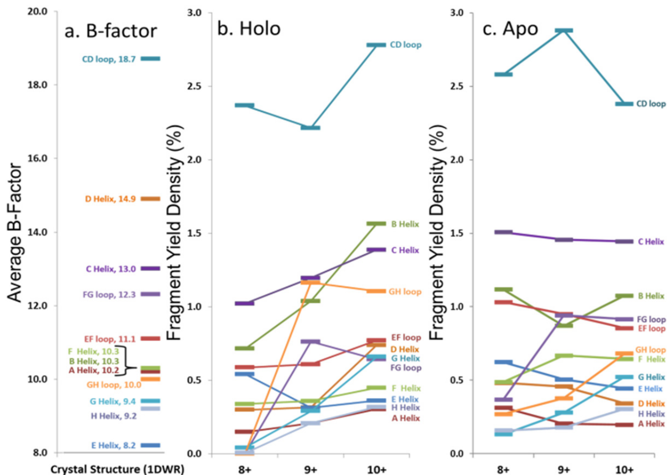
Figure 5. Comparison of average (a) B-factor values and fragment yield densities of respective labelled regions from the (b) holo and (c) apo forms of myoglobin for the three native-like charge states. Regions with greater B-factors or fragmentation yield densities indicate less stable regions whereas those with lower values indicate more stable regions. The C- and N-termini have been removed from the figure. Standard deviations for fragment yield densities are given in Figure 4 and Figure S2 for holo and apo forms, respectively.
