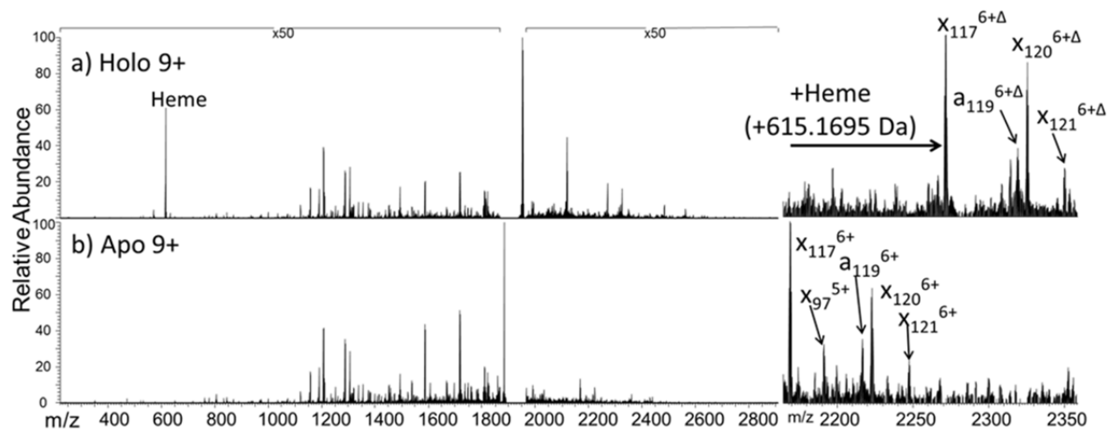
Figure 1. 193 nm UVPD mass spectra of the 9+ charge state of the a) holo and b) apo form of myoglobin. Panels to the right are expanded regions ( m/z 2175 to 2350) with several ions labelled to illustrate the mass shift (+615.1695 Da) affiliated with retention of the heme group. \Delta indicates the inclusion of heme in the fragment ions. The 50x amplification applies to both spectra.
