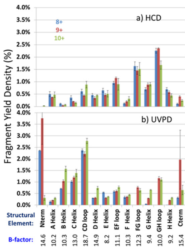
Figure 4. Normalized fragmentation yields averaged over the total number of amino acids in each structural element for charge states 8+ (blue bars), 9+ (red bars), and 10+ (green bars) of holomyoglobin for (a) HCD and (b) UVPD. Numbers under the structural regions show the calculated average B-factors for holomyoglobin.
