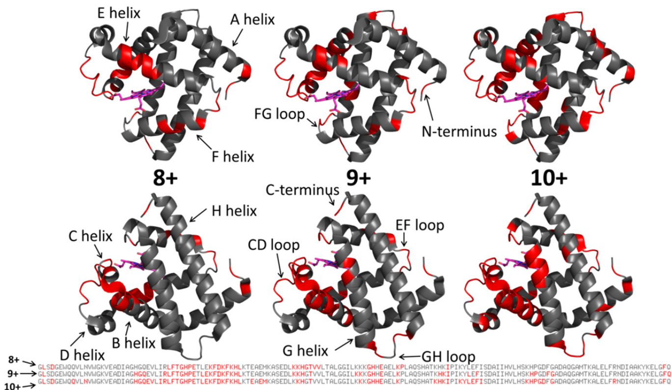
Figure 3. Those residues that were found to have enhanced backbone cleavage frequencies upon UVPD activation are highlighted in red on the holo-myoglobin crystal structure 1DWR, as also indicated in the primary sequence below for the native charge states (8+, 9+, 10+) evaluated. The heme group is shown as a hot pink color. The 1DWR crystal structure has been rotated 180° about the x-axis between the top and bottom structures.
