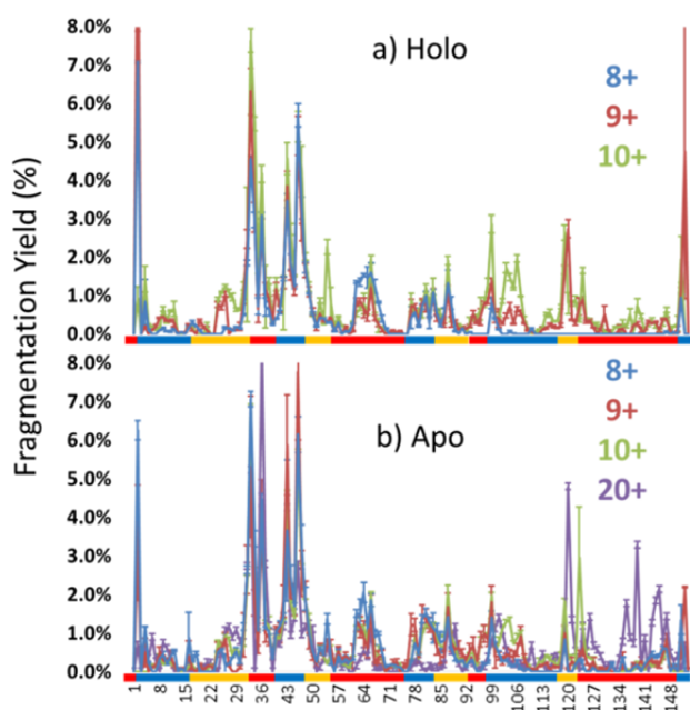
Figure 2. Normalized fragmentation yields upon UVPD of the 8+ to 10+ charge states for both a) holo and b) apo forms based on averaging 3-4 replicates. The fragmentation yields for the 20+ denatured state of apo-myoglobin are shown in b as well. Structural regions are demarcated below the graphs with colored bars showing the loops and helices.
