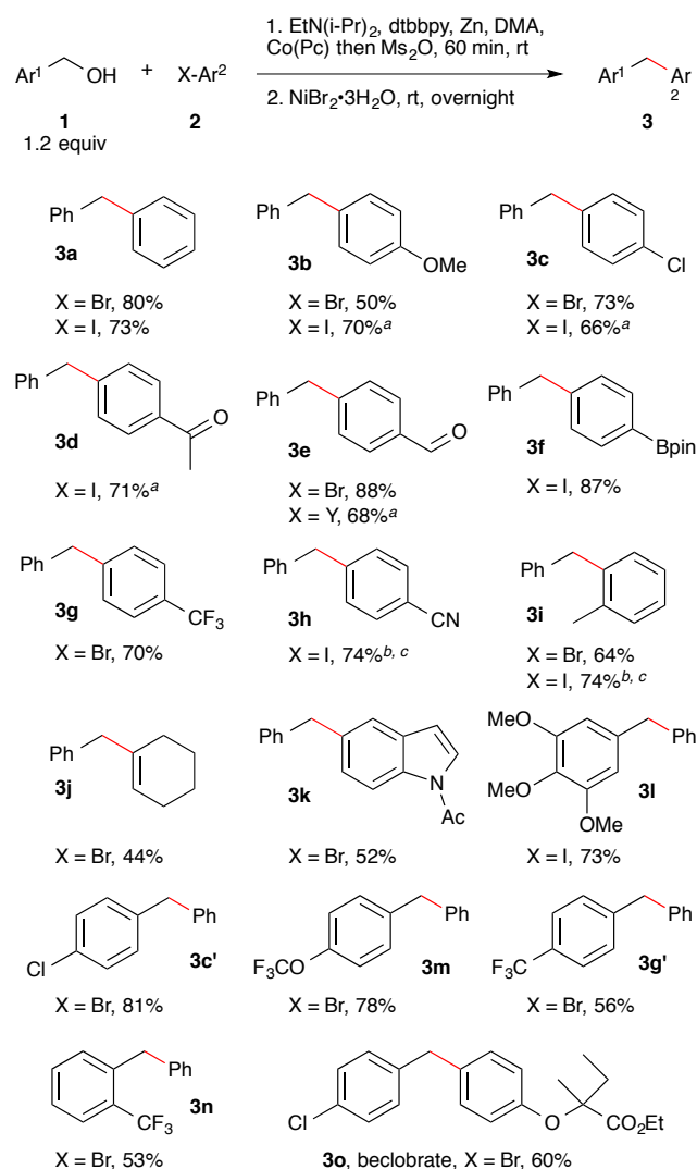
Scheme 2. Nickel and cobalt co-catalyzed arylation of benzyl mesylates. Reactions performed as in Table 2, footnote a with 7 mol% NiBr 2 ·3H 2 O, 5 mol% dtbbpy, and 1 mol% Co(Pc). Yield is isolated yield of purified product. See Supporting Information for details on reaction selectivity. ND = not detected. a No Co(Pc) was added to this reaction. b 3 mol% Co(Pc) was added to this reaction. c Reaction was run at 60 °C.
