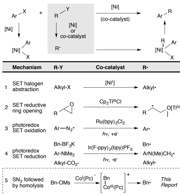
Figure 1. Comparison of radical co-generation methods in cross-coupling. An electrophile (Ar-X) reacts to form an arylmetal intermediate and the other substrate (R-Y) reacts to form a radical (R•).
