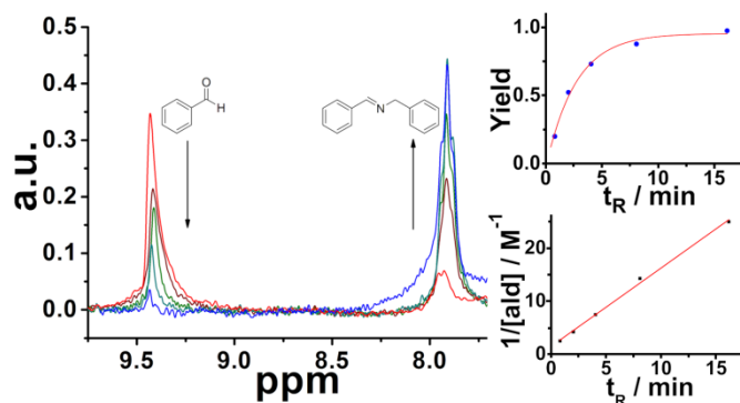
Fig. 1 Imine synthesis monitored by in-line NMR. Left: Superimposition of the spectra recorded. Right up: Yield as a function of the residence time. Yield calculated as A_{\text{im}}/(A_{\text{im}}+A_{\text{ald}}) . Right down: fitting of the experimental results to second-order kinetics.
