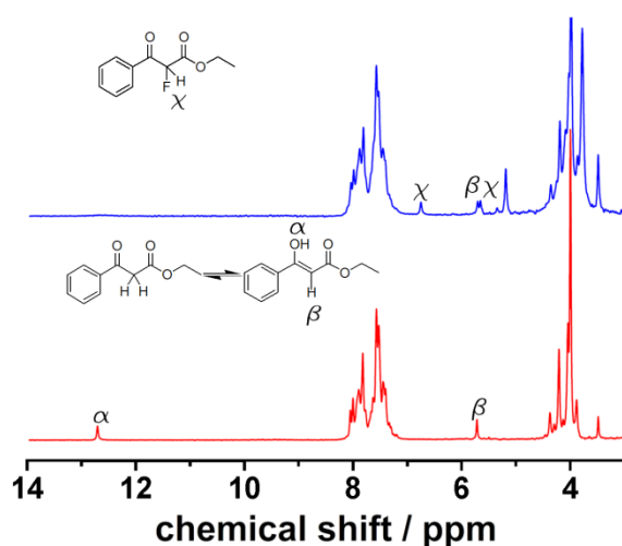
Fig. 4 Results of monitoring of a tautomerisation reaction employing Flow-NMR. Red: tautomeric equilibrium of the starting solution monitored employing Flow ^1\text{H} NMR. Blue: ^1\text{H} NMR spectrum after mixing 4 with Selectfluor under flow conditions.
