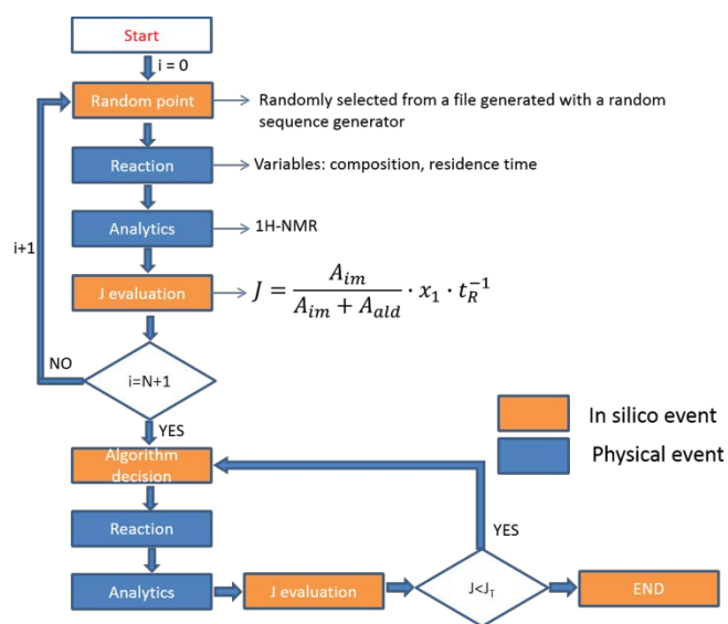
Figure 7 Self-optimization reaction of an imine synthesis under flow employing in-line NMR to feedback the signal.
