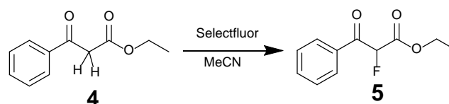
Scheme 3 Synthesis of ethyl-2-fluoro-3-oxo-3-phenylpropanoate with Selectfluor.
