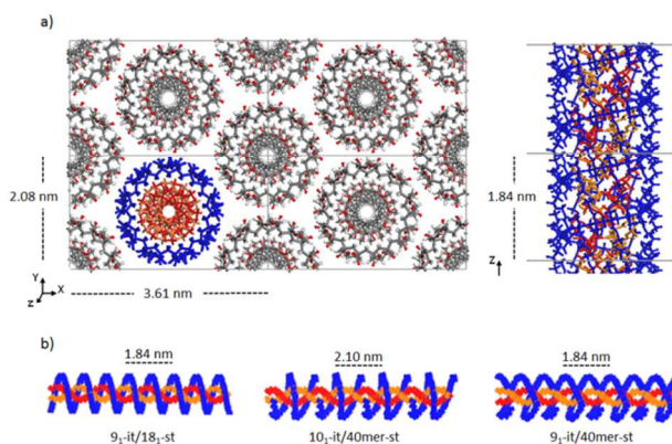
Figure 2. a) Initial model crystal structure of the 9_1 - it -/ 18_1 - st -PMMA stereocomplex, b) schematic representations of the three triple helix stereocomplex systems.
