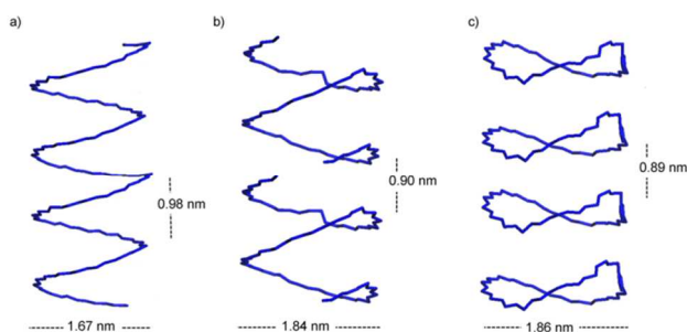
Figure 7. The syndiotactic helix backbone of the a) 9_1 - it /18 1 - st b) 9_1 - it /40mer- st and c) 9_1 - it /cyclic-18mer- st stereocomplex models. The it -PMMA double helix is not shown. The larger diameter of the 9_1 - it /40mer- st and distinct helical curvature of this model enable the fit to the experimental X-ray diffraction peaks at 2.08 nm and 0.78 nm, respectively.
