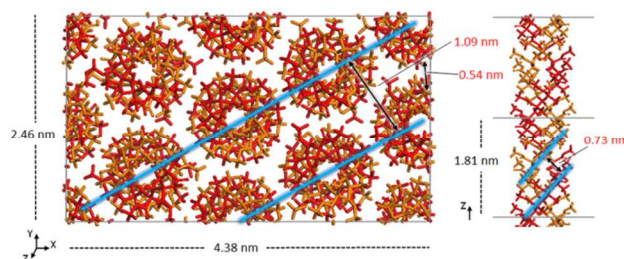
Figure 4. Model of the optimized crystal structure of 9_1 it -PMMA in the Right Down packing motif. The chain-chain spacing (left) and pitch spacing (right) are shown in light blue.
