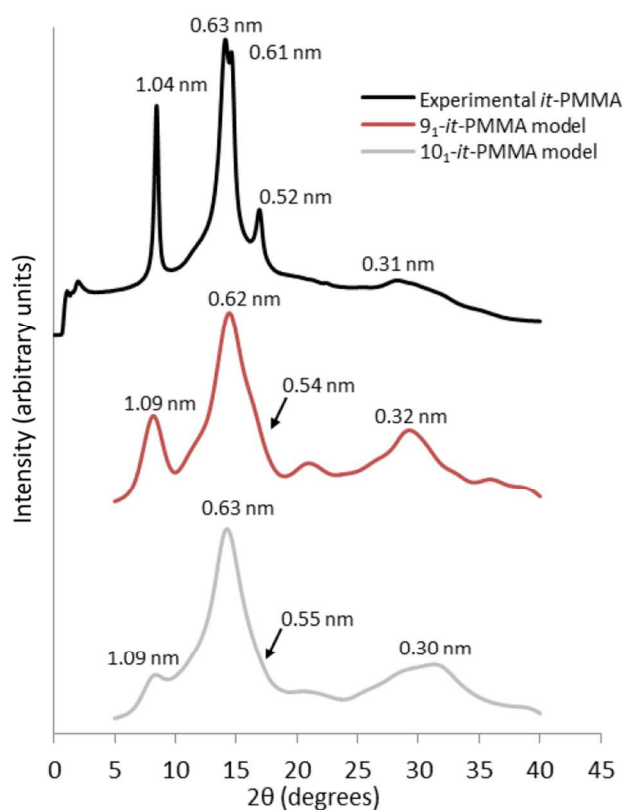
Figure 3. Wide angle X-ray scattering profiles obtained from powder diffraction experiments and molecular dynamics simulations for the it -PMMA double helix in the Right Down packing motif.
