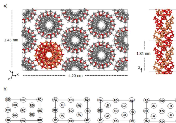
Figure 1. a) Initial model crystal structure of 9_1 it -PMMA, b) the four packing motifs examined in this study (from left to right): Right Down (RD), Right Down/Right Up (RD/RU), Right Down/Left Down (RD/LD), and Right Down/Left Up (RD/LU).
