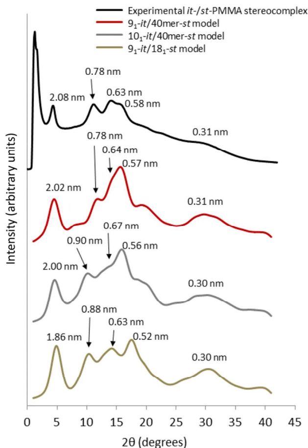
Figure 5. Wide angle X-ray scattering data obtained from powder diffraction experiments and molecular dynamic simulation for the it - st -PMMA stereocomplex in the Right Down packing motif.
