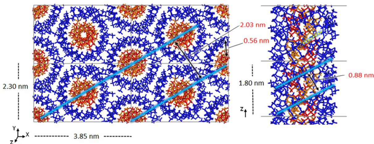
Figure 6. Optimized crystal structure model of 9_1 - it -/40mer- st -PMMA in the Right Down packing motif. The chain-chain spacing (left) and pitch spacing (right) are shown in light blue. The gap between 40-unit st -PMMA fragments is shown by a dotted yellow line.
