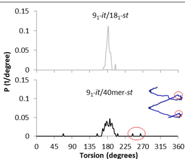
Figure 8. Backbone torsion distribution of the st -PMMA in the it - st -PMMA stereocomplex models. The 9_1 - it /18 1 - st model represents an ideal helix, while the 9_1 - it /40mer- st model exhibits non-ideal helical geometry. The torsions associated with this non-ideal helical geometry are circled in red.
