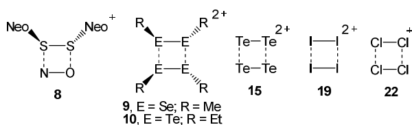
Scheme 2 \pi^* - \pi^* -Bonded four-membered rings.
