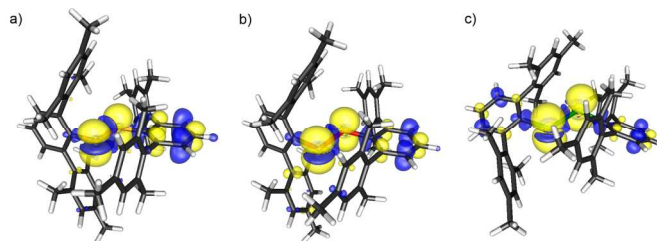
Figure 4 Calculated spin densities for 17a-c at contour levels of 0.0025 (yellow) and -0.0005 (blue). Note the small but noticeable negative spin density on the para-H atom of one terphenyl ring for 17a and 17b .
