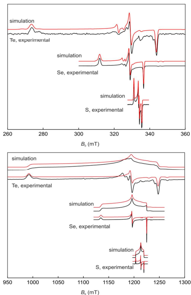
Figure 3 Field-sweep EPR spectra for 17a (E = S) 17b (E = Se) and 17c (E = Te) measured in frozen \text{CH}_2\text{Cl}_2/\text{THF} solution (1:1), along with the corresponding simulations.
