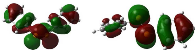
Figure 2 HOMO (left) of C_2 symmetric (C_6F_5Se)_2 ( 13b ) and SOMO (right) of C_2 symmetric [(C_6F_5Se)_2]^{+\bullet} ( 14b ).
