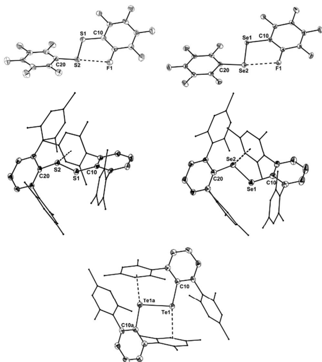
Figure 1 Molecular structures of the radical cations 14a,b and 17a-c ; thermal ellipsoids are set at 30% probability.
