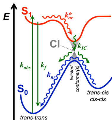
Scheme 2. Generalized photoinduced dynamics of THIA and other cyanine dyes.
