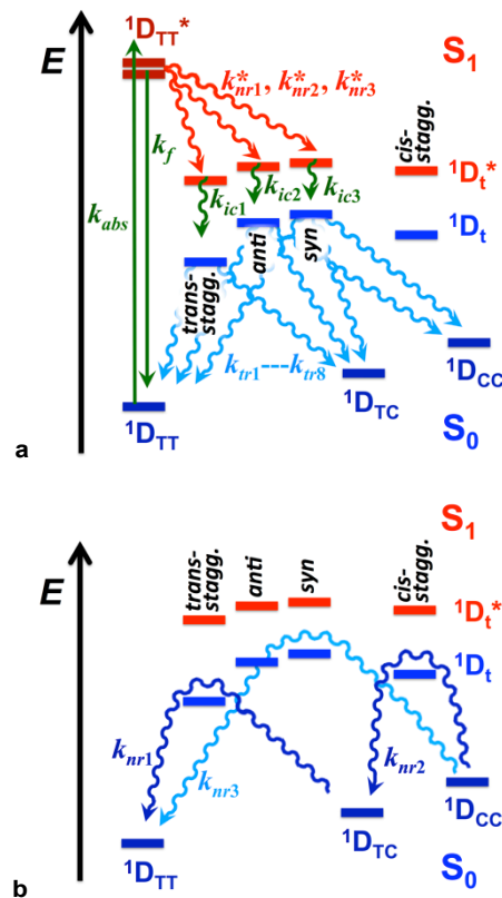
Scheme 3. Multiple paths of relaxation of THIA.
