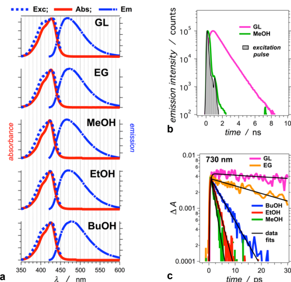
Figure 1. Photophysical properties of THIA in: glycerol (GL), ethylene glycol (EG), methanol (MeOH), ethanol (EtOH), and 1-butanol (BuOH). (a) Normalized steady-state spectra: absorption (Abs), emission (Em, \lambda_{\text{ex}} = 400 nm), and excitation (Exc, \lambda_{\text{em}} = 470 nm). (b) Emission decays for glycerol and methanol recorded using TCSPC ( \lambda_{\text{ex}} = 406 nm, \lambda_{\text{em}} = 475 nm, half-height pulse width, PW = 195 ps). (c) Transient-absorption decays of THIA in the five alcohols, recorded at 730 nm. This transient corresponds to the excited-state conformer that undergoes radiative deactivation ( \lambda_{\text{ex}} = 385 nm; PW 800nm = 50 fs, 2 \mu\text{J}/\text{pulse} ).
