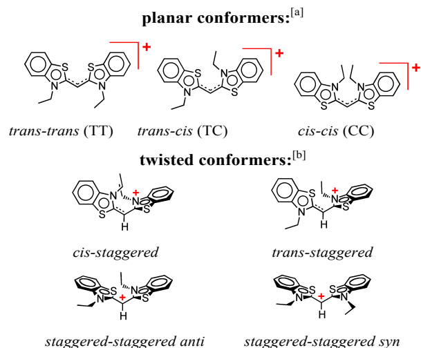
Scheme 1. Conformers of 3,3'-Diethylthiacyanine (THIA).
