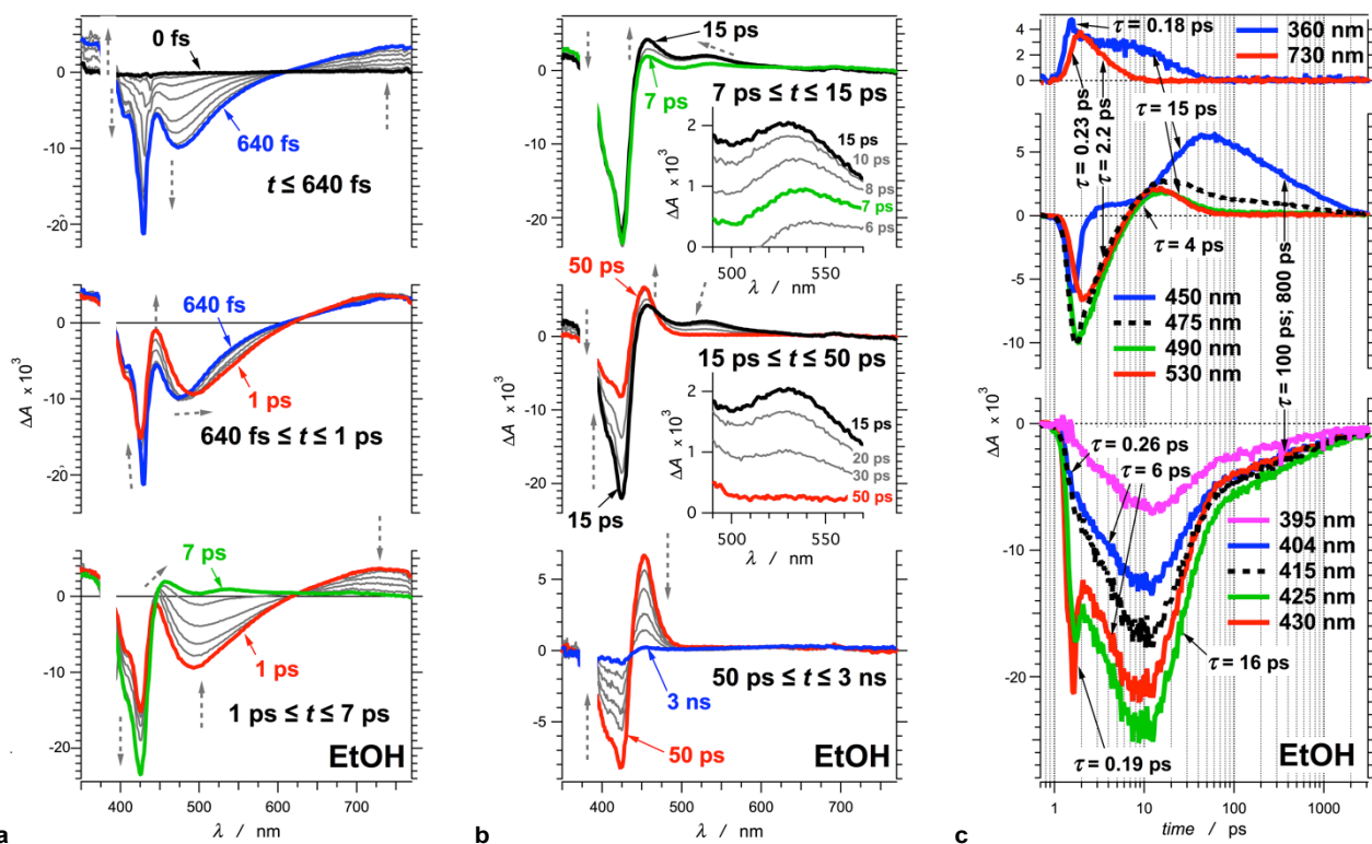
Figure 2. Transient absorption of THIA (10 \mu\text{M} in ethanol). (a) Chirp-corrected transient-absorption spectra in the subpicosecond and picosecond time domains. (b) Transient-absorption spectra in the picosecond and nanosecond time domains. (insets) Expanded spectral region around 530 nm, showing the band that was ascribed to the twisted conformers of the singlet excited state. The grey dashed arrows indicate the changes in \Delta A (vertical direction) and the shifts of the spectral maxima and minima (horizontal direction). (c) Transient-absorption kinetics recorded at different wavelengths. The logarithmic abscissa allows for presenting the various time domains on the same graph. The pump time, i.e., t_0 , was set at 1 ps. ( \lambda_{\text{ex}} = 385 \text{ nm} ; \text{PW}_{800\text{nm}} = 50 \text{ fs} , 2 \mu\text{J/pulse} ).
