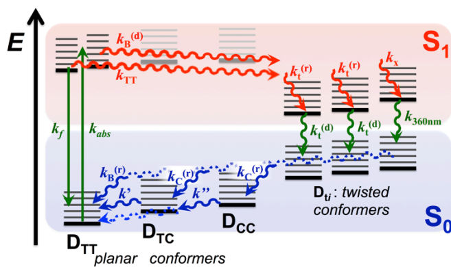
Scheme 3. Excited- and ground-state dynamics of THIA as determined from transient-absorption kinetics.
