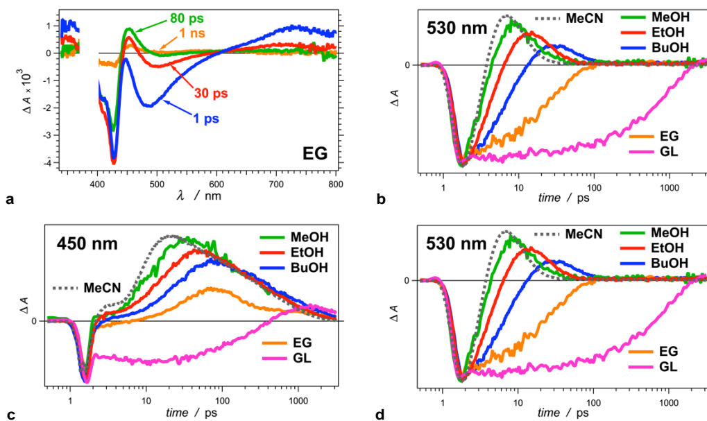
Figure 3. Solvent dependence of the transient-absorption kinetics of THIA (10 \mu\text{M} ). (a) Chirp-corrected transient-absorption spectra for a relatively viscous solvent, ethylene glycol (EG). (b) Transient-absorption kinetics recorded at 530 nm (showing the rise and the decay of the twisted conformers) for alcohols with different polarity and viscosity (Table 1): methanol (MeOH), ethanol (EtOH), 1-butanol (BuOH), ethylene glycol (EG) and glycerol (GL), as well as for a non-viscous aprotic solvent, acetonitrile (MeCN). (c) Transient-absorption kinetics of THIA recorded at 450 nm (showing the formation and the decay of the ground-state trans-cis and cis-cis conformers) for different alcohols and for MeCN. (d) Transient-absorption kinetics of THIA recorded at peak (i.e., minimum) of the bleach band (corresponding to the ground-state trans-trans conformers) for different alcohols and for MeCN. The logarithmic abscissa of the kinetic data allows for presenting the various time domains on the same graph. The pump time, i.e., t_0 , was set at 1 ps. ( \lambda_{\text{ex}} = 385 \text{ nm} ; \text{PW}_{800\text{nm}} = 50 \text{ fs} , 2 \mu\text{J/pulse} ).
