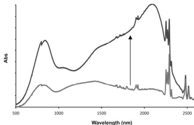
Figure 7. Low energy optical changes on addition of one equivalent of fluoride ion to electrochemically generated \mathbf{I}^{4+} after equilibration with one equivalent of fluoride guest. Solvent: 0.1 M TBAPF 6 in acetonitrile at 273 K
