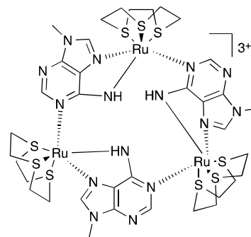
Figure 1. Structure of macrocycle 1 3+
