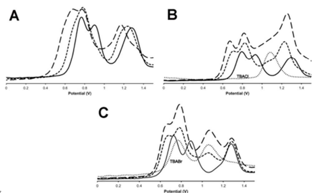
Figure 6. Square wave voltammograms, SWVs, for the oxidations of 1^{3+} on the addition of (A) TBAF; (B) TBACl; (C) TBABr. Key: (—) = untreated 1^{3+} , (---) = +1 equivalent of guest, (····) = +3 equivalents of guest. In (B) and (C) (····) = SWV of TBACl and TBABr respectively in identical conditions (Vs. Ag/AgCl Solvent: 0.1 M TBAPF _6 in acetonitrile)
