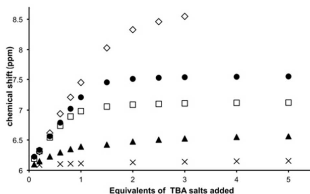
Figure 3. Changes in the chemical shifts of the 9MA-based NH6 proton of \mathbf{1}^{3+} (concentration of hexafluorophosphate salt: 1.75 mM \text{l}^{-1} of host dissolved in d^3 -MeCN) on addition of the following selected anions: \text{ClO}_4^- (x), \text{I}^- (▲), \text{Br}^- (□), \text{Cl}^- (●), and \text{F}^- (◇). The data for the fluoride titration is truncated as higher binding ratios lead to precipitation of the host.
