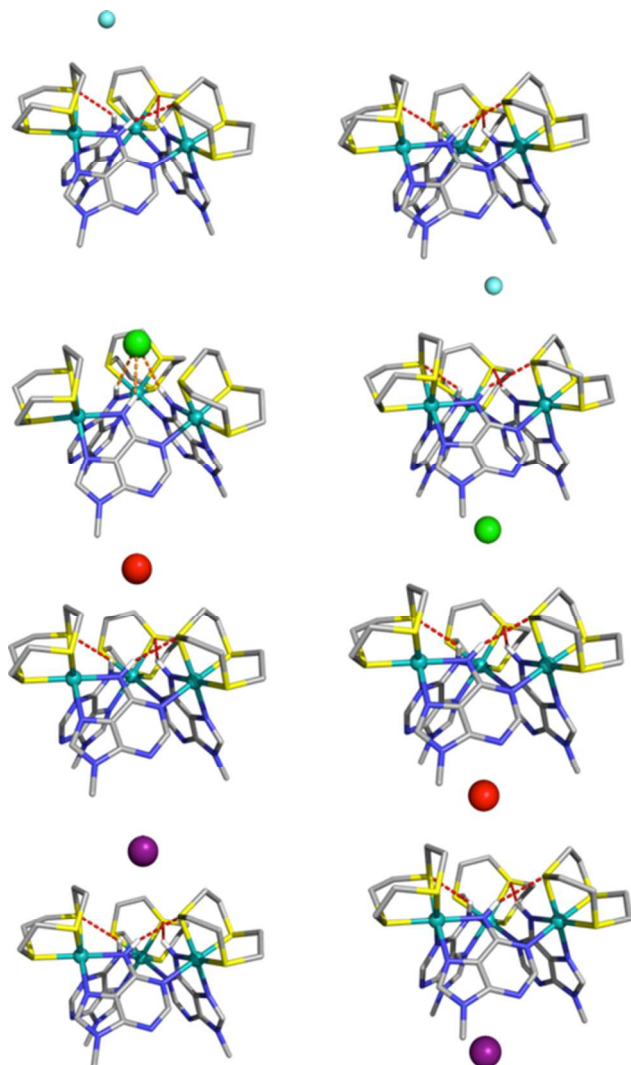
Figure 5. Optimized structures of 1^{3+} with F^- (cyan), Cl^- (green), Br^- (red), and I^- (purple) for binding in the \alpha pocket (left) or the \beta pocket (right). Binding scenario \beta is disfavoured relatively to \alpha by 3.8 ( F^- ), 1.9 ( Cl^- ), 2.5 ( Br^- ) and 2.2 ( I^- ) kcal mol ^{-1} respectively. The N-H...S and N-H...Cl ^- hydrogen bonds are drawn as red and orange dashed lines, respectively.
