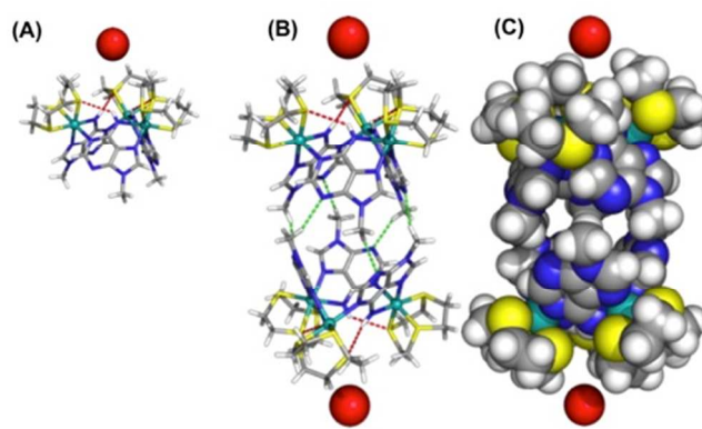
Figure 2. (A) Details from the single crystal X-ray structure of [\mathbf{1}](\text{Br})_3 showing the weak N–H...S hydrogen bonds (red dashed lines) within the of \mathbf{1}^{3+} unit. (B) Dimeric “capsules” formed in the structure through C–H...N hydrogen bonds (green dashed lines) between facing bowls. (C) CPK model of capsules showing axial entrances occupied by bromide anions and equatorial “gates” locked by the steric bulk of N-methyl groups of 9MA ligands. The following atomic colour scheme was used: carbons in grey, hydrogens in white, sulfurs in yellow, nitrogens in blue, ruthenium centres in teal and bromide anions in red
