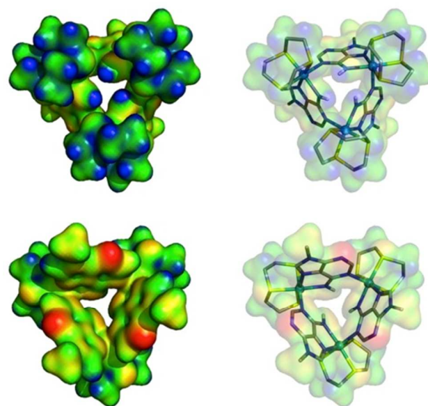
Figure 4. Electrostatic potential mapped on the molecular electron density surface (0.02 electrons/Bohr 3 ) for receptor \mathbf{1}^{3+} presented in two different views. Top: N-H binding site pointing to front. Bottom: 9-methyl adenine groups pointing to front. The color scale runs from 0.10 (red) to 0.48 (blue) atomic units.
