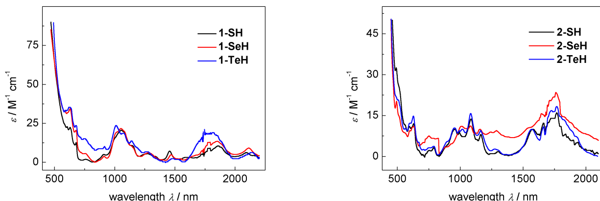
Fig. 3 Vis/NIR spectra of hydrochalcogenido complexes 1-SH (9.2 mM, black), 1-SeH (9.7 mM, red), and 1-TeH (4.1 mM, blue) recorded in DME at 25 °C (left) and vis/NIR spectra of hydrochalcogenido complexes 2-SH (2.0 mM, black), 2-SeH (6.6 mM, red), and 2-TeH (6.5 mM, blue) recorded in benzene at 25 °C (right). The molar absorption coefficients for complexes 2-EH were calculated per uranium center for a better comparison.
