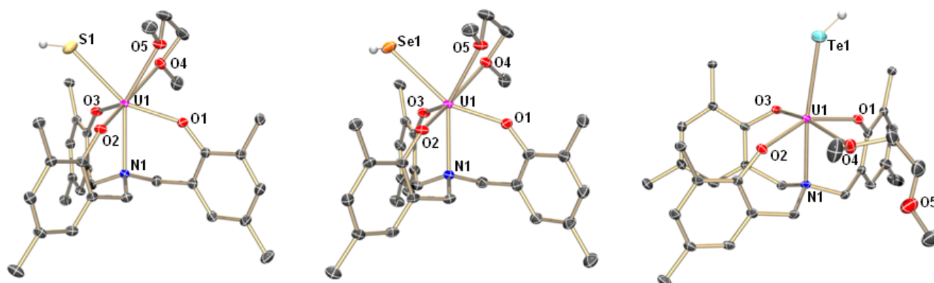
Fig. 1 Molecular structures of uranium hydrosulfide complex 1-SH (left), uranium hydroselenide complex 1-SeH (center), and uranium hydrotelluride complex 1-TeH (right). The chalcogen-bound H atoms in 1-SH and 1-TeH could be located on the difference Fourier map, the proton in 1-SeH was placed in a position of optimized geometry. All other H atoms, the adamantyl groups, and co-crystallized solvent molecules are omitted for clarity. Thermal ellipsoids are at 50% probability.
