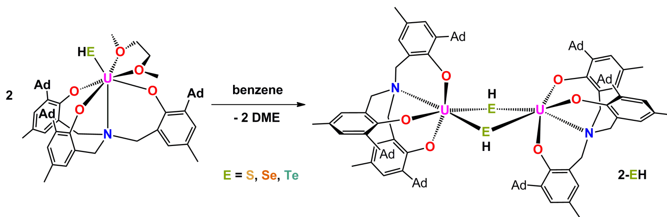
Scheme 2 Synthesis of dinuclear hydrochalcogenide complexes 2-EH (E = S, Se, Te).
