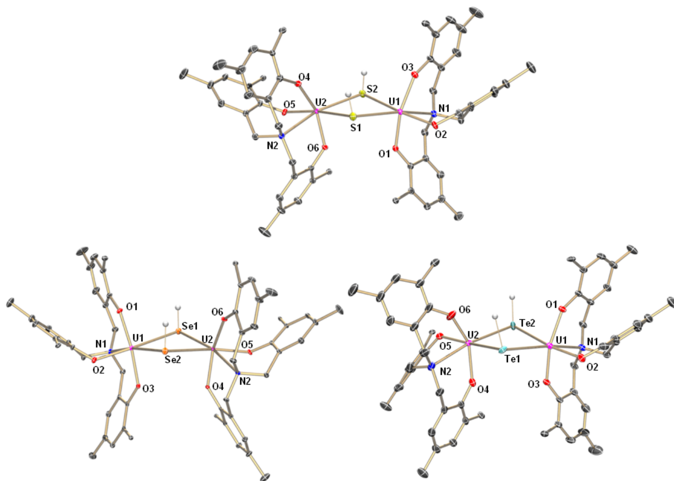
Fig. 2 Molecular structures of uranium hydrosulfide complex 2-SH (top), uranium hydroselenide complex 2-SeH (bottom left), and uranium hydrotelluride complex 2-TeH (bottom right). The chalcogen-bound H atoms in 2-SH and 2-TeH could be located on the difference Fourier map, the protons in 2-SeH were placed in a position of optimized geometry. All other H atoms, the adamantyl groups and co-crystallized solvent molecules are omitted for clarity. Thermal ellipsoids are at 50% probability.
