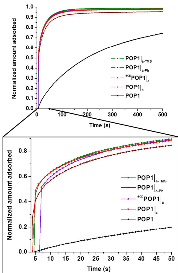
Figure 6. Time-dependent propane uptake profiles for \text{POP1} , \text{POP1}_{|\text{a}} , ^{\text{scp}}\text{POP1}_{|\text{a}} , \text{POP1}_{|\text{a-TMS}} , and \text{POP1}_{|\text{a-Ph}} at 0.3 bar and 298 K. Data in each profile were normalized to the maximum uptake values at 15000 s (see complete set of data in Figure S13 in the ESI†).
