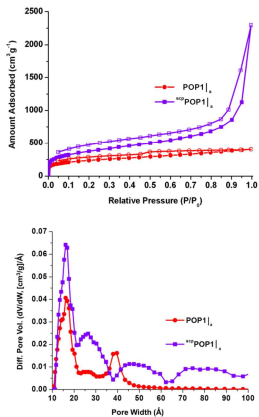
Figure 5. (Top) \text{N}_2 isotherms measured at 77 K of \text{POP1}|_{\text{a}} (red circles) and supercritical \text{CO}_2 -processed POP-A ( ^{\text{scp}}\text{POP1}|_{\text{a}} – purple squares). Closed symbols, adsorption; open symbols, desorption. (Bottom) Pore size distributions based on DFT calculations (slit-pore model) for \text{POP1}|_{\text{a}} (red circles) and ^{\text{scp}}\text{POP1}|_{\text{a}} (purple squares). See ESI† for the isotherms (Figure S6) and pore size distributions (Figure S7) of other supercritical \text{CO}_2 -processed POPs.
