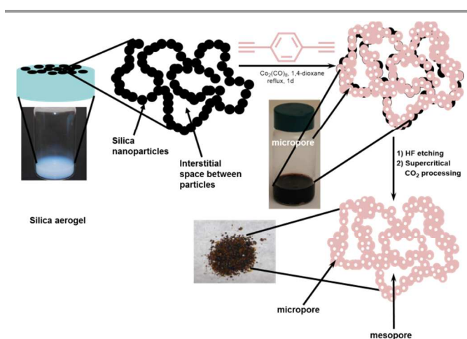
Figure 1. An illustration of the synthesis of a POP possessing a hierarchy of pores. From left to right: a silica aerogel template is infiltrated with a solution of the monomer and catalyst. After polymerization, HF etching and supercritical CO 2 processing of the resulting monolith afford the desired POP as a powder. In this scheme, the interstitial spaces between the silica nanoparticles that made up the monolithic aerogel template are responsible for the formation of mesopores.
