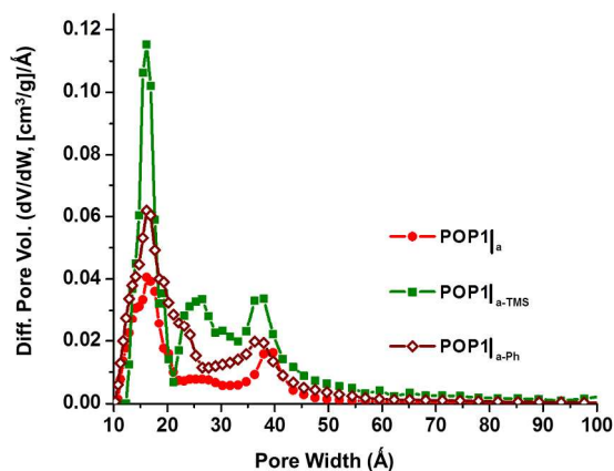
Figure 4. Pore size distributions based on DFT calculations (slit-pore model) for \text{POP1}|_{\text{a}} (red circles), \text{POP1}|_{\text{a-TMS}} (green squares) and \text{POP1}|_{\text{a-Ph}} (brown diamonds).
