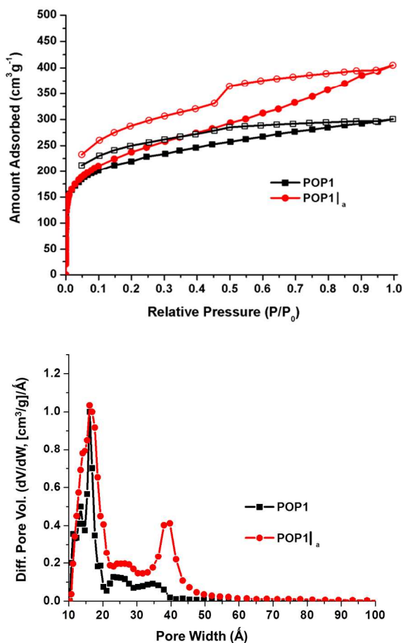
Figure 2. (Top) N 2 isotherms measured at 77 K of POP1 (black squares) and POP1 a (red circles). Closed symbols, adsorption; open symbols, desorption. (Bottom) Pore size distributions based on DFT calculations (slit-pore model) for POP1 a (red circles) and POP1 without template (black squares).
