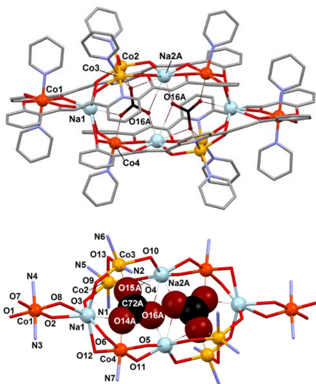
Figure 5. (top) Representation of the cation of [\text{Co}_8\text{Na}_4(\text{L})_4(\text{OH})_2(\text{CO}_3)_2(\text{py})_{10}](\text{BF}_4)_2 ( 2 ), with unique metals and closest O atoms from \text{CO}_3^{2-} labelled. Color code: grey, C; red, O; purple, N; orange, Co(II); dark orange, Co(III); blue, Na; \text{CO}_3^{2-} emphasized in dark red and black. Hydrogen atoms not shown. Only one position of disordered species shown. (bottom) Core of complex 2 with unique atoms labelled. The closest positions of the encapsulated \text{CO}_3^{2-} ions, of the two disordered locations resolved are shown and emphasized in space filling format.
