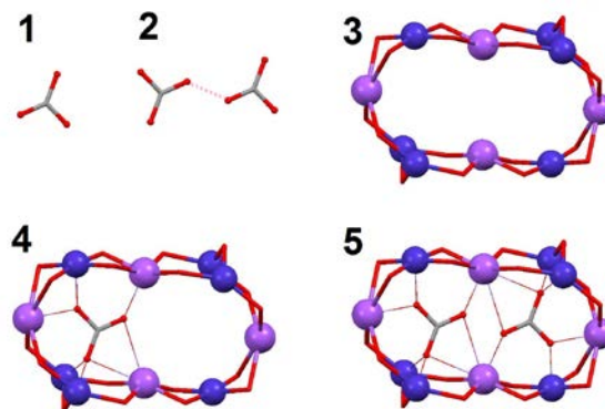
Figure 6. Simplified scheme of the models used for DFT calculations: ‘1’, a free \text{CO}_3^{2-} anion ( E_1 ); ‘2’, a dimer of two \text{CO}_3^{2-} anions ( E_2 ); ‘3’, the full cluster anion of 2 without the \text{CO}_3^{2-} ligands ( E_3 ); ‘4’, the entire cluster anion of 2 with only one \text{CO}_3^{2-} ligand ( E_4 ); ‘5’, the cluster of 2 with both encapsulated \text{CO}_3^{2-} groups ( E_5 ). All species have been calculated in the gas phase and their energies obtained at the B3LYP-D2/SVP level.
