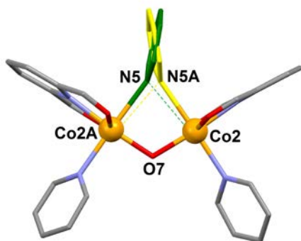
Figure 4. Representation of the central core of [\text{Co}_4(\text{L})_2(\text{OH})(\text{py})_7]\text{NO}_3 ( 1 ) emphasizing the two positions of the disordered \mu -pyridine group (yellow and green).
