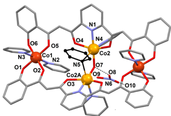
Figure 3. Molecular structure of [\text{Co}_4(\text{L})_2(\text{OH})(\text{py})_7]\text{NO}_3 ( 1 ) with crystallographically unique heteroatoms labelled. Carbon atoms are in grey except these of the central \mu -pyridine group, which has been emphasized in black. Hydrogen atoms not shown. Only one of two disordered positions of \text{NO}_3^- and \mu -pyridine are shown.
