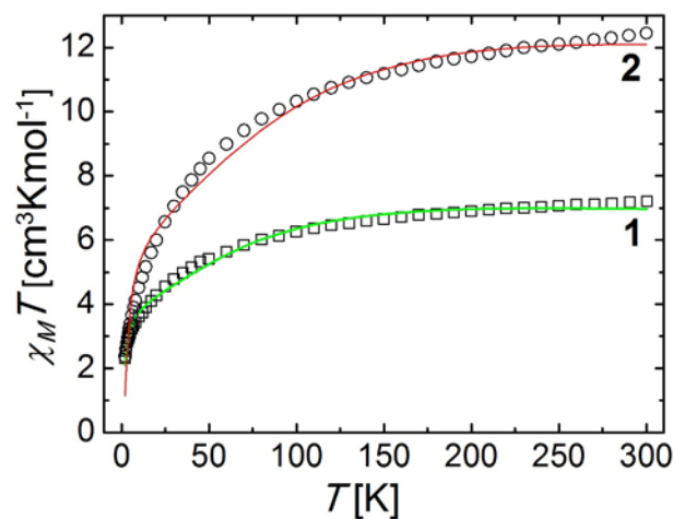
Figure 7. Plots of \chi_M T vs T for complexes 1 and 2 . The solid lines are best fits to the experimental data (see text for details).
