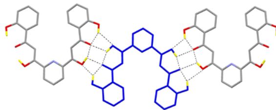
Figure 2. Representation of three molecules of H 4 L emphasizing the various three-center hydrogen bonding interactions established between them.
