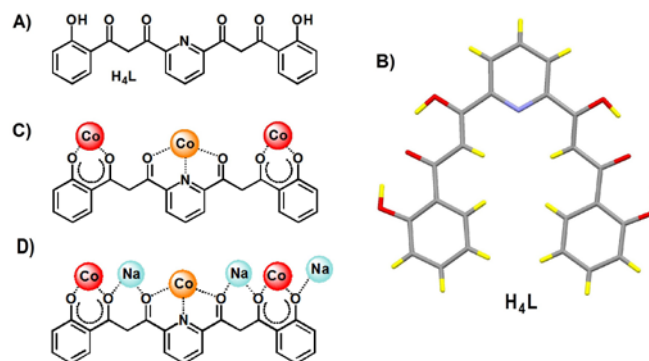
Figure 1. Bis-dicarbonyl form of ligand H 4 L (A), solid state molecular structure of H 4 L (C, grey; O, red; N, purple; H, yellow) showing its fully enolic form (B), and coordination modes featured by H 4 L in compounds 1 and 2 (C).
