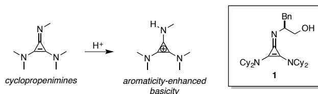
Figure 1. Enantioselective Brønsted base catalysis with cyclopropenimine 1 .
