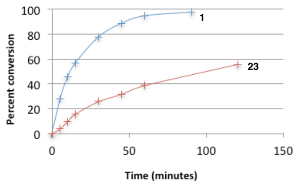
Chart 1. Conversion rates of catalysts 1 and 23 .
