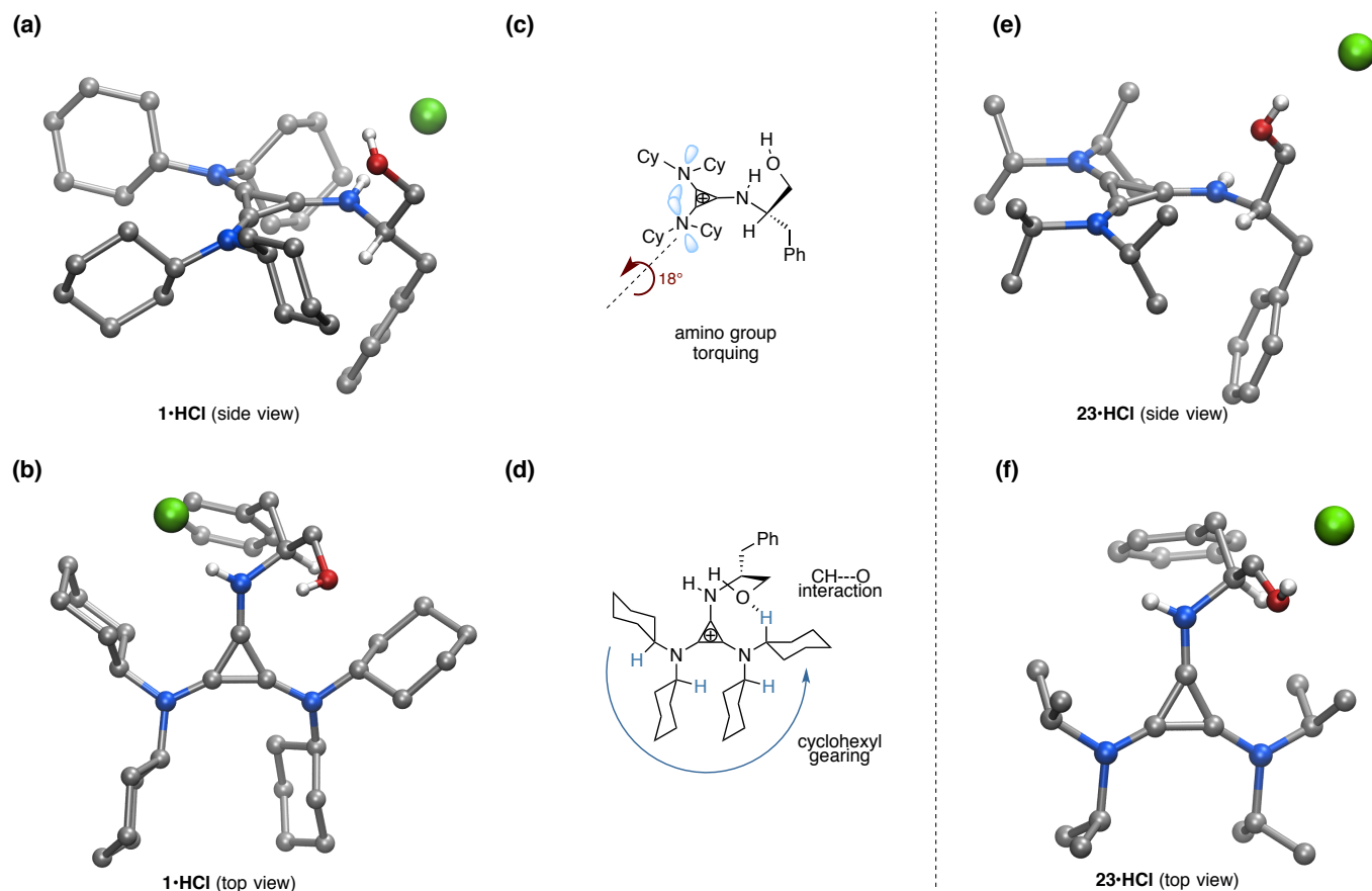
Figure 4. Molecular structure of (a) 1 •HCl side view; (b) 1 •HCl top view; (c) Depiction of amino group torquing phenomenon of 1 •HCl; (d) Depiction of cyclohexyl gearing effect and key CH...O interaction of 1 •HCl; (e) 23 •HCl side view; and (f) 23 •HCl top view. For (a) and (b) a co-crystallized molecule of H 2 O has been omitted for clarity. For (e) and (f) the hydroxymethyl group was disordered and only one of the crystal forms is shown for clarity. A molecule of co-crystallized benzene was also removed for 23 •HCl. The unmodified structures are included in the supporting information file.
