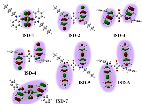
Figure 3. The natural transition orbitals for the “hole” in second excited state ( S_2 ) of seven ISD molecules.
