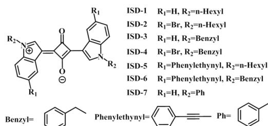
Figure 1. Structures and numbering scheme for ISD compounds studied in this paper.
