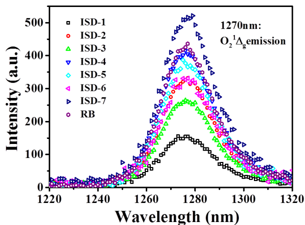
Figure 7. Luminescence of singlet oxygen sensitized with seven ISD dyes and Rose Bengal as reference.
