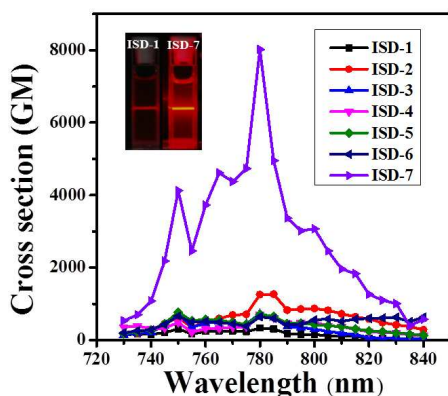
Figure 5. (a) TPA cross-section of ISDs in THF solutions. The inset shows the corresponding TPA fluorescence photographs of the ISD-1 (left) solution and the ISD-7 (right) solution under 780 nm illumination.
