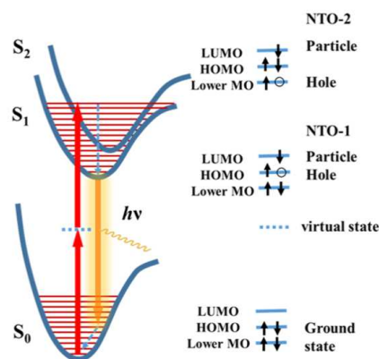
Figure 2. Energy level diagrams for the essential states for centrosymmetric chromophores in TPA process and the schematic diagram for the electron transition between energy level. Lower MO presents not only HOMO-1 orbital.
