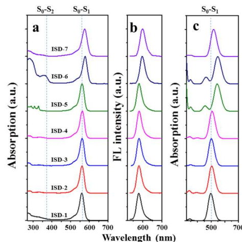
Figure 4. (a) Steady-state one-photon absorption and (b) fluorescence of ISD molecules in THF, and (c) the simulated absorption spectra.
