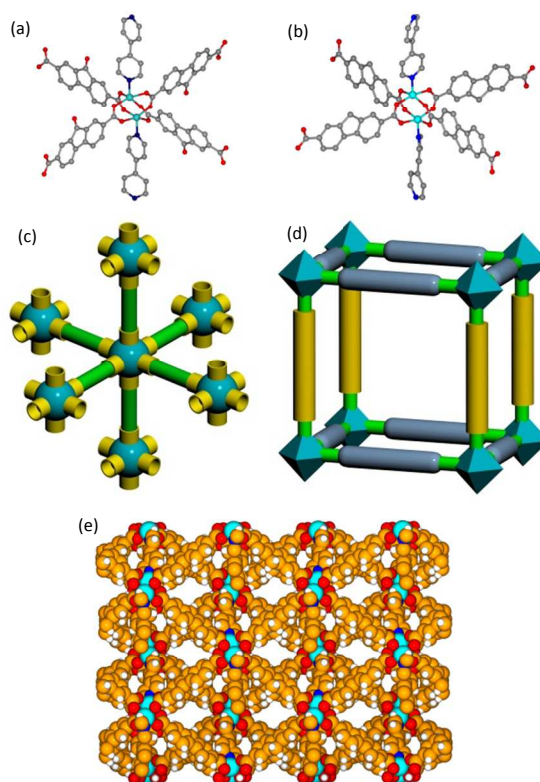
Figure 1. SBU of (a) LMOF-201 and (b) LMOF-202; (c) Illustrations of the connectivity of ligands (green) to the Zn core (aqua) and (d) a single cage of the framework; (e) The overall 3D structure of LMOF-202 viewing along the a axis. Colour code: White (H), Orange (C), Blue (N), Red (O), Aqua (Zn).
