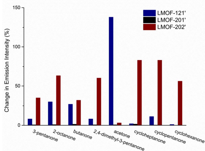
Figure 2. A comparison of fluorescence enhancement after 10 s exposure of LMOF-121' and LMOF-202' to the vapors of ketones.
