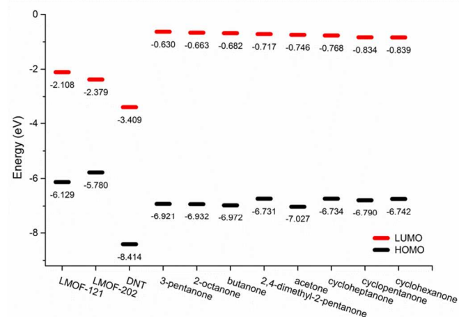
Figure 4. An illustration of molecular orbital energy levels of LMOF-121, LMOF-202, and analytes computed at B3LYP/SDD (on Zn), 6-31+G*(on H, C, N, O). 41
