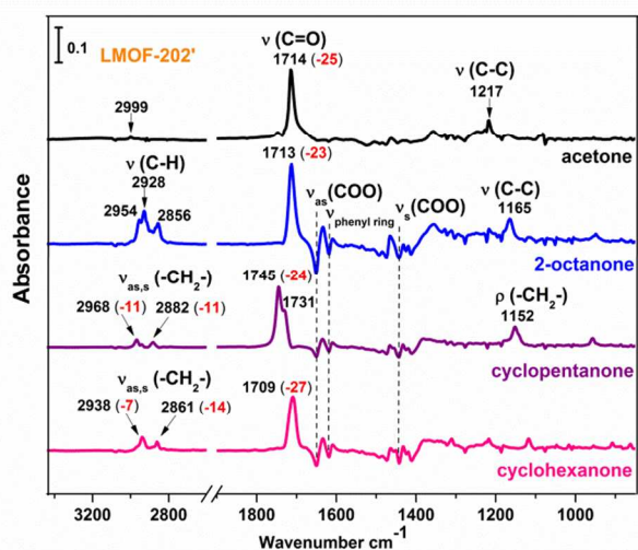
Figure 5. IR absorption spectra of adsorbed ketone molecules: acetone, 2-octanone, cyclopentanone, cyclohexanone in LMOF-202' referenced to IR spectrum of blank LMOF-202'. The spectra were recorded after exposing LMOF samples to vapors for 3 min.
