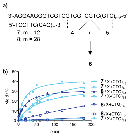
Figure 3: a) Principle of native chemical PNA ligation aided by partial DNA blockers 7 and 8 and b) time course of the product formation triggered by DNA templates varying in triplet repeats length for reaction systems involving 7 or 8 . Conditions: 1 \mu M reactive PNA probes in buffer (10 mM NaH 2 PO 4 , 150 mM NaCl, 10 mM MesNa, pH 7.5), 100 nM DNA template, 100 nM partial blocker, R = (CH 2 ) 2 SO 3 H.
