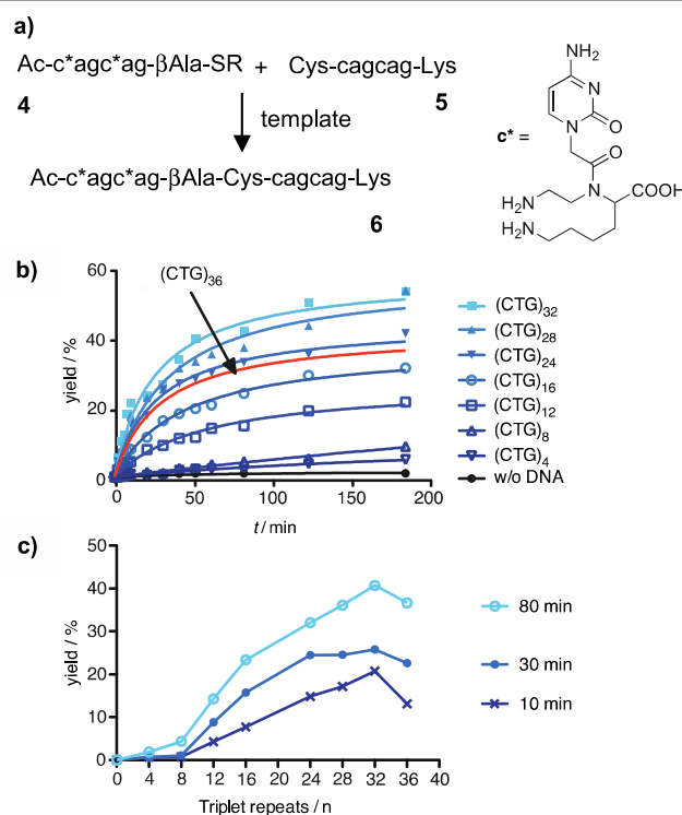
Figure 2: a) Native chemical ligation reaction between aminomodified PNA probes 4 and 5 ; b) time course of product 6 formed in absence or presence of 100 nM DNA templates varying in the number of triplet repeats; c) template dependence of yields obtained after 10 min, 30 min or 80 min. (Conditions: see Figure 1, R = (CH 2 ) 2 SO 3 H).
