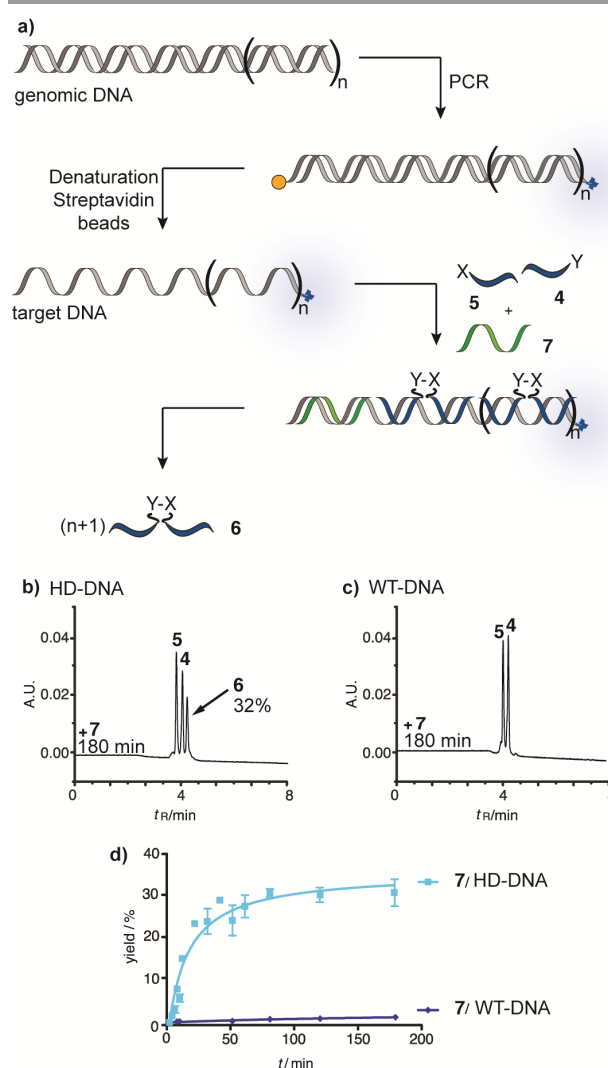
Figure 4: a) Principle of native chemical PNA ligation on templates obtained via PCR from human genomic DNA. UPLC traces (b, c) and time course (d) of reactions performed on DNA from b) a Chorea Huntington patient (HD-DNA) or c) a healthy individual (WT-DNA). Conditions: see Figure 3.
