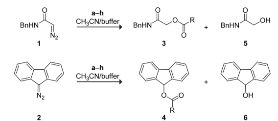
Scheme 2 Chemoselective esterification in an aqueous environment
