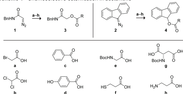
Scheme 1 Chemoselective esterification in acetonitrile
