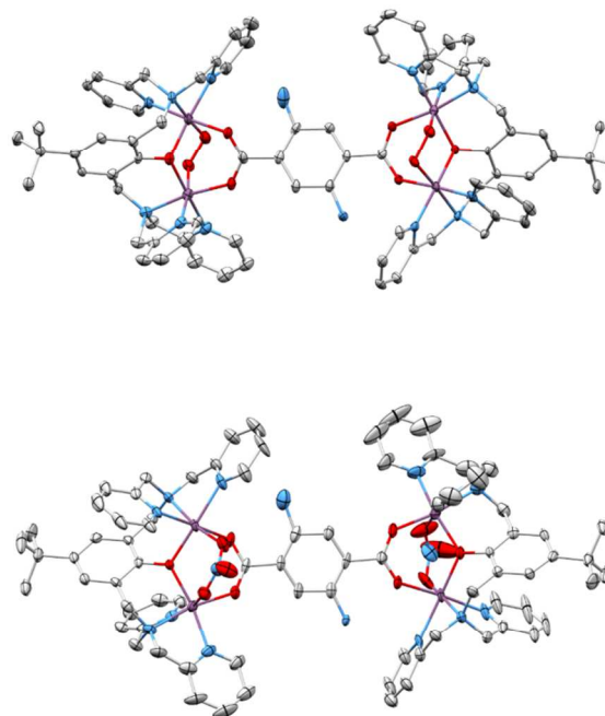
Figure 5. Molecular structure of the cations in (a) [\{(bpbp)Co_2(O_2)\}_2(NH_2bdc)](NO_3)_4 \cdot 7H_2O , 2b (NO 3 ) 4 ·7H 2 O, (b) [\{(bpbp)Co_2(NO_3)\}_2(NH_2bdc)](NO_3)_2 \cdot 2H_2O , 2b deoxy (NO 3 ) 2 ·2H 2 O. Two amine nitrogen atoms are shown on the 2-aminoterephthalato linker due to 45 50% occupancy in both positions. Hydrogen atoms omitted for clarity. Anisotropic displacement parameters drawn at the 30% probability level.
