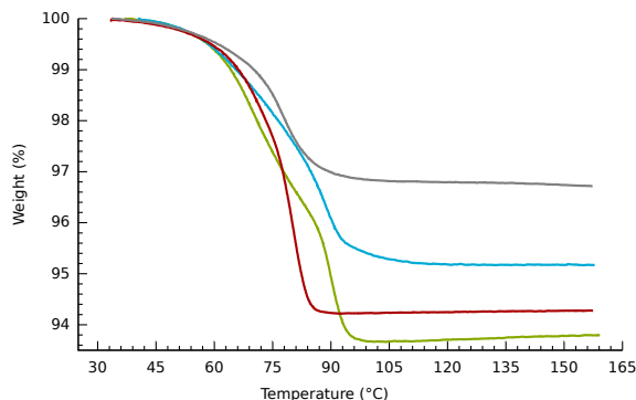
Figure 3. TGA comparison for [\{(bpbp)Co_2(O_2)_2\}_2(bdcR_4)](NO_3)_4 \cdot nH_2O , bdcR_4^{2-} = Cl_2bdc^{2-} (red, 2c ), bdc^{2-} (green, 2a ), NH_2bdc^{2-} (blue, 2b ) and F_4bdc^{2-} (grey, 2d ) showing temperature difference in deoxygenation and dehydration.
