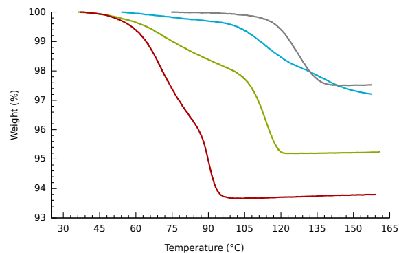
Figure 1. Thermogravimetric plot for NO 3 - (red), BF 4 - (green), PF 6 - (blue) and CF 3 SO 3 - (grey) salts of [ \{(\text{bpbp})\text{Co}_2(\text{O}_2)_2(\text{bdc})\}^{4+} ] ( 2a ) showing temperature dependent deoxygenation, accompanied by dehydration, see text.
