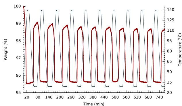
Figure 2. Temperature dependent cycling of reversible O 2 binding by 2a (BF 4 ) 4 measured using TGA.
