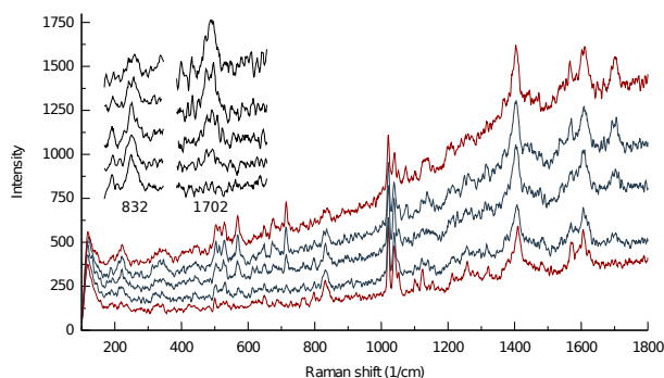
Figure 6. rRaman spectra from 100 to 1800 cm -1 following thermal deoxygenation of [(bpbp)Co 2 (O 2 ) 2 ](NH 2 bdc)](NO 3 ) 4 •7H 2 O, 2b (NO 3 ) 4 •7H 2 O at 20°C, 70°C, 90°C, 100°C and 120°C (from bottom to top).
