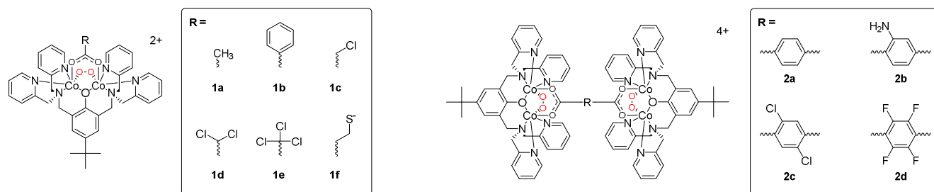
Scheme 1. Chemical structures of the cations in [(\text{bpbp})\text{Co}_2(\text{O}_2)(\text{O}_2\text{CR})](\text{A})_2 and [\{(\text{bpbp})\text{Co}_2(\text{O}_2)\}_2(\text{bdcR}_4)](\text{A})_4 .
