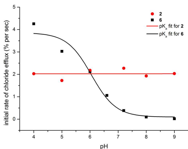
Fig. 7 pH dependence of the chloride transport ability of compounds 2 and 6 (1 mol% with respect to lipid). Chloride transport experiments were conducted as described in Figure 5 but at various different pHs. The obtained data was fitted to an asymptotic function and the initial rate of chloride efflux was calculated (see ESI† for details) and plotted as a function of pH. Apparent \text{pK}_a values could subsequently be estimated by fitting the obtained plot to the following sigmoidal function: y = \max + ((\min - \max)/(1 + 10^{(\text{pK}_a - x)})) .
