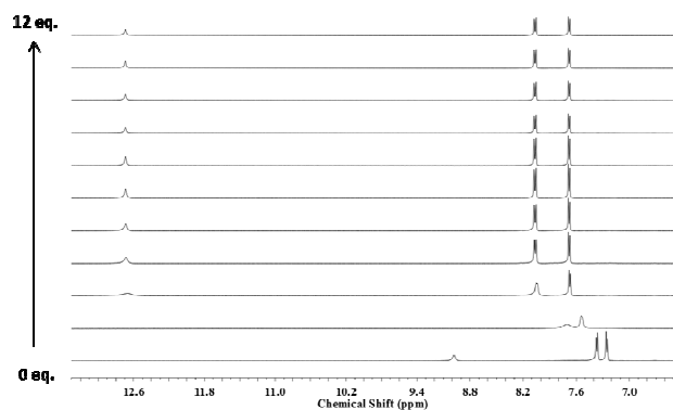
Fig. 2 Stack plot of the ^1\text{H} NMR spectrum of receptor 6 ( 2.5 \times 10^{-3} M) upon titration with chloride (0 – 12 eq.) added as its tetrabutylammonium salt in \text{CD}_3\text{CN} at 25^\circ\text{C} .
