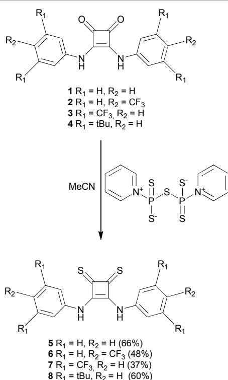
Scheme 1 Synthesis of thiosquaramide receptors 5–8 . Yields are given between brackets.
