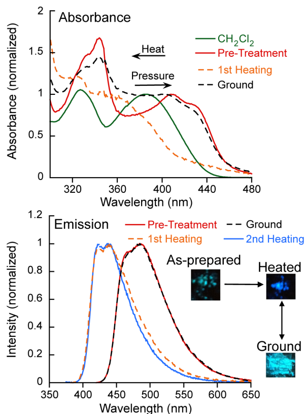
Figure 3: Absorbance (top) and emission (bottom) spectra of 7, drop cast from \text{CH}_2\text{Cl}_2 with heating and grinding cycles. Excitation wavelengths were 395 nm (green phase) and 350 nm (blue phase).
