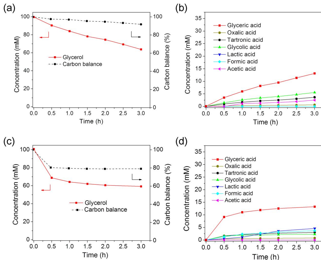
Figure 3. Glycerol oxidation using (a,b) Au/C and (c,d) Pd/C catalysts: (a,c) glycerol concentration and carbon balance, and (b,d) reaction products. Reaction conditions: 0.2 g Au/C or Pd/C, 60 °C, 1000 rpm stirring rate, 107 mL reaction volume, 0.1 M glycerol, 0.4 M NaOH, and 120 mL/min O 2 flow.
