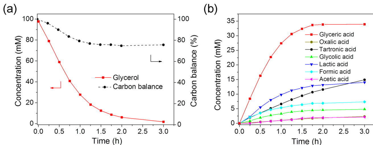
Figure 4. Reaction profile of glycerol oxidation reaction using 60 sc% Pd-on-Au/C catalyst (a) glycerol and carbon balance, and (b) reaction products. Reaction conditions: 0.2 g 60 sc% Pd-on-Au/C, 60 °C, 1000 rpm stirring rate, 107 mL, 0.1 M glycerol, 0.4 M NaOH, and 120 mL/min O 2 flow.
