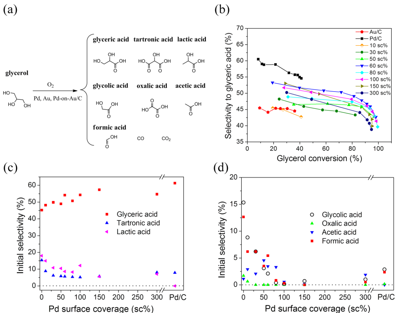
Figure 6. (a) Scheme of glycerol oxidation reaction and its products; Plots of (b) glyceric acid selectivity vs. glycerol conversion and (c,d) selectivity values extrapolated to zero conversion ("initial selectivity") for Au/C, Pd/C, and Pd-on-Au/C catalysts. Reaction conditions: 0.2 g catalyst, 60 °C, 1000 rpm stirring rate, 107 mL, 0.1 M glycerol, 0.4 M NaOH, and 120 mL/min O 2 flow.
