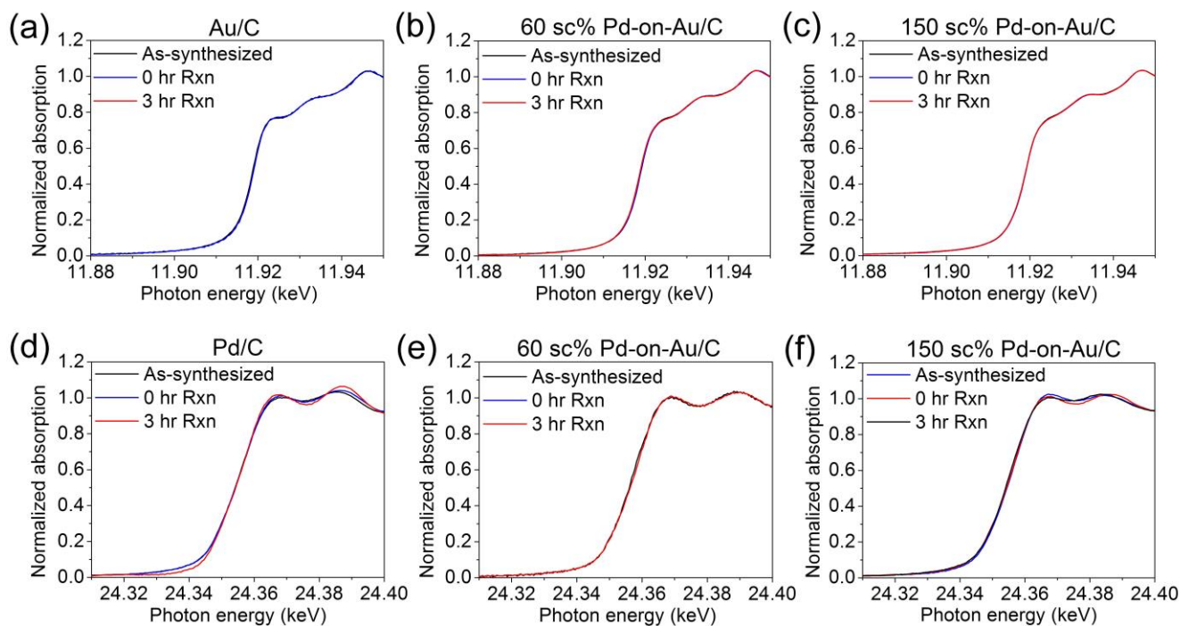
Figure 7. XANES spectra at the Au L III edge for (a) Au/C and Pd-on-Au/C with (b) 60 sc% and (c) 150 sc%; and at the Pd K edge for (d) Pd/C and Pd-on-Au/C with (e) 60 sc% and (f) 150 sc%.
