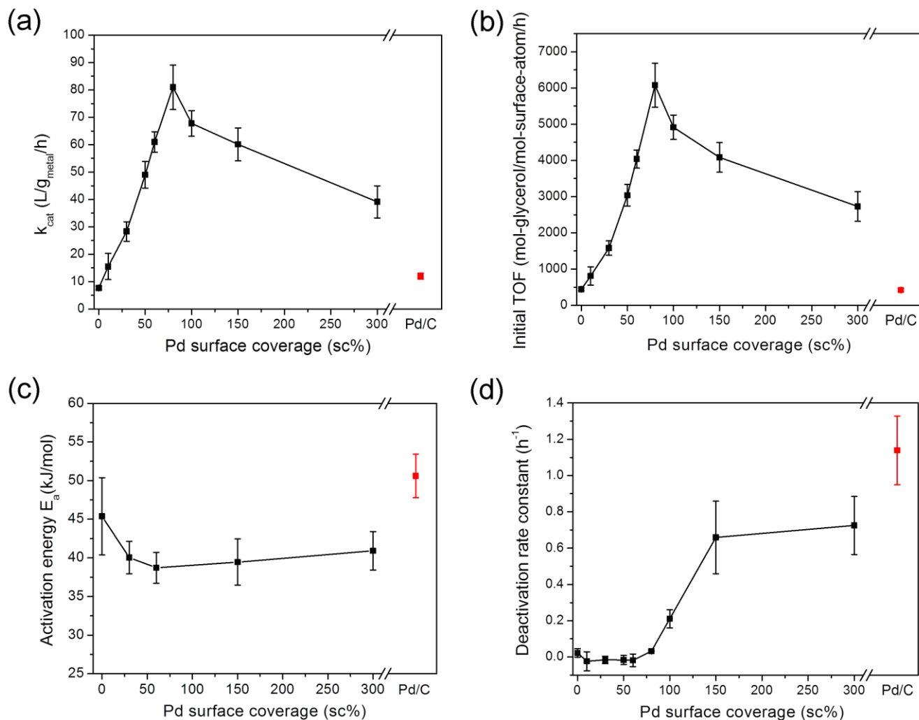
Figure 5. Plots of (a) k_{\text{cat}} (b) initial TOF, (c) apparent activation energy, and (d) deactivation constant values with Pd surface coverage. Reaction conditions for (a), (b), and (d): 0.2 g catalyst, 60 °C, 1000 rpm stirring rate, 107 mL, 0.1 M glycerol, 0.4 M NaOH, and 120 mL/min O 2 flow. Reaction temperature range for (c): 40-80 °C.
