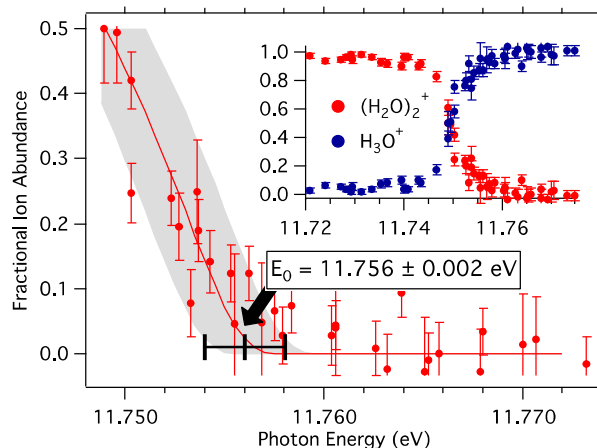
Fig. 3. Breakdown diagram for the dissociative photoionization of the water dimer: (H_2O)_2 + h\nu \rightarrow H_3O^+ + OH + e^- .
