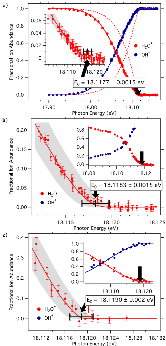
Fig. 2. iPEPICO breakdown curves corresponding to the H_2O \rightarrow OH^+ + H + e^- dissociative photoionization process, a) at room temperature, b) in molecular beam with 1 st order light, c) in molecular beam with 2 nd order light.
