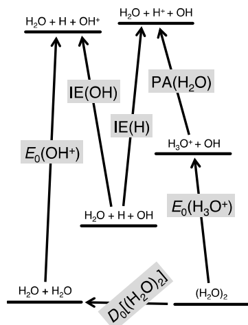
Fig. 1. Floating thermochemical cycle, not anchored to the standard scale of enthalpies of formation, used to derive the proton affinity of water. PA: proton affinity, IE: ionization energy, D_0 : 0 K neutral dissociation energy, E_0 : 0 K dissociative photoionization energy.
