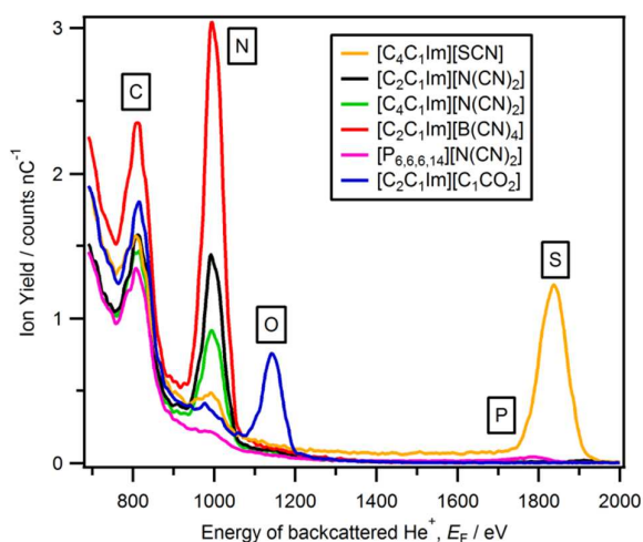
Figure 5. LEIS spectra ( ^4\text{He}^+ , E_0 = 3 keV) for which a nitrogen peak was observed ( [\text{C}_4\text{C}_1\text{Im}][\text{SCN}] , [\text{C}_2\text{C}_1\text{Im}][\text{N}(\text{CN})_2] , [\text{C}_4\text{C}_1\text{Im}][\text{N}(\text{CN})_2] , [\text{C}_2\text{C}_1\text{Im}][\text{B}(\text{CN})_4] , [\text{P}_{6,6,6,14}][\text{N}(\text{CN})_2] and [\text{C}_2\text{C}_1\text{Im}][\text{C}_1\text{CO}_2] ).
