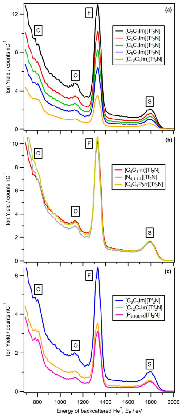
Figure 3. LEIS spectra ( ^4\text{He}^+ , E_0 = 3 keV) for: (a) [\text{C}_n\text{C}_1\text{Im}][\text{Tf}_2\text{N}] , (b) [\text{C}_4\text{C}_1\text{Im}][\text{Tf}_2\text{N}] , [\text{C}_4\text{C}_1\text{Pyrr}][\text{Tf}_2\text{N}] and [\text{N}_{4,1,1,1}][\text{Tf}_2\text{N}] , (c) [\text{C}_8\text{C}_1\text{Im}][\text{Tf}_2\text{N}] , [\text{C}_{12}\text{C}_1\text{Im}][\text{Tf}_2\text{N}] and [\text{P}_{6,6,6,14}][\text{Tf}_2\text{N}] .
