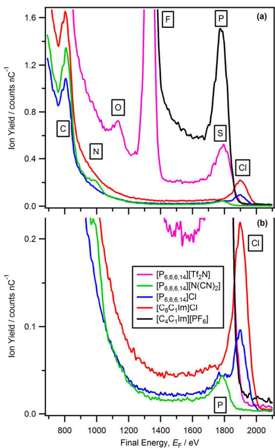
Figure 4. LEIS spectra ( ^4\text{He}^+ , E_0 = 3 keV) for phosphorus- and chlorine-containing ionic liquids ( [\text{P}_{6,6,6,14}][\text{N}(\text{CN})_2] , [\text{P}_{6,6,6,14}]\text{Cl} , [\text{C}_8\text{C}_1\text{Im}]\text{Cl} , [\text{C}_4\text{C}_1\text{Im}][\text{PF}_6] , [\text{P}_{6,6,6,14}][\text{Tf}_2\text{N}] ). (a) LEIS intensity scaled to show all P peaks, (b) LEIS intensity scaled to show all Cl peaks.
