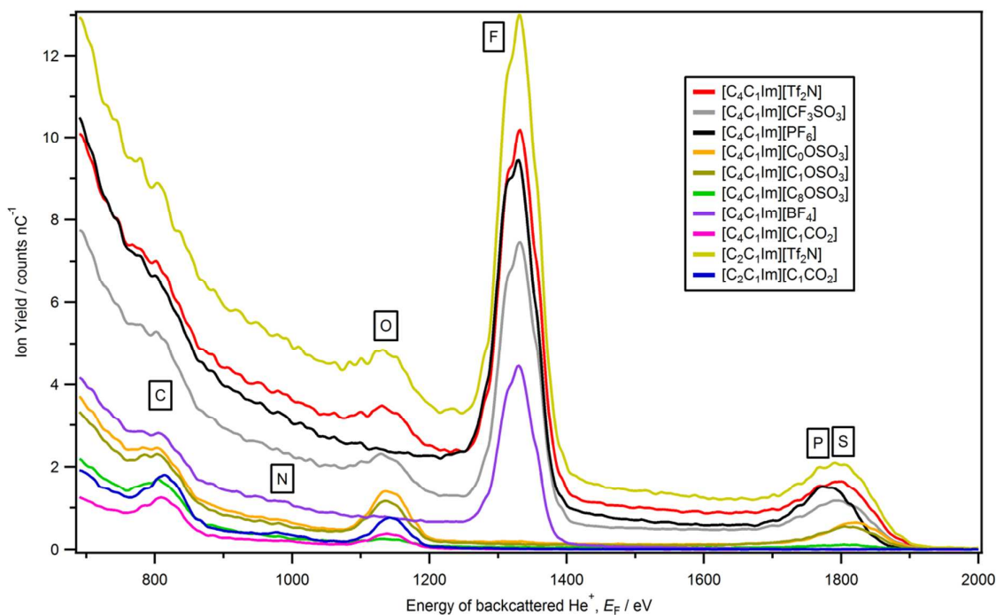
Figure 1. LEIS spectra ( {}^4\text{He}^+ , E_0 = 3 keV) for eight [\text{C}_4\text{C}_1\text{Im}][\text{A}] and two [\text{C}_2\text{C}_1\text{Im}][\text{A}] ionic liquids. Ionic liquids which contain cyano groups (e.g. [\text{C}_4\text{C}_1\text{Im}][\text{N}(\text{CN})_2] ) are not included in this plot (see Figure 5 for LEIS spectra of cyano-containing ionic liquids).
