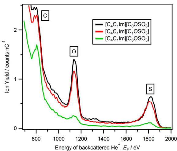
Figure 7. LEIS spectra ( ^4\text{He}^+ , E_0 = 3 keV) for [\text{C}_4\text{C}_1\text{Im}][\text{C}_n\text{OSO}_3] ionic liquids ( n = 0, 1, 8 ).
