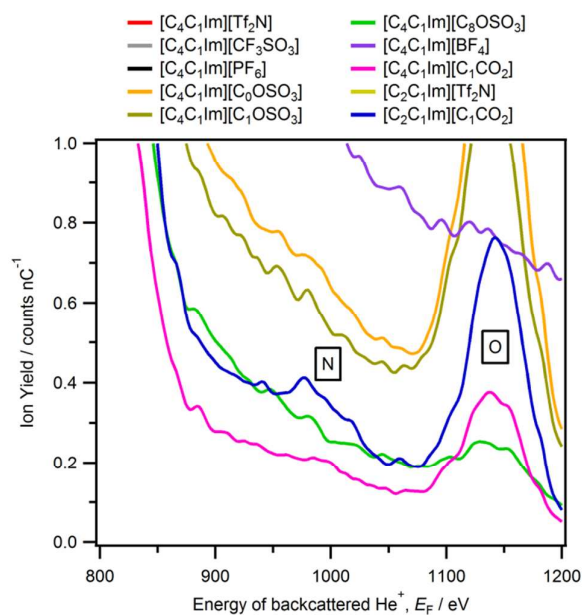
Figure 2. LEIS spectra ( {}^4\text{He}^+ , E_0 = 3 keV) for eight [\text{C}_4\text{C}_1\text{Im}][\text{A}] and two [\text{C}_2\text{C}_1\text{Im}][\text{A}] ionic liquids. The energy range given is 800 eV to 1200 eV, with the y-scale is cropped to zoom in on the cationic nitrogen peak observed for [\text{C}_2\text{C}_1\text{Im}][\text{C}_1\text{CO}_2] . Ionic liquids which contain cyano groups (e.g.
