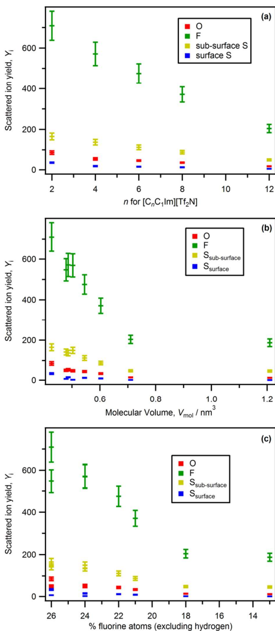
Figure 8. Scattered ion yield, Y_i , for [C_nC_1Im][Tf_2N] , [C_4C_1Pyrr][Tf_2N] , [N_{4,1,1,1}][Tf_2N] and [P_{6,6,6,14}][Tf_2N] vs.: (a) n for [C_nC_1Im][Tf_2N] , (b) molecular volume, V_{\text{mol}} , (c) percentage of fluorine atoms (excluding hydrogen atoms).
