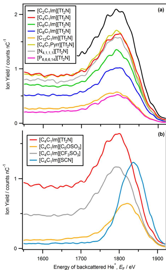
Figure 6. LEIS spectra ( ^4\text{He}^+ , E_0 = 3 keV) for sulfur-containing ionic liquids (region shown 1550 eV to 1920 eV): (a) [cation][Tf 2 N], (b) [C 4 C 1 Im][A].
