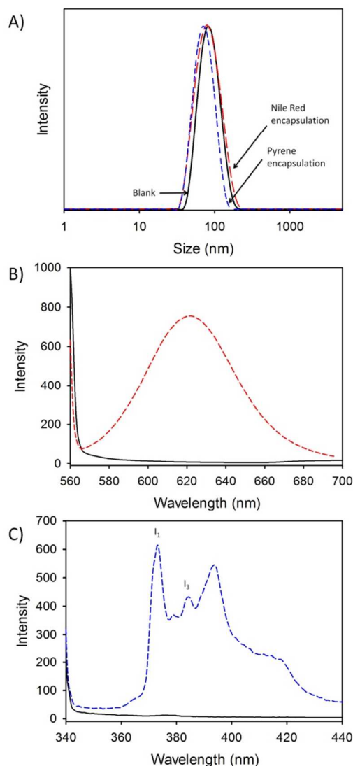
Fig. 6 Encapsulation of guest molecules during G_2 -(HPMA 50 -co-EGDMA 0.8 ) hyp -polydendron nanoprecipitation into water: A) DLS measurements of empty nanoprecipitates (black solid line), Nile Red containing nanoprecipitates (red long dashed line) and pyrene (blue short dashed line); B) Fluorescence spectroscopy of Nile Red loaded nanoprecipitates (red dashed line) vs. unloaded nanoprecipitates; C) Fluorescence spectroscopy of pyrene loaded nanoprecipitates (blue dashed line) vs. unloaded nanoprecipitates.
