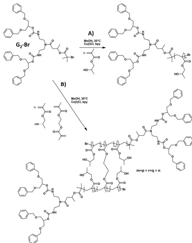
Scheme 2 Cu-catalysed ATRP Synthesis of A) linear dendritic hybrids and B) hyp -polydendrons using HPMA, EGDMA and G_2 -Br. Scheme shows only two polymer chains conjoined for clarity. Many additional chains are combined into the branched architecture
