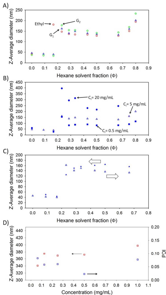
Fig. 3 Self-assembly of branched polymers on addition of hexane (bad solvent) to acetone (good solvent) solutions: A) Impact of hexane solvent fraction on z-average diameter for p(\text{HPMA}_{50-co}\text{-EGDMA}_{0.8}) (open red circles), G_1(\text{HPMA}_{50-co}\text{-EGDMA}_{0.8}) (open blue triangles) and G_2(\text{HPMA}_{50-co}\text{-EGDMA}_{0.8}) (open green diamonds); B) Impact of initial solution concentration ( C_i ) on self-assembly of G_1(\text{HPMA}_{50-co}\text{-EGDMA}_{0.8}) ; C) Reversible assembly of G_1(\text{HPMA}_{50-co}\text{-EGDMA}_{0.8}) (arrows indicate direction of solvent addition); and D) Robustness of G_1(\text{HPMA}_{50-co}\text{-EGDMA}_{0.8}) nanoparticles to dilution ( \Phi_{\text{hexane}} = 0.800 ).
