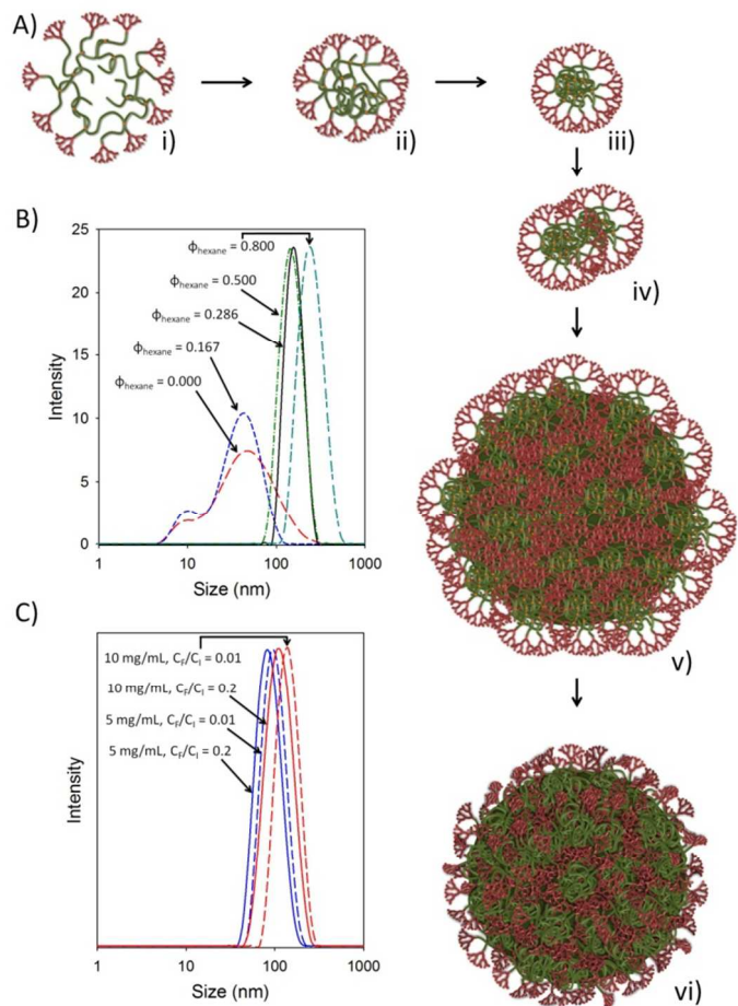
Fig. 5 Proposed mechanism for hyp -polydendron self-assembly and nanoprecipitation: A) Progressive collapse of solvated hyp -polydendrons to form nuclei (i-iii) and subsequent assembly to form swollen assemblies (iii-v) which finally desolvate and decrease slightly in hydrodynamic diameter (vi); B) Dynamic light scattering showing the impact of \Phi_{\text{hexane}} on the observed DLS size distributions; C) DLS measurements of aqueous hyp -polydendron nanoprecipitates formed from varying THF concentrations and different dilutions
