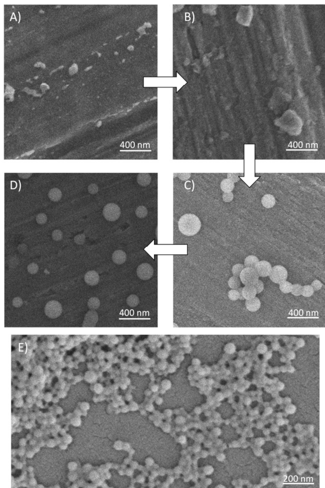
Fig. 4 Scanning electron microscopy of self-assembled nanoparticles from G_2 - (\text{HPMA}_{50}\text{-co-EGDMA}_{0.8}) . Hexane addition to acetone solutions with solvent fractions of: A) \Phi_{\text{hexane}} = 0.090 , B) \Phi_{\text{hexane}} = 0.286 , C) \Phi_{\text{hexane}} = 0.500 , and D) \Phi_{\text{hexane}} = 0.800 . E) Nanoparticles generated by aqueous nanoprecipitation from a THF solution ( C_1 = 5\text{mg/mL} ) an aqueous concentration of C_F = 1\text{mg/mL}
