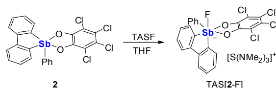
Scheme 1. Synthesis of TAS[2-F].
