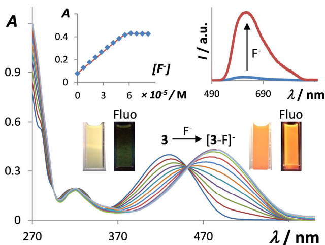
Figure 4. Spectral changes in the UV-Vis absorption spectrum of 3 ( 5.5 \times 10^{-5} M in \text{CH}_2\text{Cl}_2 ) upon addition of fluoride. The inset on the top left shows the experimental and the calculated 1:1 fluoride binding isotherms for 3 at 483 nm. The data were fitted with K > 10^7 \text{ M}^{-1} ( \epsilon(\mathbf{3}) = 1400 \text{ M}^{-1}\text{cm}^{-1} and \epsilon([\mathbf{3-F}]^-) = 7850 \text{ M}^{-1}\text{cm}^{-1} ). The inset on the top right shows the fluorescence spectra of 3 ( 5.0 \times 10^{-6} M in \text{CH}_2\text{Cl}_2 ) before and after addition of a stoichiometric amount of fluoride ( \lambda_{\text{excitation}} = 482 nm). The pictures of the cells were taken using a solution of 3 ( 5.5 \times 10^{-5} M) in \text{CH}_2\text{Cl}_2 , before and after addition of fluoride. The fluorescent images (labelled as Fluo) were illuminated with a hand-held UV lamp.
