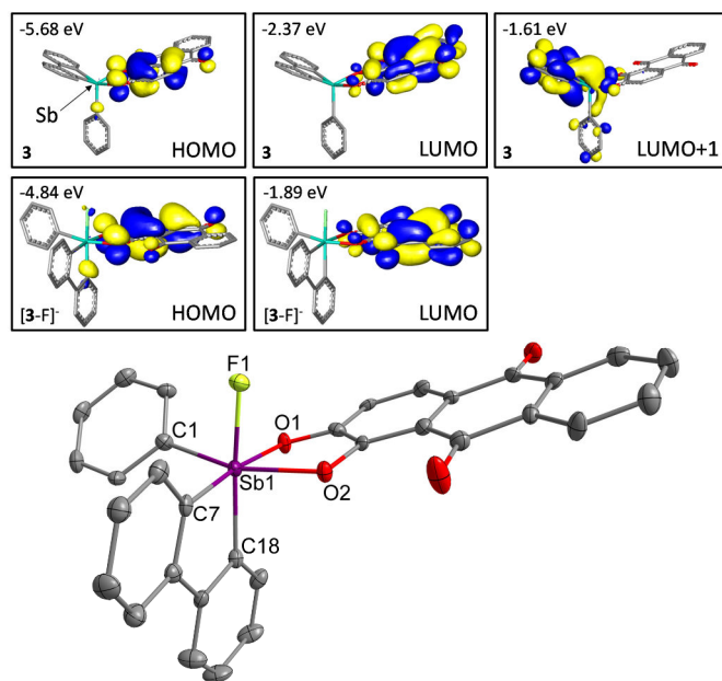
Figure 3. (top) Contour plot of the relevant orbitals in 3 and [3-F]^- (Isodensity = 0.036). (bottom) Structure of the crystallized enantiomer of TAS[3-F]. Thermal ellipsoids are drawn at the 50% probability level. The hydrogen atoms and the TAS cations are omitted for clarity. Selected bond lengths (Å) and angles (deg) with the corresponding metrical parameters for the second independent molecule in brackets: Sb1-F1 1.978(4) [1.979(2)], Sb1-O1 2.077(3) [2.082(3)], Sb1-O2 2.100(3) [Sb2-O6 2.100(2)], Sb1-C1 2.126(4) [2.127(4)], Sb1-C7 2.132(4) [2.128(4)], Sb1-C18 2.141(4) [2.138(4)], F1-Sb1-C18 172.14(12) [170.05(12)], C1-Sb1-O2 160.53(12) [162.58(12)], C7-Sb1-O1 172.36(12) [171.80(12)], O1-Sb1-O2 77.61(10) [77.90(10)], C7-Sb1-C18 82.02(15) [81.96(14)].
