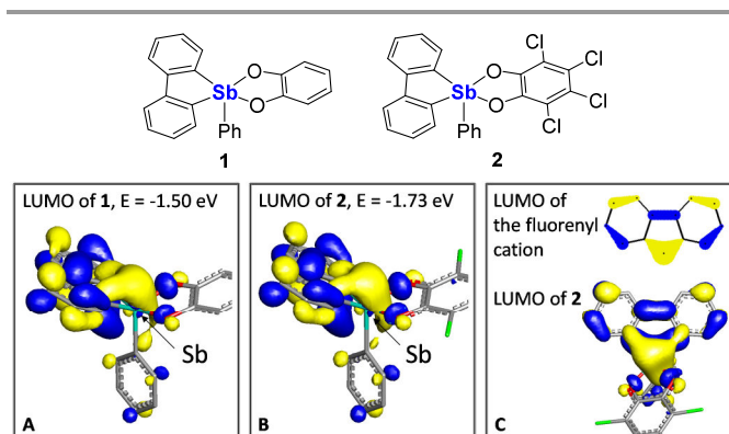
Figure 1. (top) Chemical structures of 1 and 2 . (bottom) Contour plot and energy of the LUMO in 1 (panel A) and 2 (panel B) (Isodensity = 0.036). Panel C shows the similarity existing between the LUMO of the fluorenyl cation and that of 2 .
