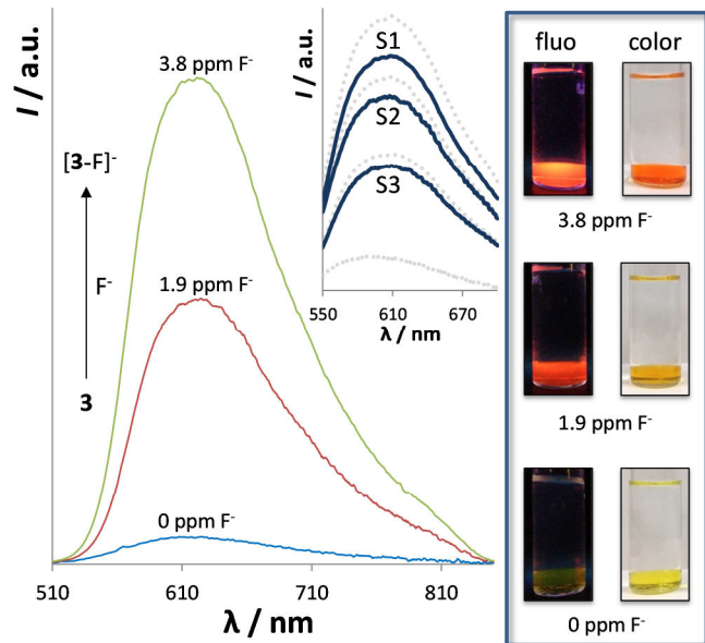
Figure 5. (A) Fluorescence spectra ( \lambda_{\text{excitation}} = 482 nm) of solutions of 3 ( 5.0 \times 10^{-6} M) in \text{CH}_2\text{Cl}_2 . For each measurement, the solution was prepared by the 100-fold dilution of a 5.0 \times 10^{-4} M solution of 3 which had been layered with an aqueous solution of KF (0, 1.9 and 3.8 ppm) containing TPABr (20 mM) and a citrate buffer (10 mM, pH 4.68). (B) Drinking water analysis data: each fluorescence spectrum is obtained with a solution of 3 in \text{CH}_2\text{Cl}_2 ( 5.0 \times 10^{-5} M) after layering with a standard fluoride solution or an unknown sample. The spectra drawn with dotted lines correspond to the standard fluoride solutions (0, 0.4, 0.7 and 1.0 ppm, from bottom to top). The spectra obtained for the unknown samples are drawn with solid lines (S1 = H-E-B® Baby Purified Water (with fluoride added); S2 = Nursery® Water; S3 = College Station Tap Water). (C) Naked-eye fluorescence and colorimetric response associated with the formation of [3-F]^- at a concentration of 5.0 \times 10^{-4} M.
