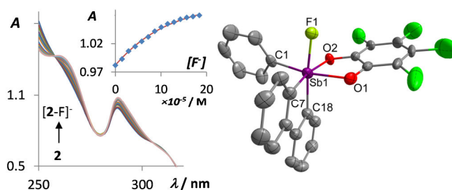
Figure 2. Left: absorption spectra in 7/3 vol. THF/water showing the conversion of 2 ( 7.2 \times 10^{-5} M) into [2-F] - upon addition of fluoride anions. The inset shows the experimental and the calculated 1:1 fluoride binding isotherm for 2 . The data were measured at 287.4 nm and fitted with K = 13500 (\pm 1400) \text{ M}^{-1} ( \epsilon(\mathbf{2}) = 13600 \text{ M}^{-1}\text{cm}^{-1} and \epsilon([\mathbf{2-F}]^{-}) = 15300 \text{ M}^{-1}\text{cm}^{-1} ). Right: Crystal structure of TAS[2-F]. Thermal ellipsoids are drawn at the 50 % probability level. The hydrogen atoms and the TAS cation are omitted for clarity. Selected bond lengths (Å) and angles (deg): Sb1-F1 1.973(4), Sb1-O1 2.105(4), Sb1-O2 2.082(4), Sb1-C1 2.131(6), Sb1-C7 2.128(6), Sb1-C18 2.141(6), F1-Sb1-C18 172.11(18), C1-Sb1-O1 168.21(19), O2-Sb1-C7 167.51(19), O1-Sb1-O2 78.65(16), C7-Sb1-C18 82.8(2).
