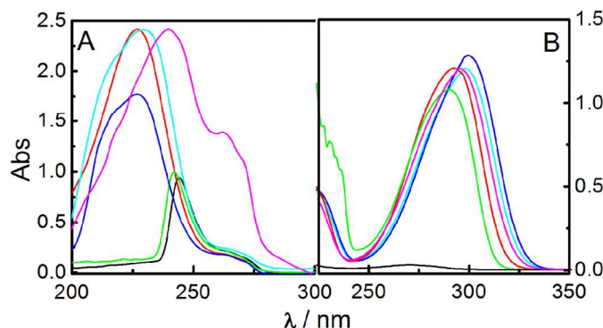
Figure 7. UV-visible absorption spectra of 1 mM LIDO (panel A) and PRO.HCl (panel B) loaded in NLC as well as solvents of different polarity; at 25 °C. Systems : —, n-hexane; —, acetonitrile; —, chloroform; —, ethanol; —, methanol and —, drug loaded NLC respectively.
