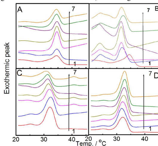
Figure 4. DSC cooling curves of LIDO (panel A) and PRO.HCl (panel B) loaded NLC dispersed in Tween 40; LIDO (panel C) and PRO.HCl (panel D) loaded NLC dispersed in Tween 60. 5 mM NLC with Span 65 + SLC + SA, 2:2:1 M/M/M, was dispersed in 10 mM aqueous Tween solution. Concentration of drug (mM): 1, 0; 2,0.2; 3,0.5; 4,1.0; 5,1.5; 6,2.0 and 7,2.5. Scan rate 2 °C/min.
