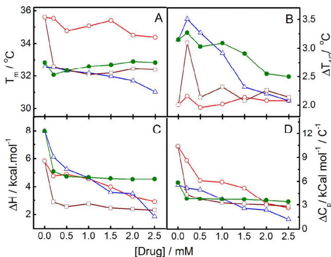
Figure 5. Effects of drugs on the temperature of maximum heat flow ( T_m , panel A), width of half peak height ( \Delta T_{1/2} , panel B), change in enthalpy ( \Delta H , panel C) and heat capacity ( \Delta C_p , panel D) of NLCs (Span65 + SLC + SA, 2:2:1 M/M/M). 5 mM lipid was dispersed in 10 mM aqueous Tween solution. System O; LIDO loaded in Tween 40: \Delta ; LIDO loaded Tween 60: \square ; PRO.HCl loaded Tween 40: \bullet ; PRO.HCl loaded Tween 60: \circ .
