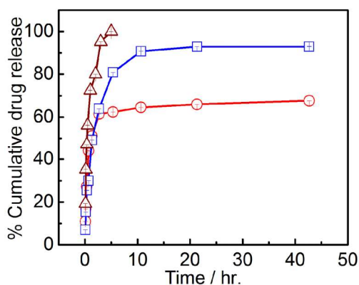
Figure 10. In vitro cumulative PRO.HCl release from NLC (5mM, Span 65 + SLC + SA, 2:2:1 M/M/M). Systems: PRO.HCl loaded dispersion in Tween 40 (O), Tween 60 (□) and free PRO.HCl in Tween 60 (Δ). Each point represents the mean \pm (S.D.) (n=3). Drug concentration was kept constant at 0.5 mM in each case. Temp. 25 °C.
