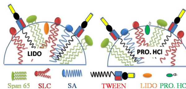
Scheme 1. Proposed model for the organization of lipids and drugs in the NLC formulations stabilized by Tweens.
