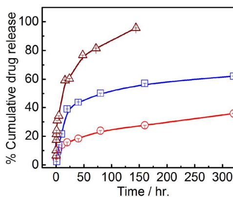
Figure 9. In vitro cumulative LIDO release from NLC (5mM, Span 65 + SLC + SA, 2:2:1 M/M/M). System: LIDO loaded NLC dispersion in Tween 40 (O), Tween 60 (□) and free LIDO in Tween 60 (Δ). Each point represents the mean \pm (S.D.) (n=3). Drug concentration was kept constant at 0.5 mM in each case. Temp. 25 °C.
