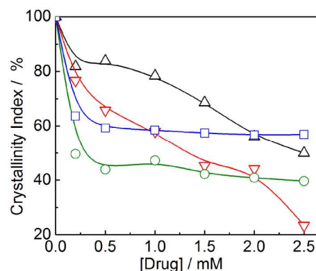
Figure 6. Effects of drug concentration on the degree of crystallinity of NLC (5 mM, Span 65+SLC+SA, 2:2:1 M/M/M). Systems: \Delta , LIDO -Tween 40; \nabla , LIDO -Tween 60; \circ , PRO.HCl-Tween 40 and \square , PRO.HCl-Tween 60.
