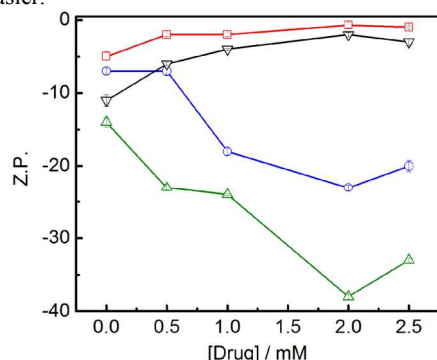
Figure 2. Influence of LIDO and PRO.HCl on the (Z.P.) of NLCs (Span 65 + SLC + SA, 2:2:1 M/M/M) dispersed in Tweens. Systems: O, LIDO -Tween 40; Δ, LIDO -Tween 60; □, PRO.HCl-Tween 40 and ∇, PRO. HCl -Tween 60. Temp. 25 °C. 5 mM lipid in the absence and presence of the drug was dispersed in 10 mM aqueous Tween solution.
