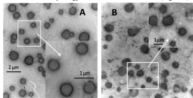
Figure 3. Representative TEM images of LIDO loaded NLC dispersion in Tween 40 (A) and PRO.HCl loaded NLC dispersion in Tween 40 (B).
