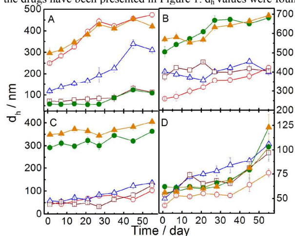
Figure 1. Hydrodynamic diameter ( d_h ) – time profile of NLCs (Span 65 + SLC + SA, 2:2:1 M/M/M) dispersed in Tweens in presence of varying concentration of drugs. Panel A: LIDO loaded NLC in Tween 40; panel B: PRO.HCl loaded NLC in Tween 40; panel C: LIDO loaded NLC in Tween 60 and panel D: PRO.HCl loaded NLC in Tween 60. 5 mM NLC was dispersed in 10 mM Tweens in each case. Drug concentration (mM): O, 0; Δ, 0.5; □, 1; ●, 2 and ▲, 2.5. Temp. 25 °C.
