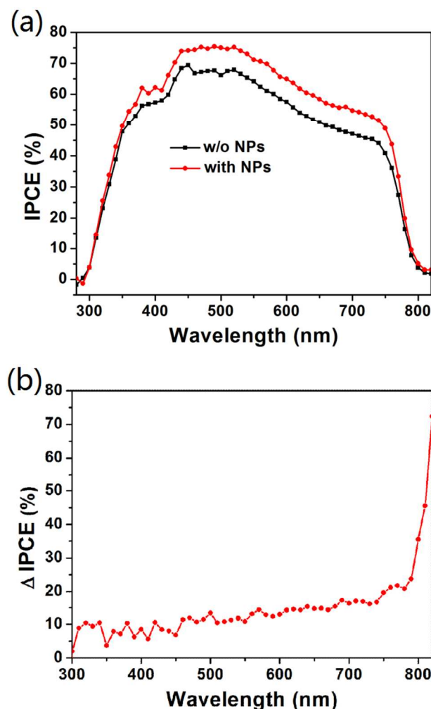
Fig. 5 (a) IPCE spectra (from 280 nm to 820 nm) of devices with and without Au-Ag alloy popcorn NPs. (b) IPCE enhancement ratio ( \Delta IPCE) of the perovskite devices. \Delta IPCE = (IPCE with NPs ( \lambda )-IPCE w/o NPs ( \lambda ))/IPCE w/o NPs ( \lambda ) \times 100%, where IPCE with NPs ( \lambda ) and IPCE w/o NPs ( \lambda ) are the IPCEs of the perovskite devices with and without popcorn NPs at wavelength of \lambda , respectively.
