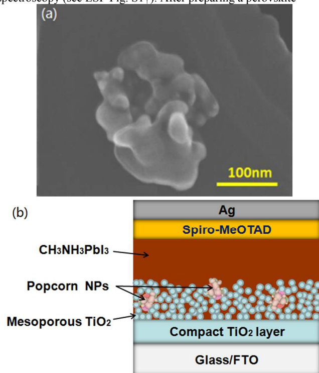
Fig. 1 (a) TEM image of a popcorn NP. (b) Illustrative structure of the perovskite solar cell with popcorn NPs embedded in the mesoporous TiO 2 framework.
