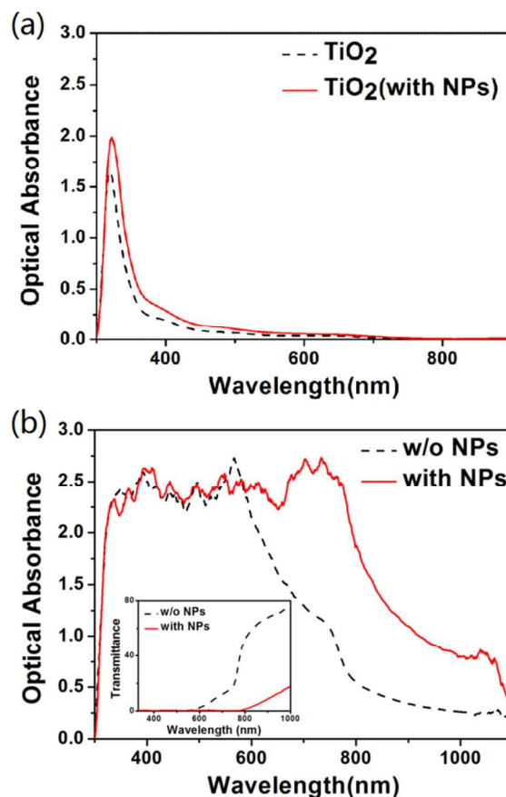
Fig. 3 (a) Optical absorption spectra of mesoporous TiO 2 layer with and without popcorn NPs. (b) Optical absorption of perovskite film on mesoporous TiO 2 framework with and without popcorn NPs. The inset shows the transmittance spectra.
