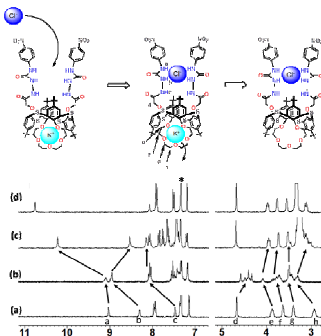
Fig. 7 Proposed negative allosteric behaviour of 4 e with Cl − and K + ions. Partial 1 H NMR spectra of 4 e /guest (H/G = 1:1); a) free 4 e ; b) 4 e ⊃ KSO 3 CF 3 ; c) Bu 4 NCl ⊃ [ 4 e ⊃ K + ]; d) 4 e ⊃ Bu 4 NCl. Solvent: CDCl 3 –DMSO (10:1, v/v). 300 MHz at 298 K. *Denotes the solvent peak.
