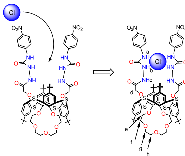
Fig. 3 Binding mode of receptor 4 e upon complexation with Cl - ions.
