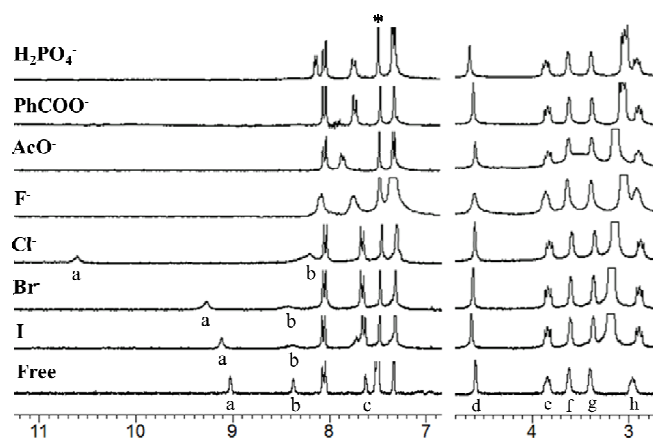
Fig. 5 Partial 1 H NMR spectra of receptor 4 e /guest (H/G = 1:1); free receptor 4 e and in the presence of 1 equiv. of Bu 4 NX (X = F, Cl, Br, I, AcO, PhCOO, H 2 PO 4 ), respectively. Host concentration was 2.5 μM. Solvent: CDCl 3 –DMSO (10:1, v/v). 300 MHz at 298 K. *Denotes the solvent peak.
