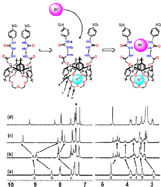
Fig. 6 Proposed positive allosteric behaviour of receptor 4 e with Br − and K + ions. Partial 1 H NMR spectra of 4 e /guest (H/G = 1:1); a) free 4 e ; b) 4 e ⊃ KSO 3 CF 3 ; c) Bu 4 NBr ⊃ [ 4 e ⊃ K + ]; d) 4 e ⊃ Bu 4 NBr. Solvent: CDCl 3 –DMSO (10:1, v/v). 300 MHz at 298 K. *Denotes the solvent peak.
