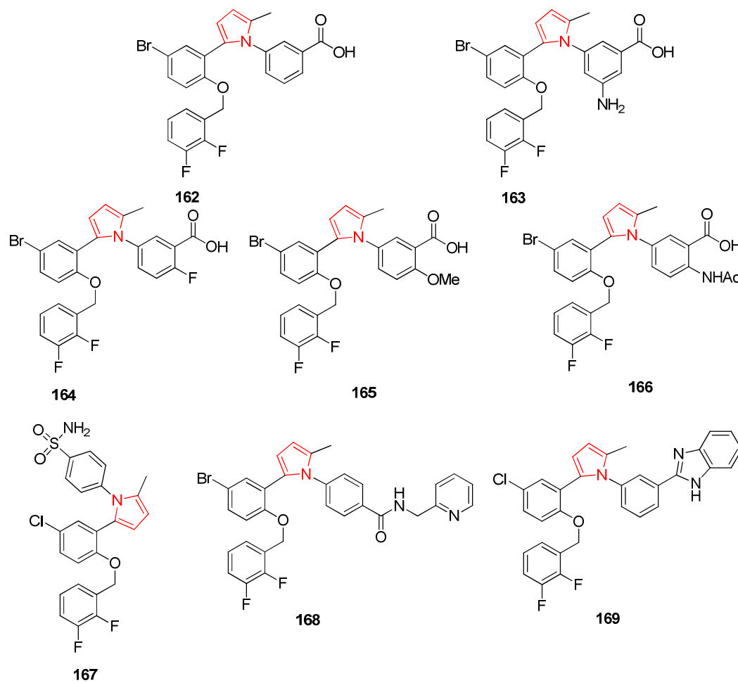
Figure 3. Pyrrole containing compounds as EP 1 receptor antagonist.
