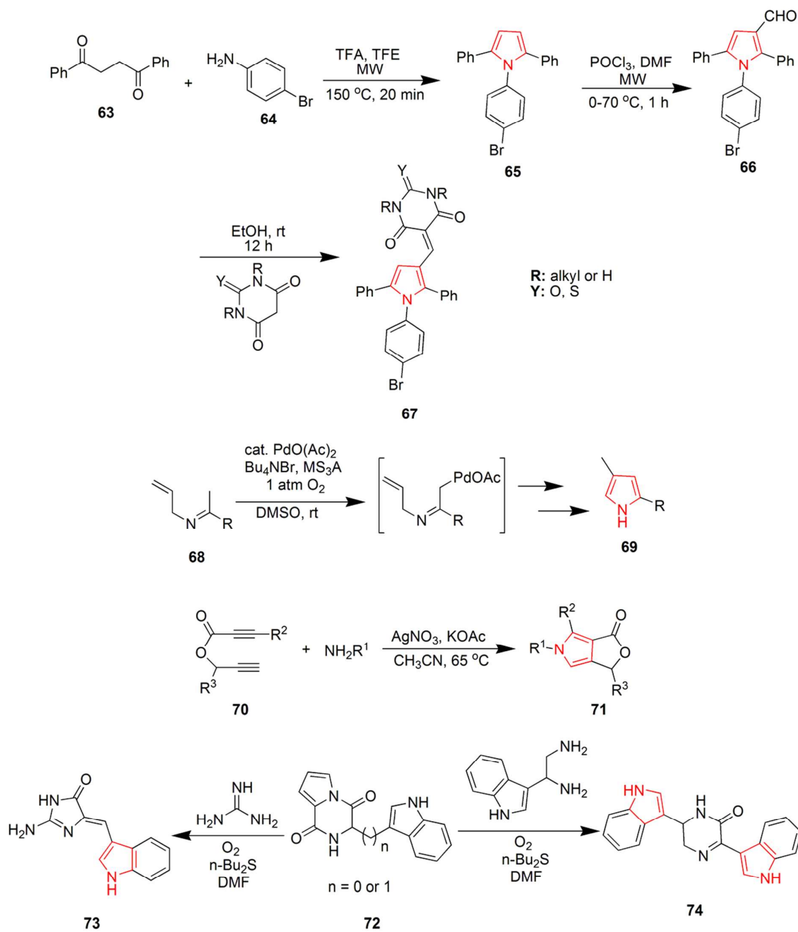
Scheme 12 Synthetic route for catalyzed pyrrole containing analogs.
