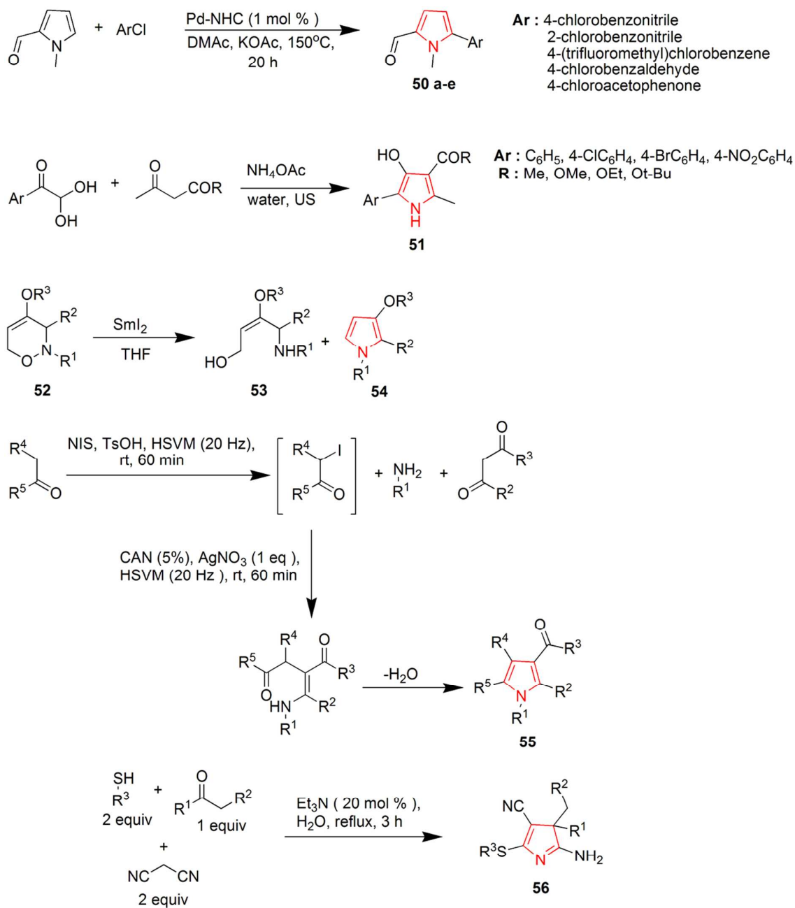
Scheme 10 systemic approach to synthesize substituted pyrroles.
