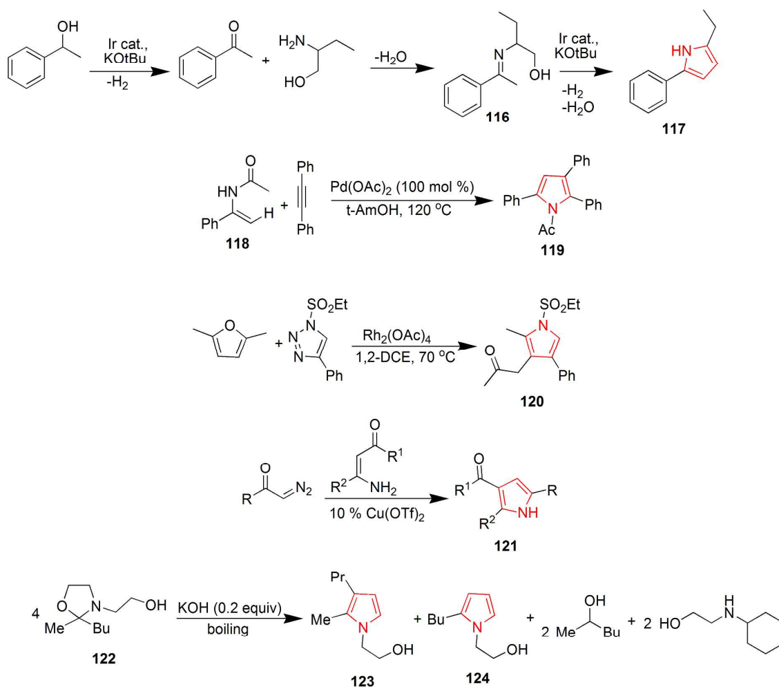
Scheme 18 Synthesis of catalyzed pyrrole molecules.
