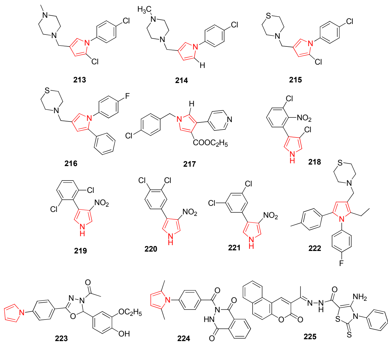
Figure 7. Pyrrole containing compounds with antimycobacterial activity.
