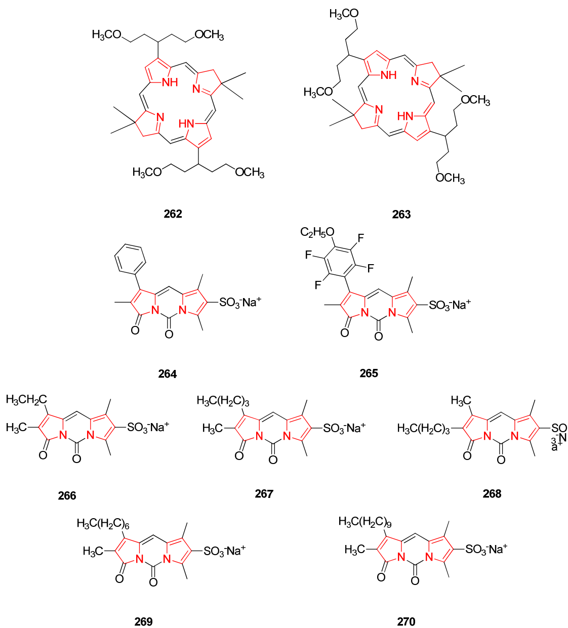
Figure 13. Pyrrole containing compounds as diagnostic and therapeutic agents
