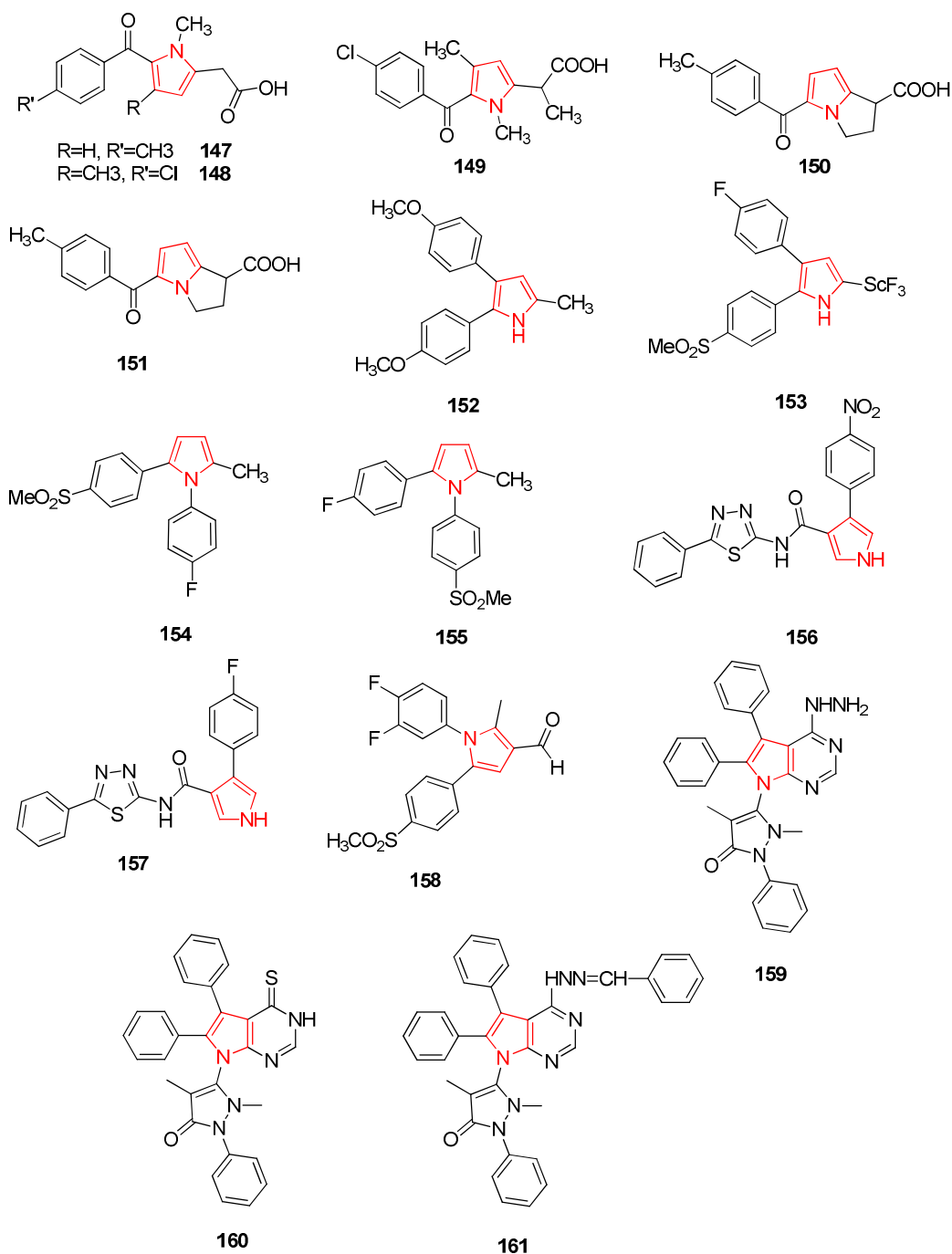
Figure 2. Pyrrole containing compounds with anti-inflammatory activity.
