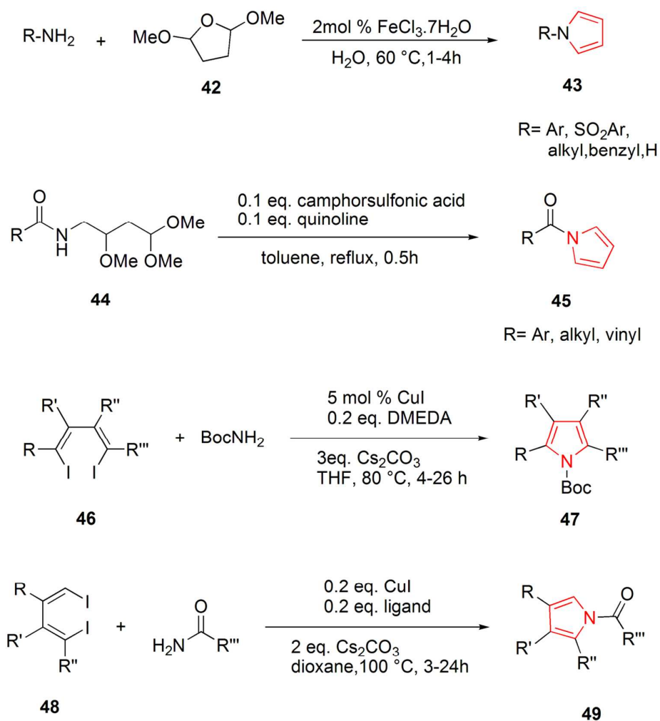
Scheme 9 Synthesis of substituted pyrrole containing analogs.
