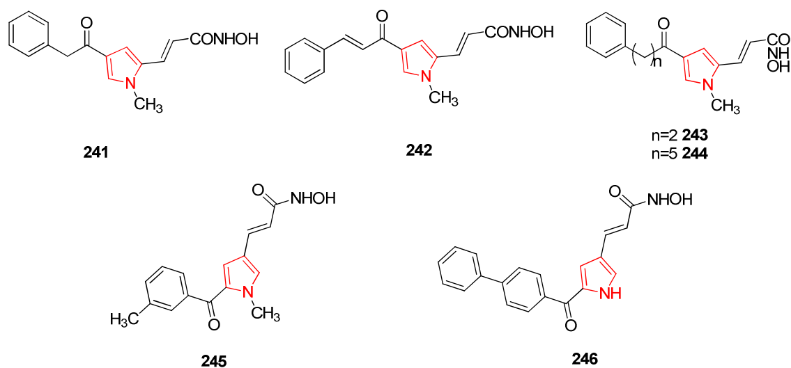
Figure 9. Pyrrole containing compounds as Histone deacetylase inhibitors.
