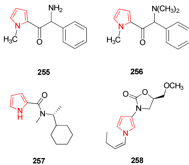
Figure 11. Pyrrole containing compounds as Monoamine oxidase inhibitors.
