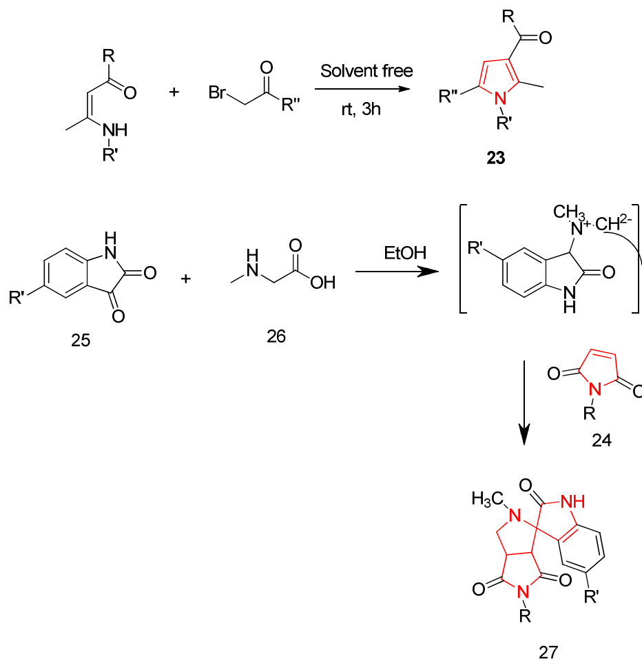
Scheme 5 Synthesis of pyrrole containing analogs.
