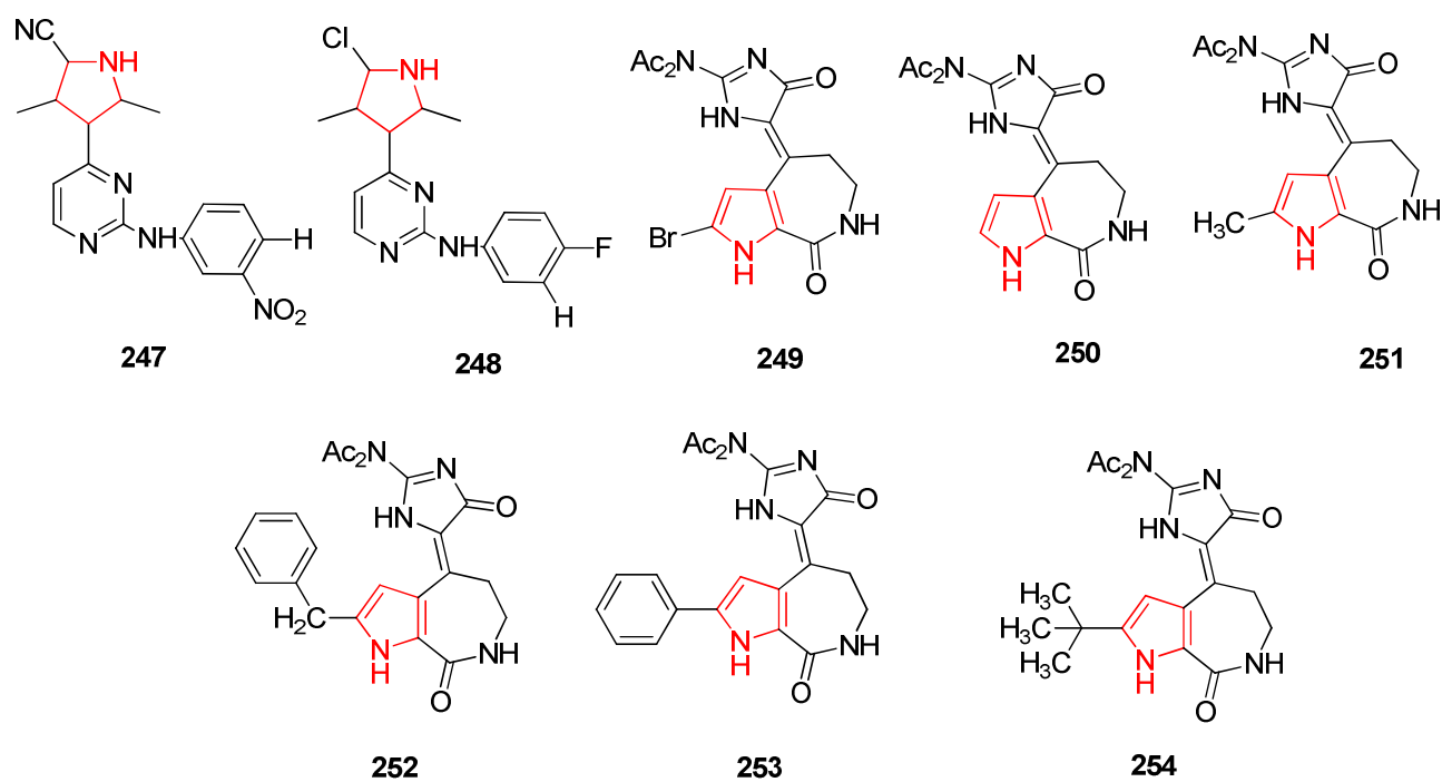
Figure 10. Pyrrole containing compounds as CDK inhibitors.
