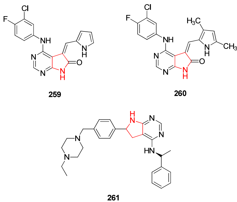
Figure 12. Pyrrole containing compounds as EGFR inhibitors.
