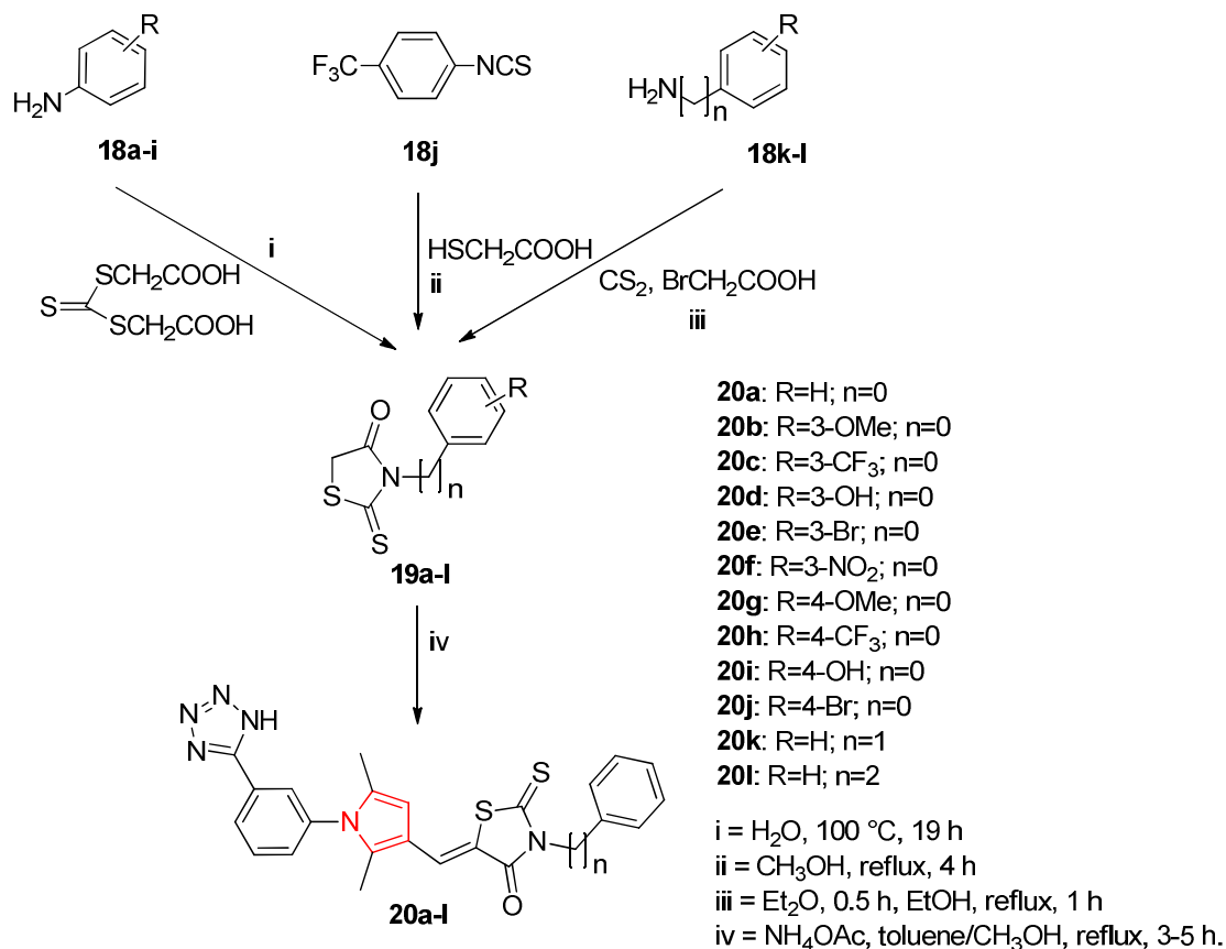
Scheme 2 Synthesis of rhodanine derivatives.
