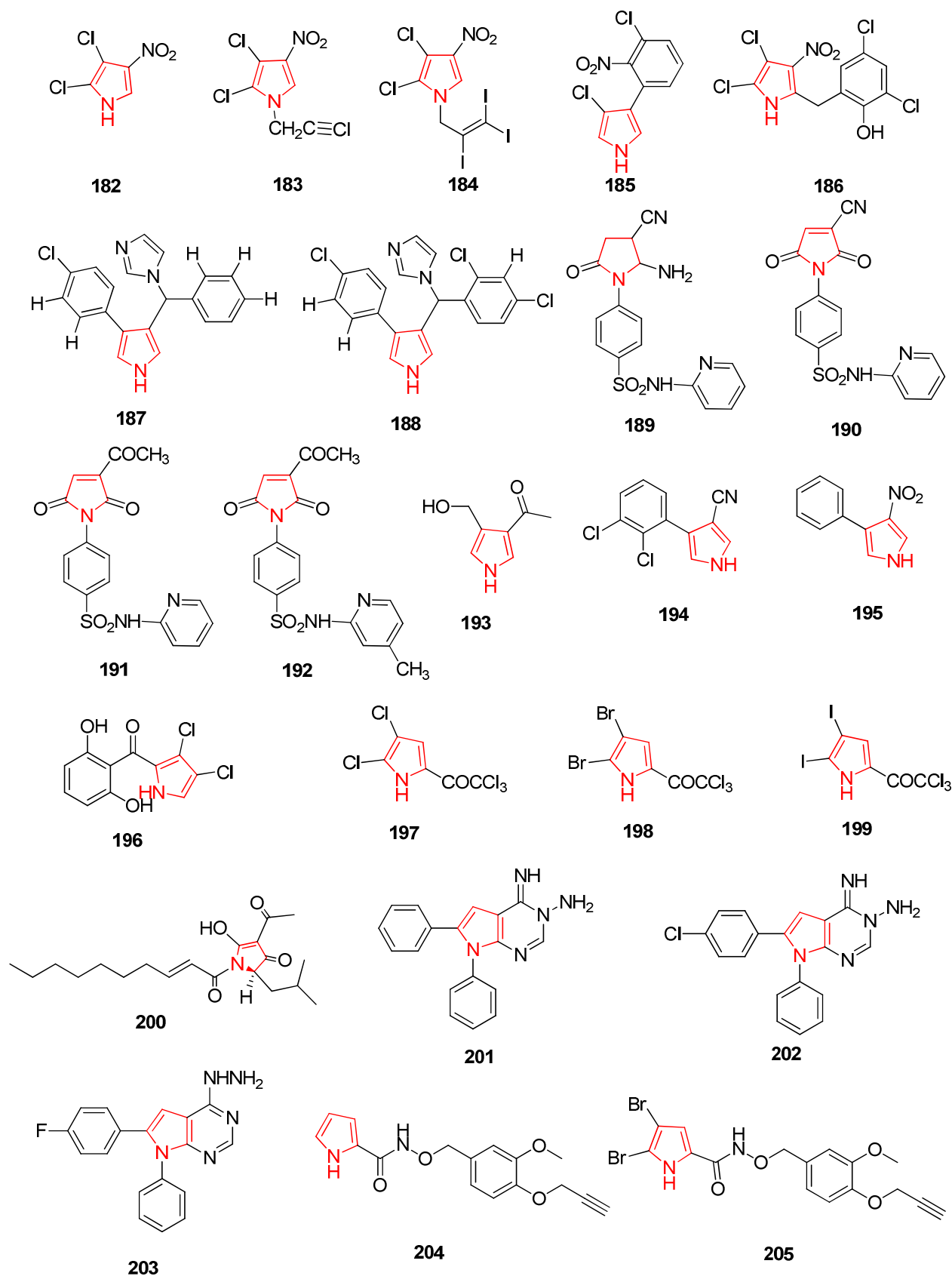
Figure 5. Pyrrole containing compounds with antifungal and antibacterial activity.
