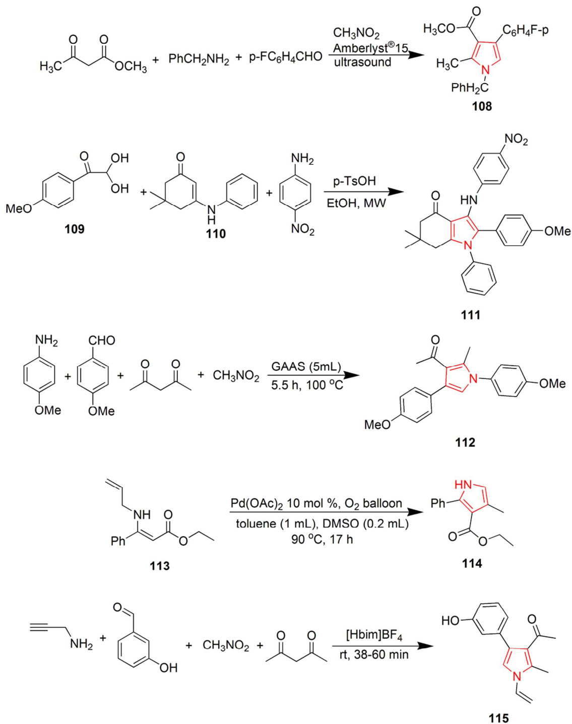
Scheme 17 Synthesis of various catalyzed pyrrole analogs.
