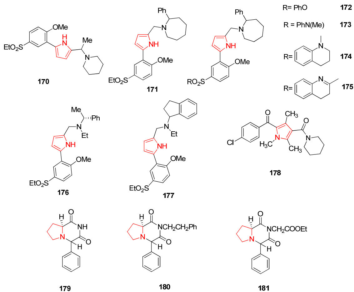
Figure 4. Pyrrole containing compounds with antipsychotic and anticonvulsant activity.
