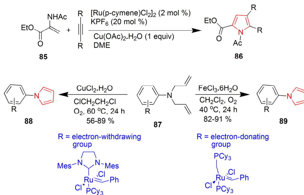
Scheme 14 Synthesis of metal catalyzed pyrroles.
