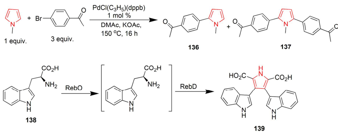
Scheme 20 Catalysis assisted formation of pyrrole containing compound.
