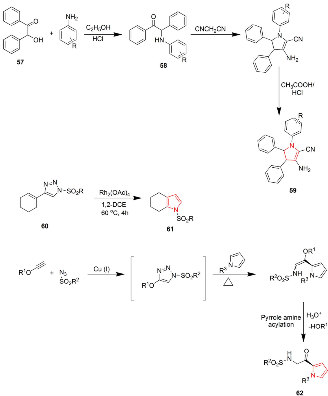
Scheme 11 Synthesis of various catalyzed pyrrole containing products.
