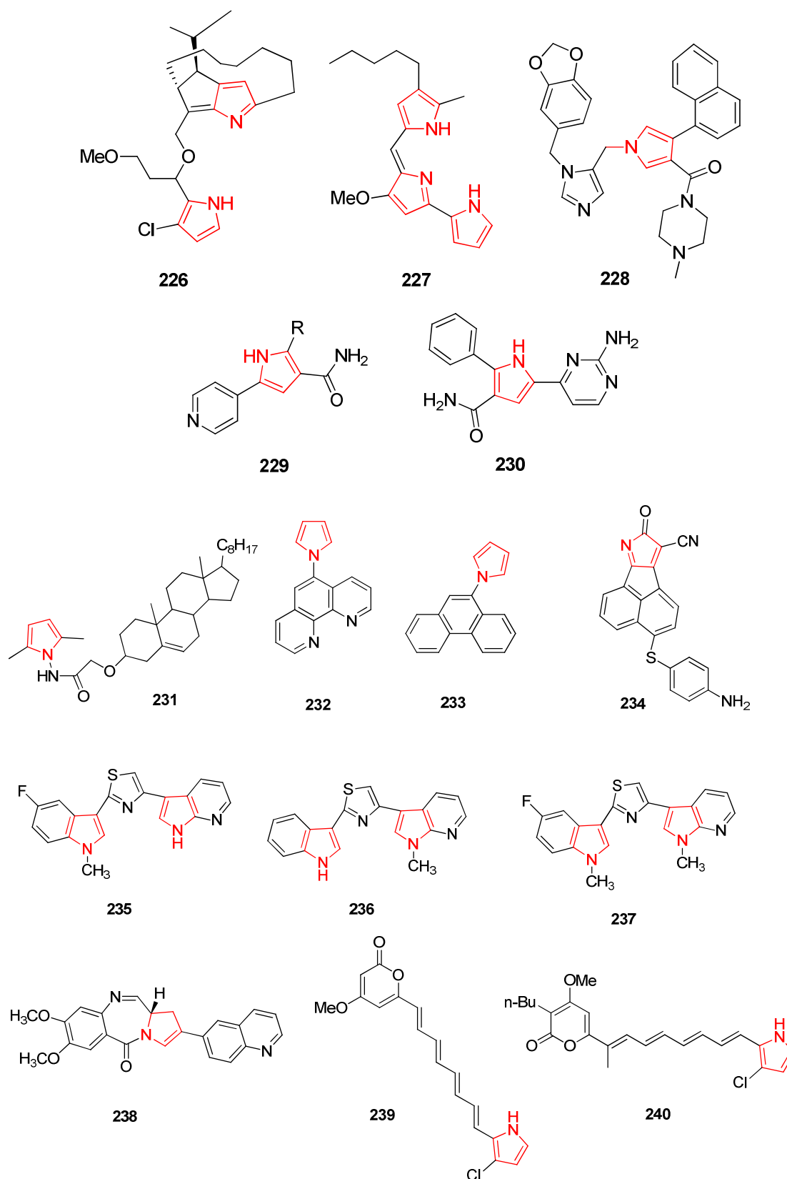
Figure 8. Pyrrole containing compounds with anti tumor activity.
