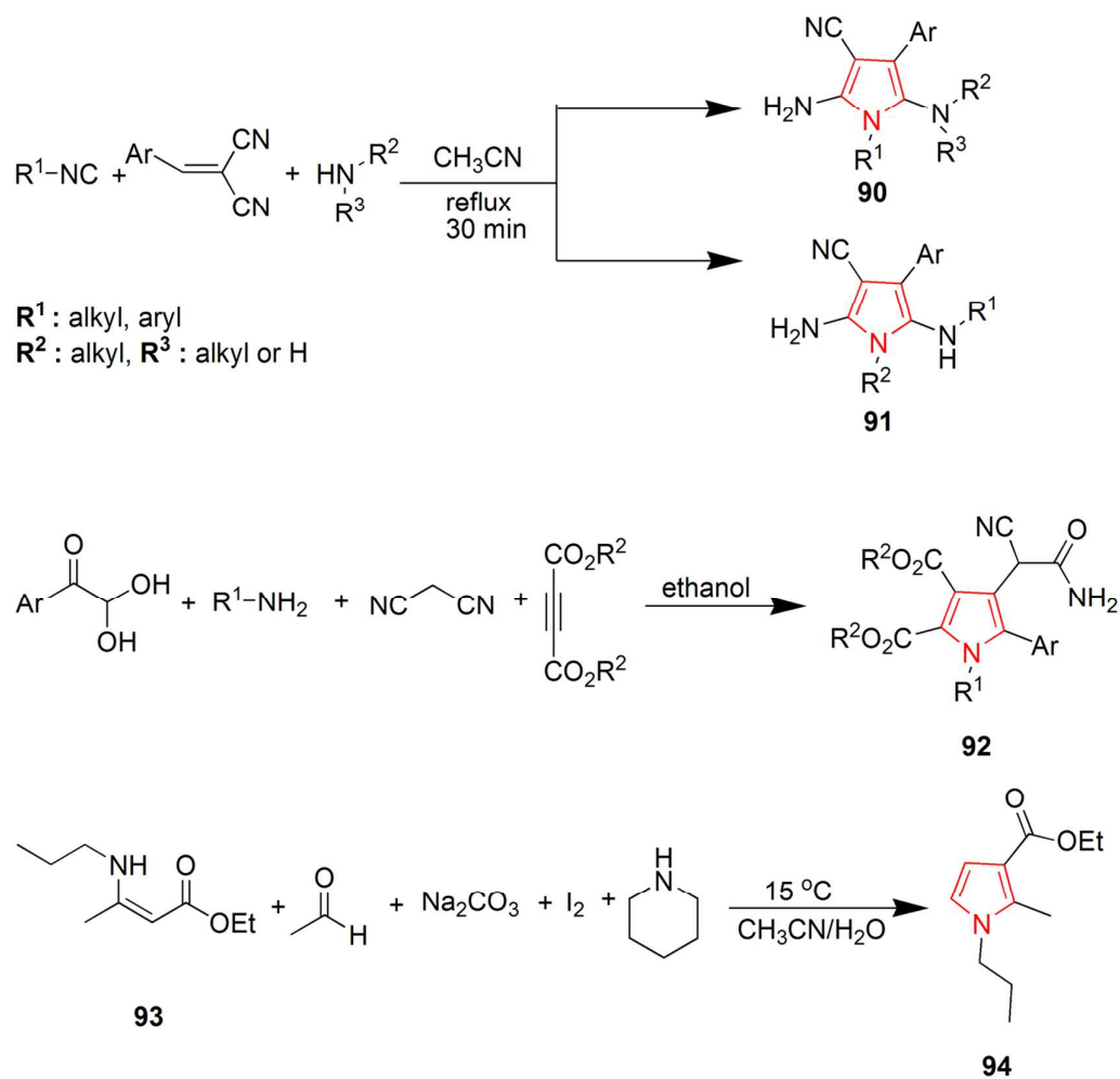
Scheme 15 Synthesis of pyrroles using various solvent systems.
