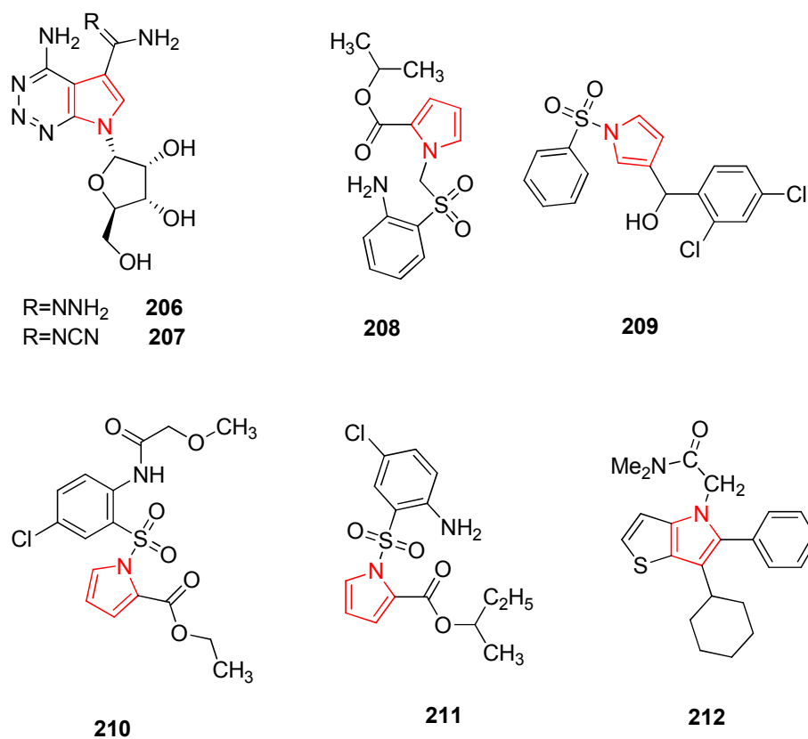
Figure 6. Pyrrole containing compounds with antiviral activity.
