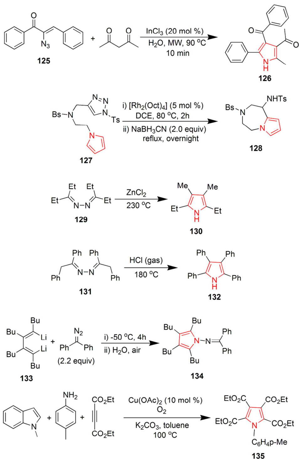
Scheme 19 Substituted pyrrole molecules.
