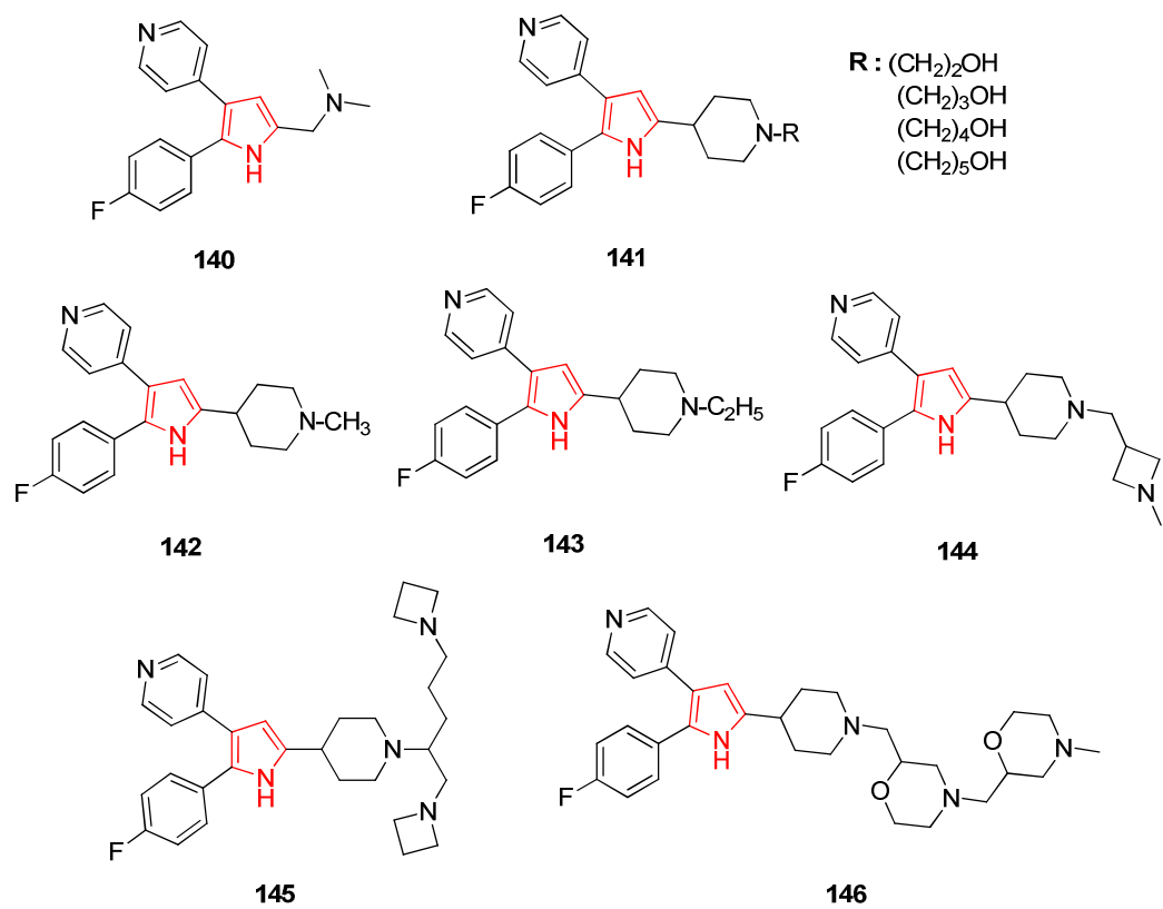
Figure 1. Pyrrole containing compounds with anticoccidial activity.
