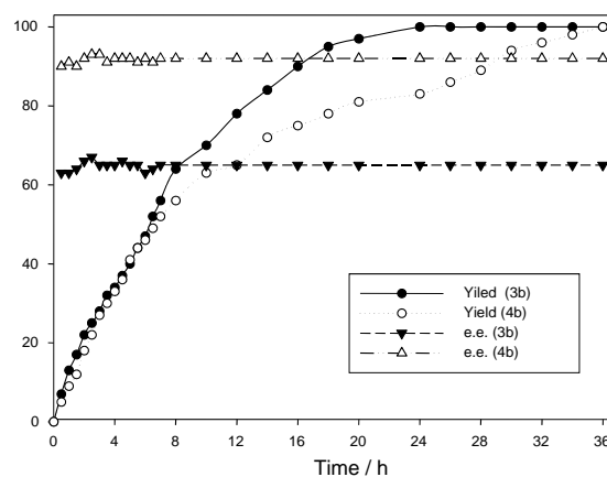
Fig. 7 Kinetic analysis of the reaction of benzaldehyde with Et 2 Zn using catalysts 3b and 4b at 0 °C in toluene. Selectivity > 99%
