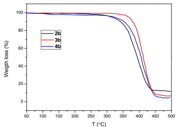
Fig. 6 Thermal analysis of the polymeric ligand 2b , and the polymeric complexes 3b and 4b .
