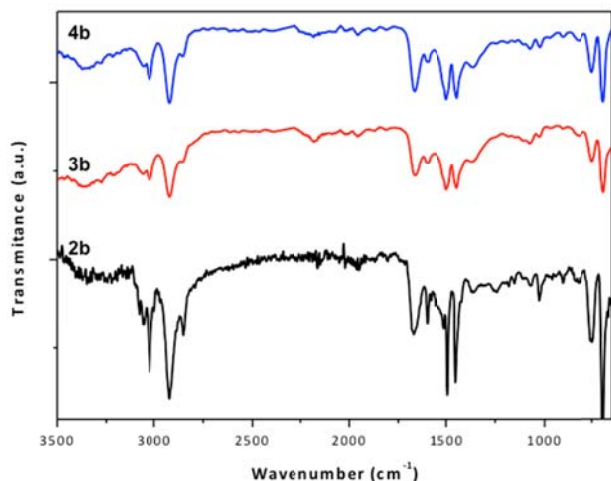
Fig. 3 FTIR spectra for polymers 2b , 3b and 4b ; 3b and 4b prepared from 2b containing 1 mmol of \alpha -amino amide/g of resin.
