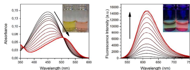
Fig. 2 Absorption and fluorescence spectra of G3 (5.0 μM) upon addition of WPA5 (0 to 1.46 equiv.) in water (excitation at 506 nm); inset: photographs showing colorimetric and fluorescent changes in aqueous solution (10.0 μM G3 (left vial), 10.0 μM G3 and 30.0 μM WPA5 (right vial)) Note: aqueous solution of WPA5 is colorless and therefore omitted
