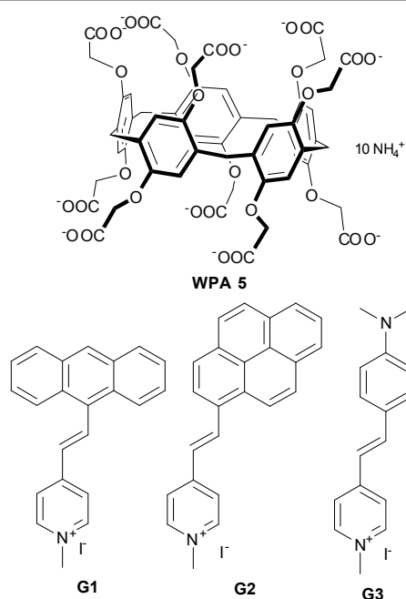
Fig. 1 Structures of WPA5 and guests G1-G3
