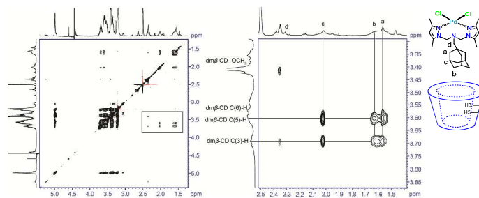
Figure 2. (left) 2D NOESY 1 H NMR spectrum of Ad-L-PdCl 2 and dm \beta -CD in D 2 O/DMSO- d 6 (1:1, v/v) with water suppression (500 MHz, 25°C); (right) Expanded 2D NOESY 1 H NMR spectrum.
