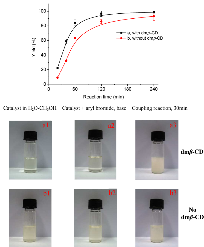
Figure 3. (top) Comparison of Suzuki-Miyaura coupling reactions performed in H 2 O-CH 3 OH (3/1, v/v) with and without dmβ-CD in air at room temperature over 4h. Each point represents the mean value ± SD of 2 runs; (bottom) Photographs comparing the homogeneity of catalyst and catalyst mixed with 4-bromobenzoic acid/Na 2 CO 3 in H 2 O-CH 3 OH (3/1, v/v), as well as the turbidity of the reaction mixtures after adding phenylboronic acid in 30 min with (a1-a3) and without (b1-b3) the host dmβ-CD, respectively.
