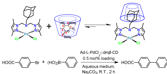
Scheme 2. Suzuki-Miyaura coupling reaction of 4-bromobenzoic acid and phenylboronic acid in aqueous media catalyzed by supramolecular inclusion complex catalyst (Ad-L-PdCl 2 ⊂dmβ-CD).
