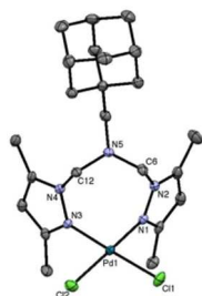
Figure 1. ORTEP diagram of adamantyl-containing Pd(II) complex shown with 50% probability ellipsoids (hydrogen atoms are omitted for clarity).
