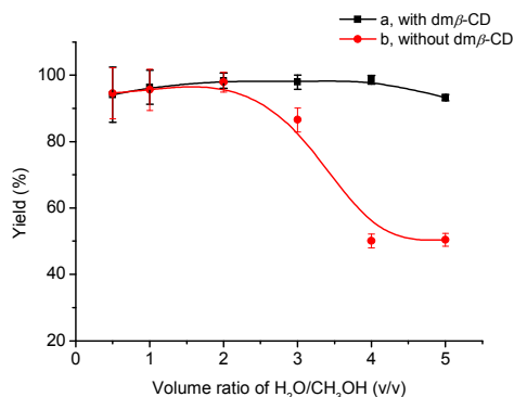
Figure 4. Comparison of Suzuki-Miyaura coupling performed in various proportions of H 2 O and CH 3 OH, with and without dm \beta -CD (conditions: room temperature, 2 h in air). Each point represents the mean value \pm SD of 2 runs.
