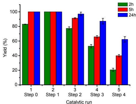
Figure 5. Variation of yield with increasing reaction time in catalyst recycling experiments; 4-bromobenzoic acid (1.0 equiv., 0.125 mol/L), phenylboronic acid (1.2 equiv.), initial catalyst loading (0.5 mol%, for step 0), TBAB (0.15 equiv.), pH (11.0, at the beginning of each step), room temperature, air, water-methanol (3:1, v/v). Each point represents the mean value \pm SD of 2 runs.
