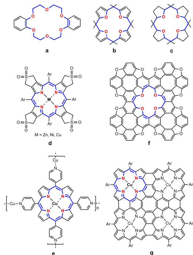
Fig. 1 Some examples of the well known crown ethers a-c and of the recently synthesized reactive building-blocks containing porphyrin ( d, e, g ) and tetraoxa[8]circulene ( f ) cores.
