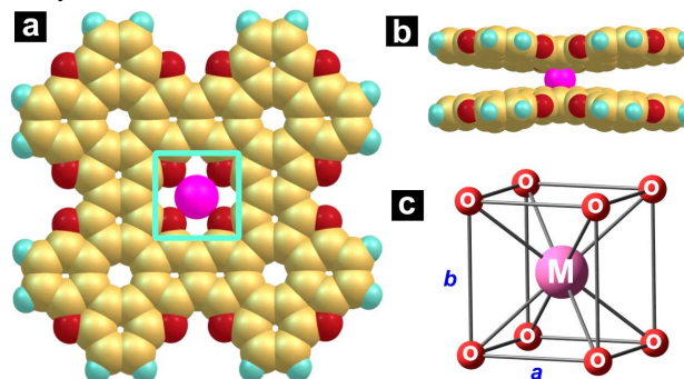
Fig. 3 The optimized structure of the sandwich-type complexes [\text{M}(\text{TOC})_2]^{n+} ( \text{M} = \text{K}^+ , 6 ; \text{Ca}^{2+} , 7 ): a – top view, b – side view, c – prism-shaped coordination cage consisting of the \text{K}^+ or \text{Ca}^{2+} ions ( a \neq b ).
