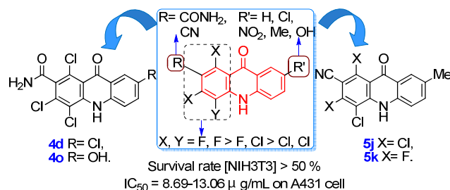
Scheme 2 The preliminary structure-selectivity relationship of polyhalo acridones.
