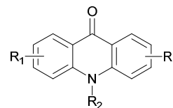
Fig. 1 The structure of acridone compounds
