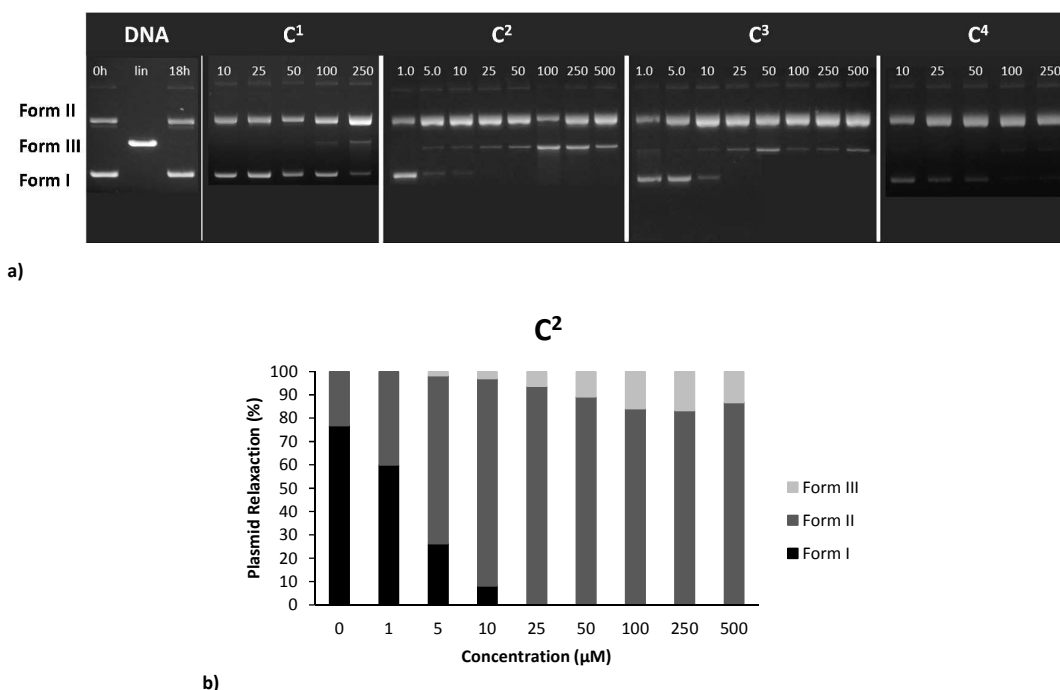
Figure 7. a) Agarose gel electrophoresis patterns for the cleavage of supercoiled \phi X174 phage DNA by C^1 - C^4 complexes after 18h of incubation at 37°C in phosphate buffer (pH 7.2) and b) percentage of plasmid relaxation for C^2 . Forms I, II and III are supercoiled, nicked circular and linear forms of DNA, respectively.
