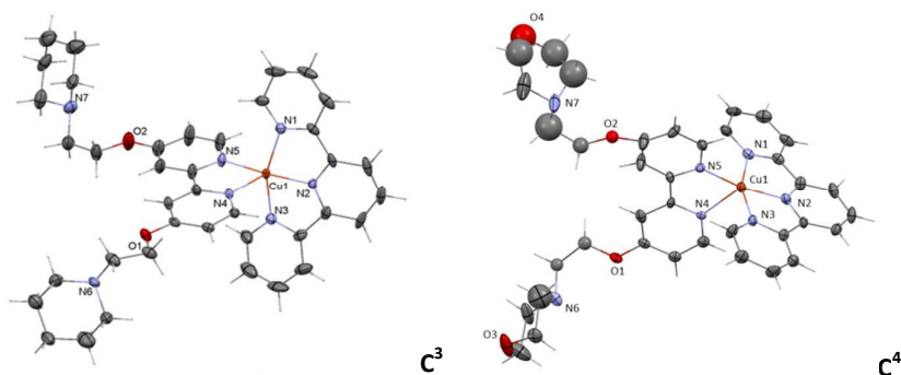
Figure 1. ORTEP diagram of \mathbf{C}^3 and \mathbf{C}^4 . Ellipsoids were drawn at the 40% probability level.
