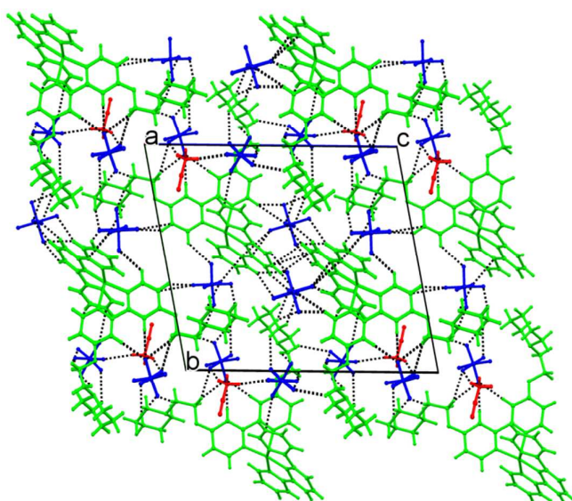
Figure 2. The crystal structure of C 4 . View along the stacking axis a emphasizing the short contacts.
