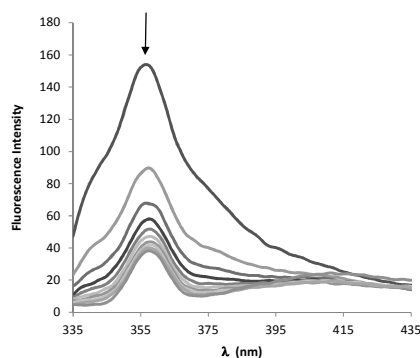
Figure 6. Fluorescence emission titration of complex C^2 ( 5 \mu\text{M} ) in PBS buffer ( \text{pH} = 7.4 ) with CT-DNA. The arrow indicate changes upon addition of increasing amounts of CT-DNA ( [\text{DNA}]/[C^2] = 0 - 11 ).
