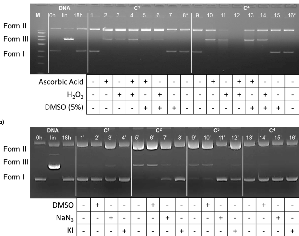
Figure 8. Cleavage of supercoiled \phi X174 DNA by Cu(II) complexes a) C 2 and C 3 and b) C 1 and C 4 in the presence of reducing (ascorbic acid, 10 \mu M), oxidizing agents (H 2 O 2 , 50 \mu M), hydroxyl radical scavenger (DMSO, 5 %) or in the dark (*), and c) C 1 - C 4 in the presence of hydroxyl radical scavenger (DMSO, 80 mM) and singlet oxygen species scavengers (NaN 3 and KI, 80 mM), after 18h of incubation at 37°C in phosphate buffer (pH 7.2), DNA lin - Linear DNA obtained by digestion with XhoI. Forms I, II and III are supercoiled, nicked circular and linear forms of DNA, respectively.
