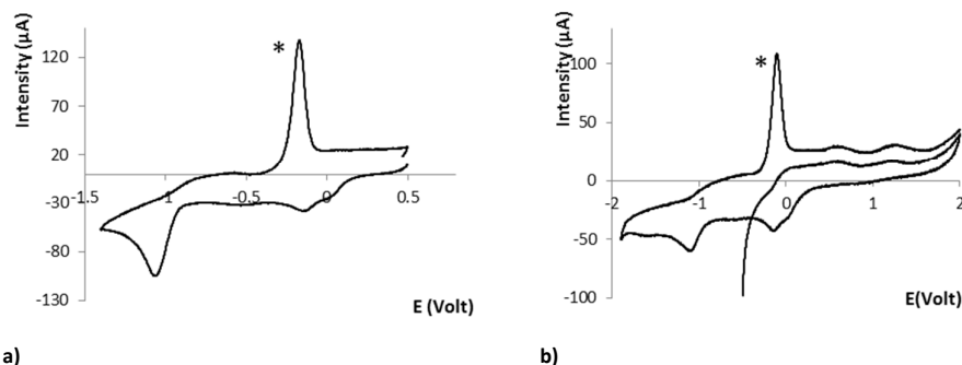
Figure 4. Representative cyclic voltammograms of a) C^2 and b) C^3 obtained in CH_3CN . (*) adsorption wave.
