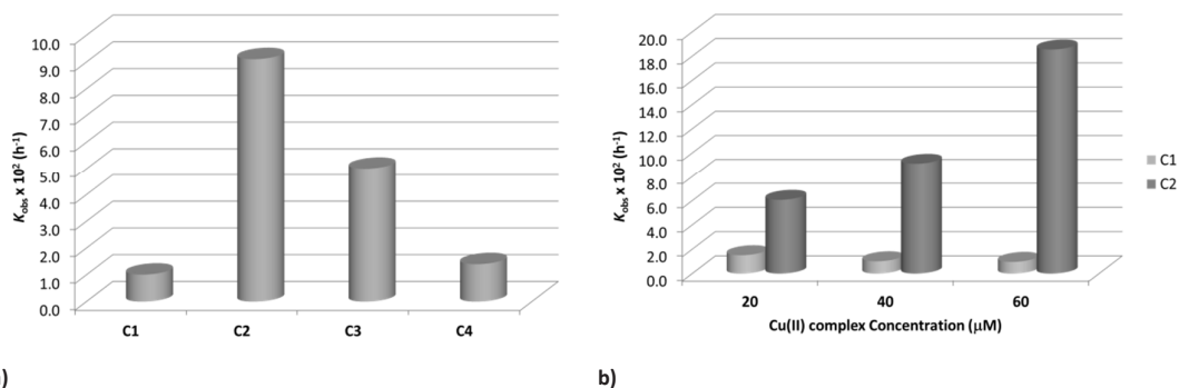
Figure 9. k_{\text{obs}} for the cleavage of supercoiled \phi X174 DNA by Cu(II) complexes a) \text{C}^1 - \text{C}^4 at 40 \mu\text{M} and b) \text{C}^1 and \text{C}^2 at indicated concentration, after incubation over time at 37°C, in phosphate buffer (pH 7.2).
