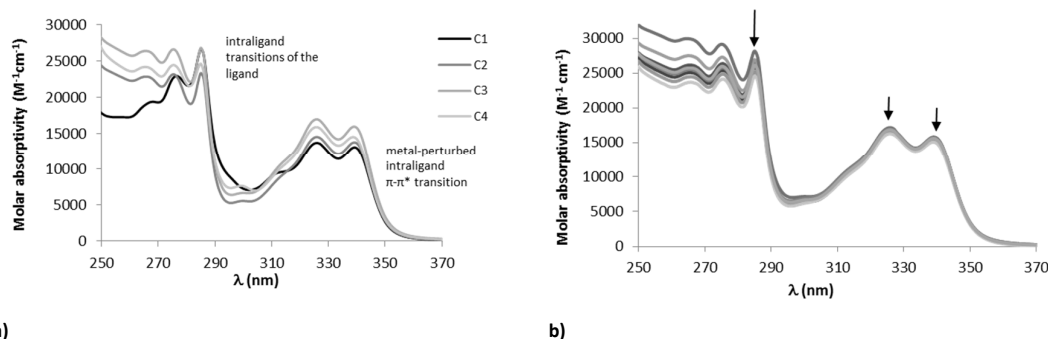
a) UV-Vis absorption spectra of a) Cu(II) complexes ( C^1 - C^4 ) and b) spectrophotometric titration of CT-DNA with complex C^3 (50 \mu M), in PBS buffer (10 mM, pH 7.2), at room temperature. The arrows indicate the changes of the bands upon addition of CT-DNA ( [DNA]/[C^3] = 0 - 3.2 ).
